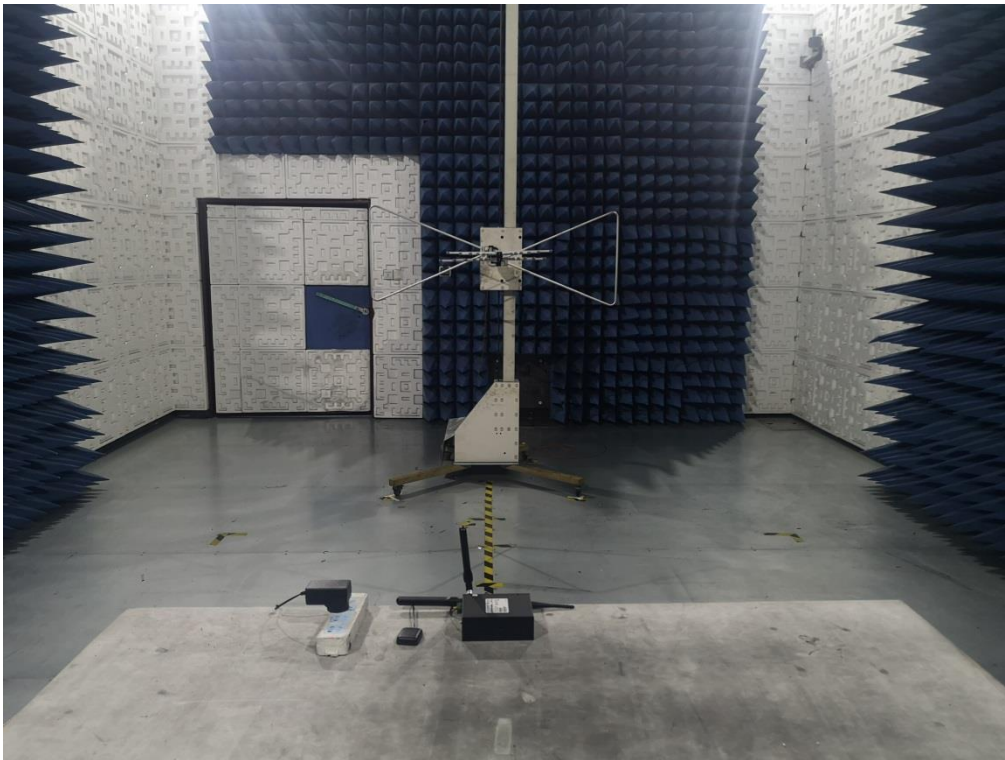
RADIATED SPURIOUS ABOVE 1G EMISSION- Glue Stick Antenna
