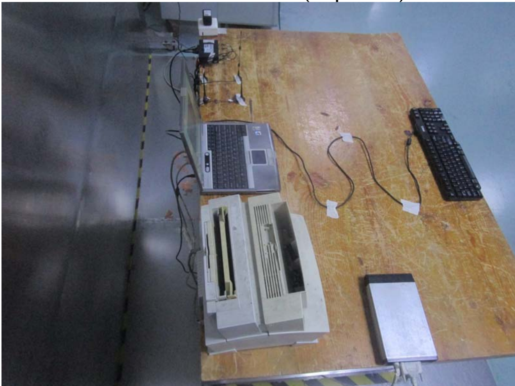
Conducted emissions side View(Adapter Mode)
