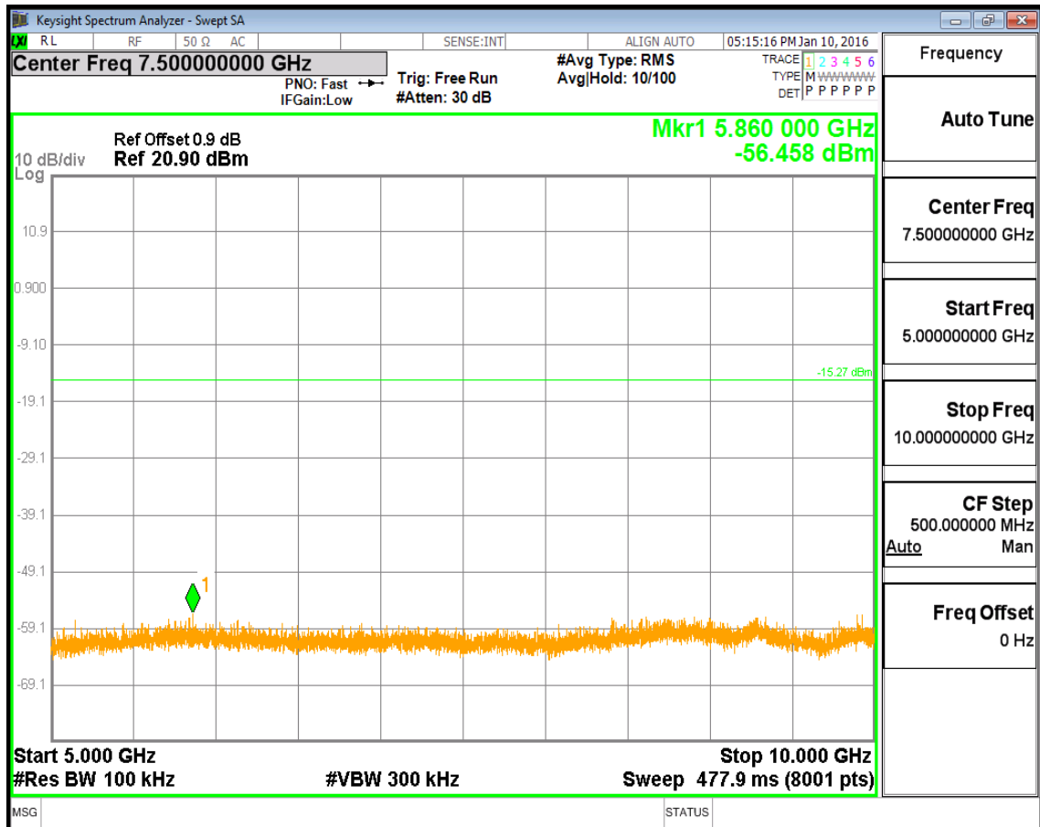
(Plot 4.9.2 A4: Channel 00: 2402MHz @ @ 8DPSK)
