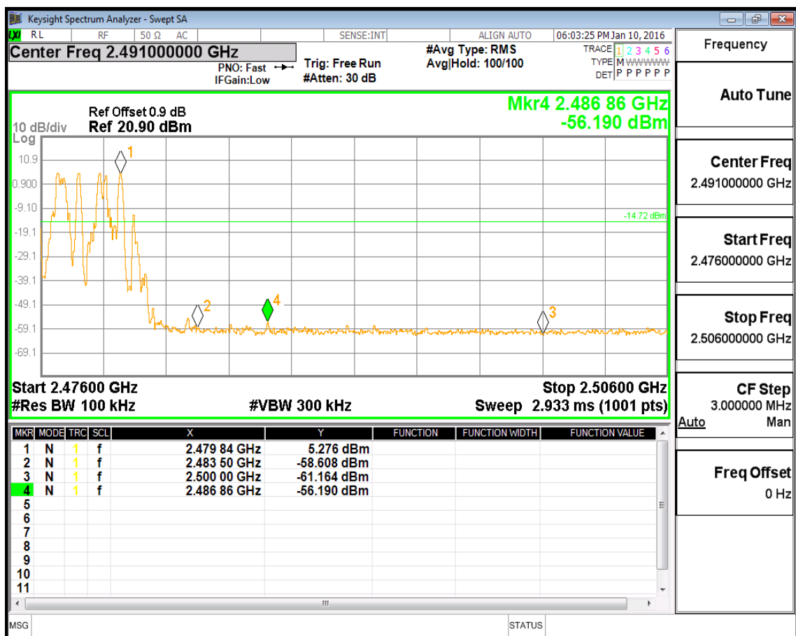
(Plot 4.9.1 D4: Right Band edge hopping on @ GFSK)
