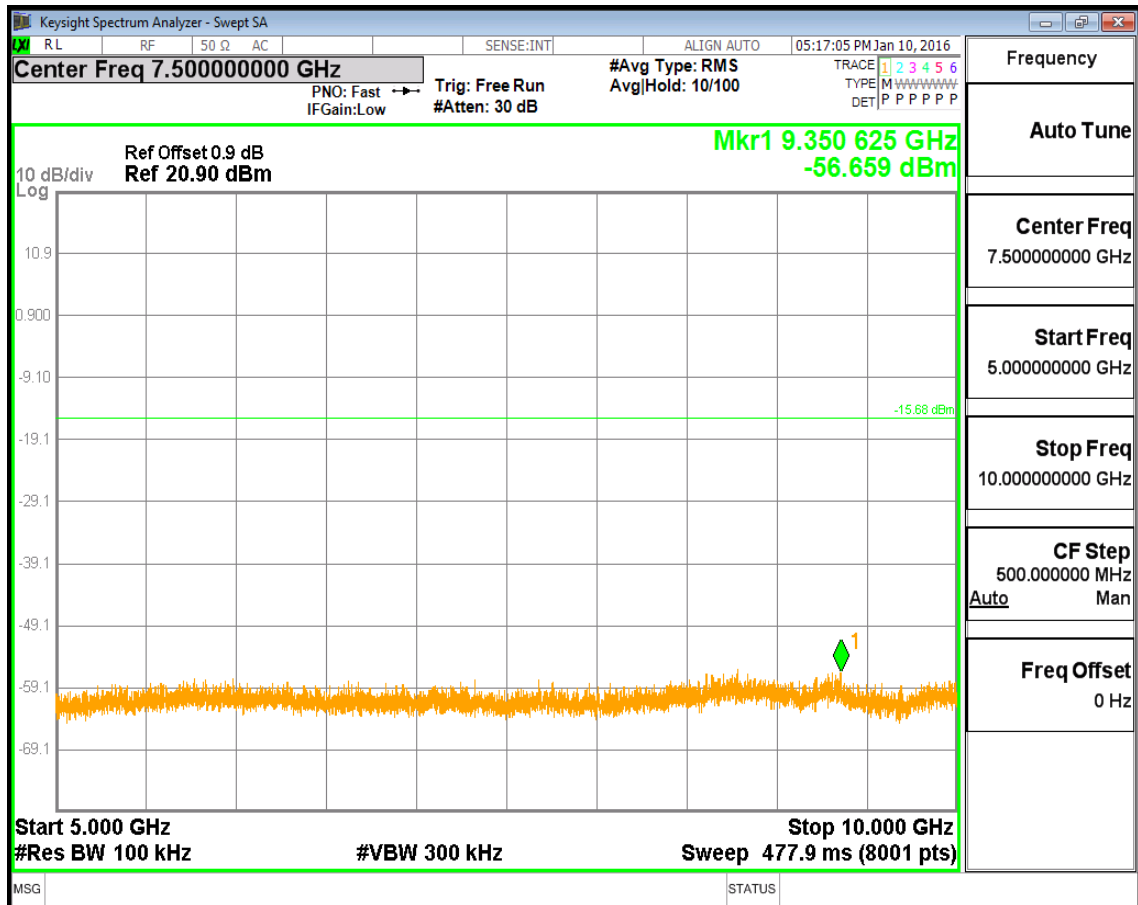
(Plot 4.9.2 B4: Channel 39: 2441MHz @ @ 8DPSK)
