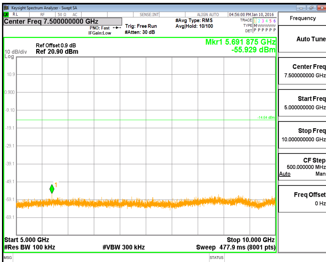
(Plot 4.9.1 B4: Channel 39: 2441MHz @ GFSK)
