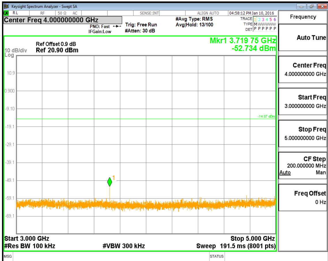
(Plot 4.9.1 C3: Channel 78: 2480MHz @ GFSK)
