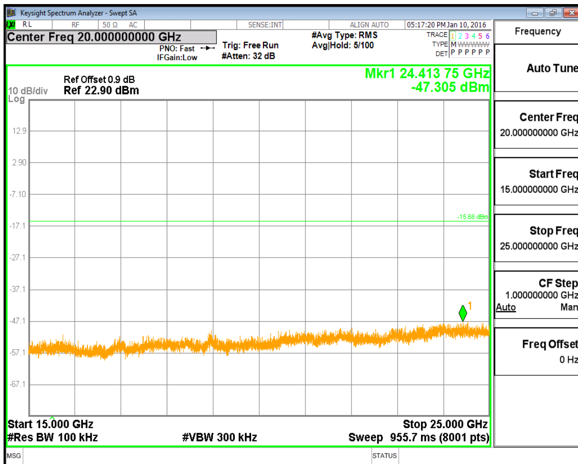
(Plot 4.9.2 B6: Channel 39: 2441MHz @ @ 8DPSK)
