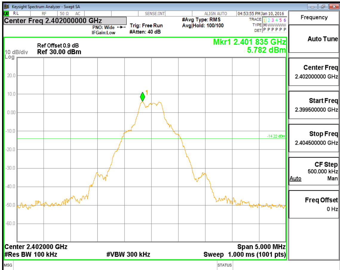
(Plot 4.9.1 A1: Channel 00: 2402MHz @ GFSK)
