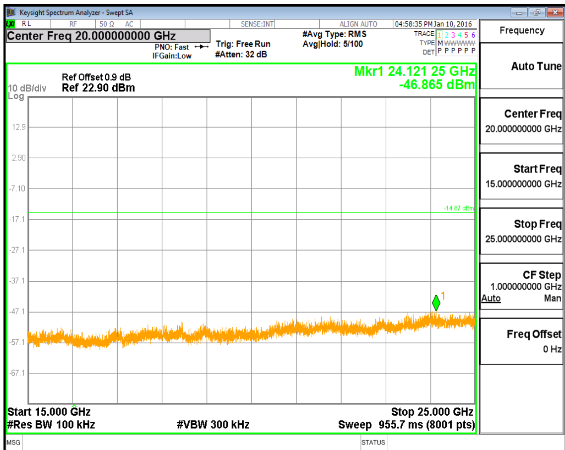
(Plot 4.9.1 C6: Channel 78: 2480MHz @ GFSK)
