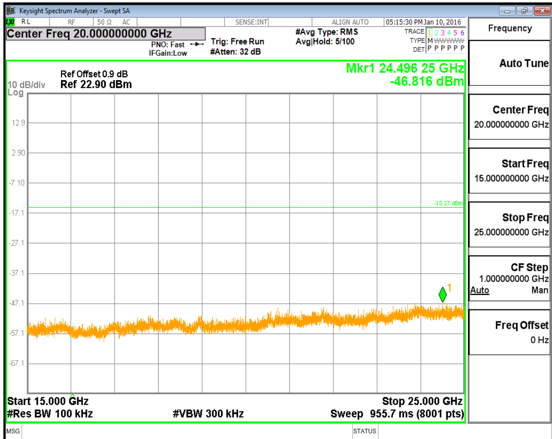
(Plot 4.9.2 A6: Channel 00: 2402MHz @ @ 8DPSK)
