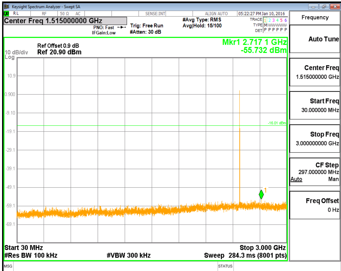
(Plot 4.9.2 C2: Channel 78: 2480MHz @ @ 8DPSK)
