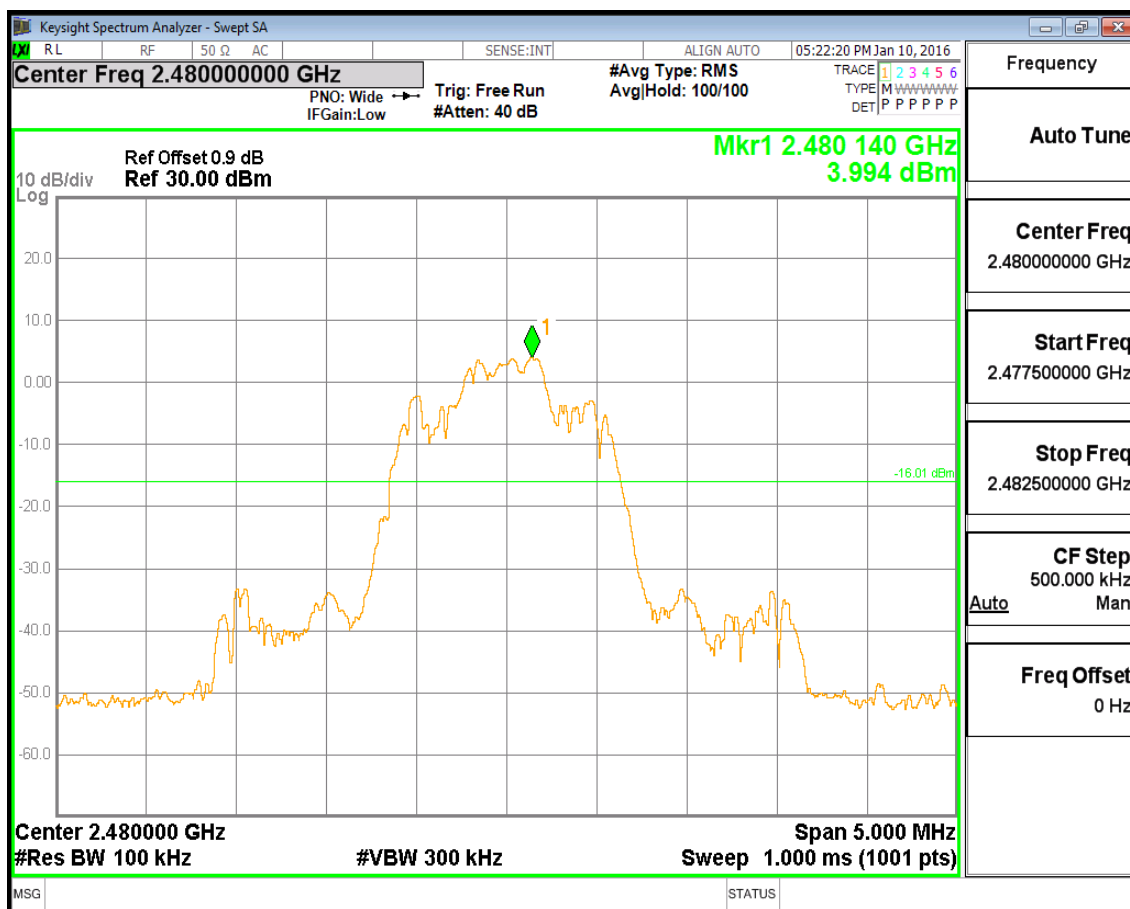
(Plot 4.9.2 C1: Channel 78: 2480MHz @ @ 8DPSK)
