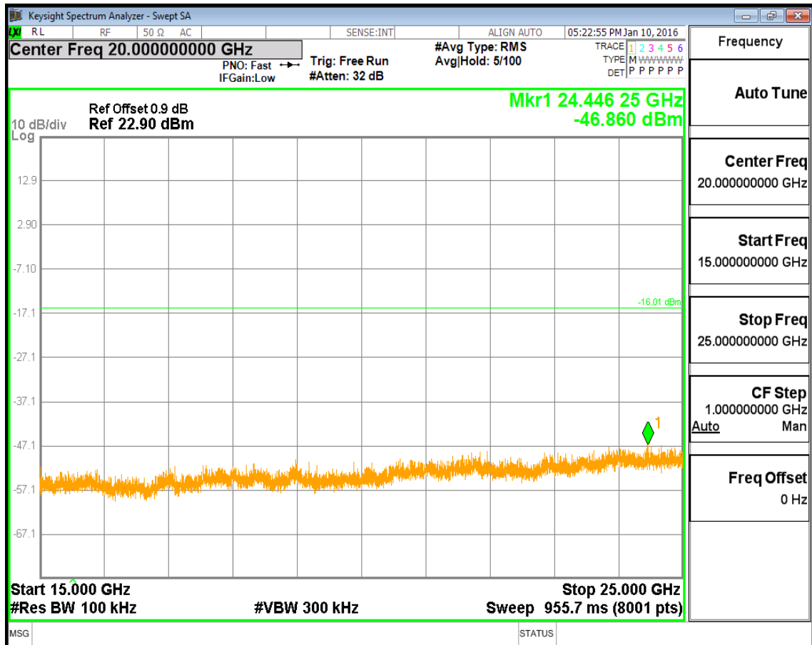
(Plot 4.9.2 C6: Channel 78: 2480MHz @ @ 8DPSK)
