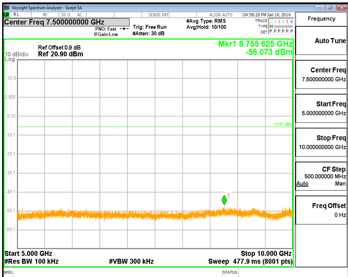
(Plot 4.9.1 C4: Channel 78: 2480MHz @ GFSK)
