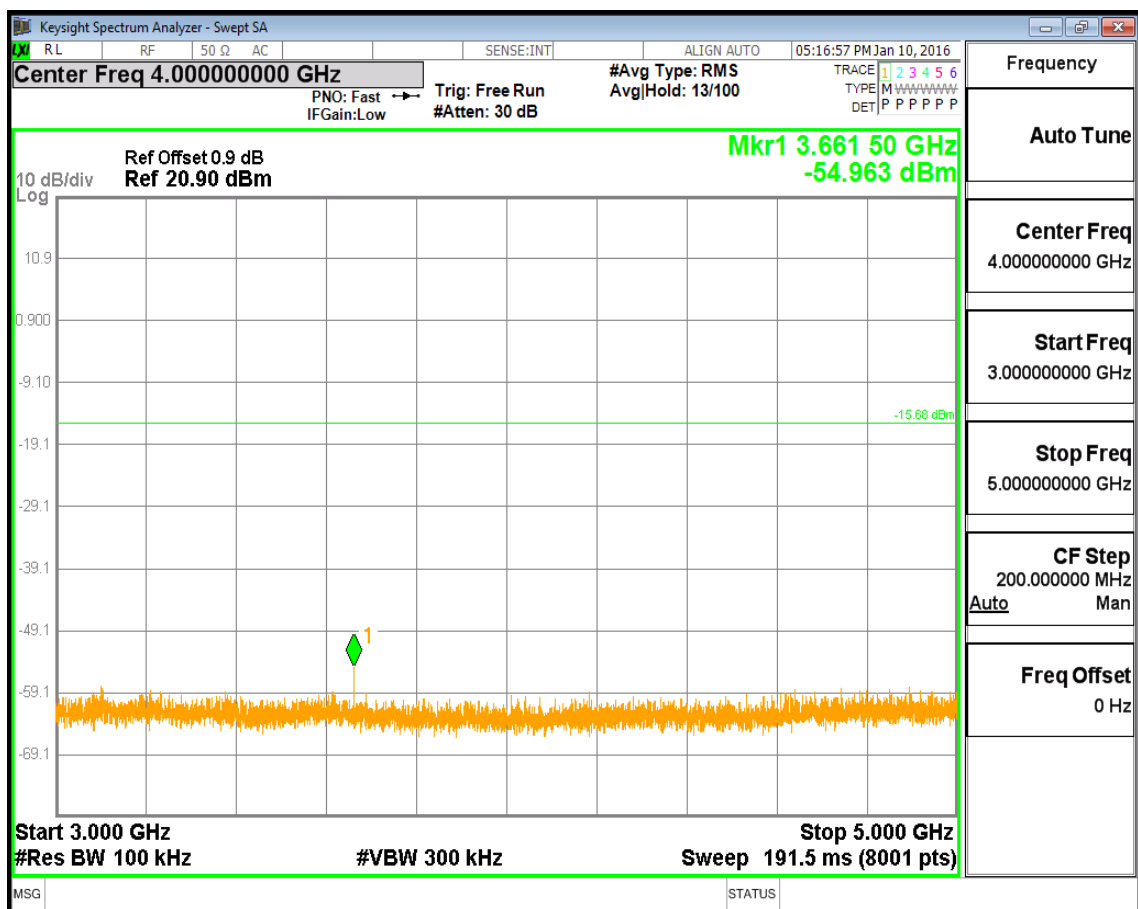
(Plot 4.9.2 B3: Channel 39: 2441MHz @ @ 8DPSK)
