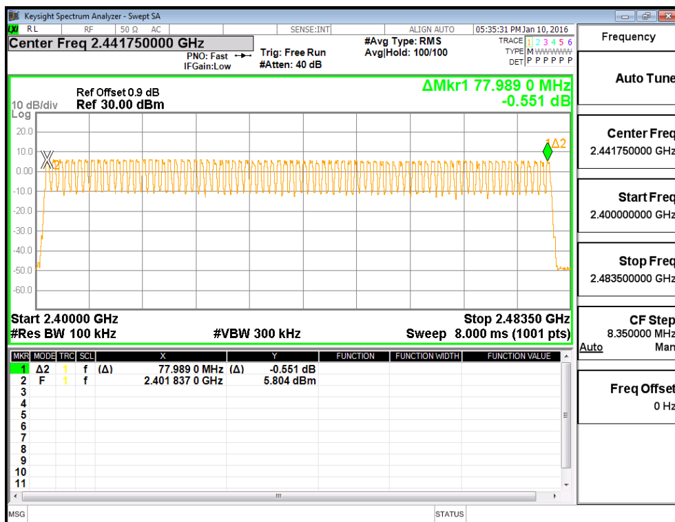
(Plot 4.7.1 A1: @ GFSK)
