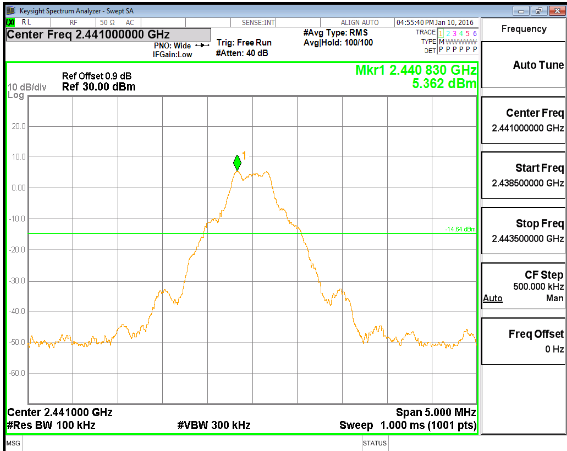
(Plot 4.9.1 B1: Channel 39: 2441MHz @ GFSK)
