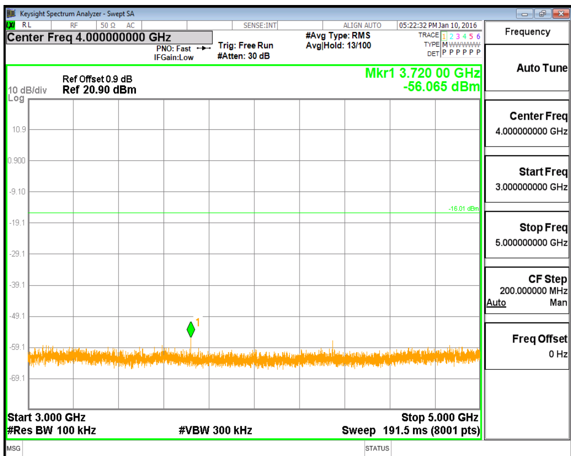
(Plot 4.9.2 C3: Channel 78: 2480MHz @ @ 8DPSK)
