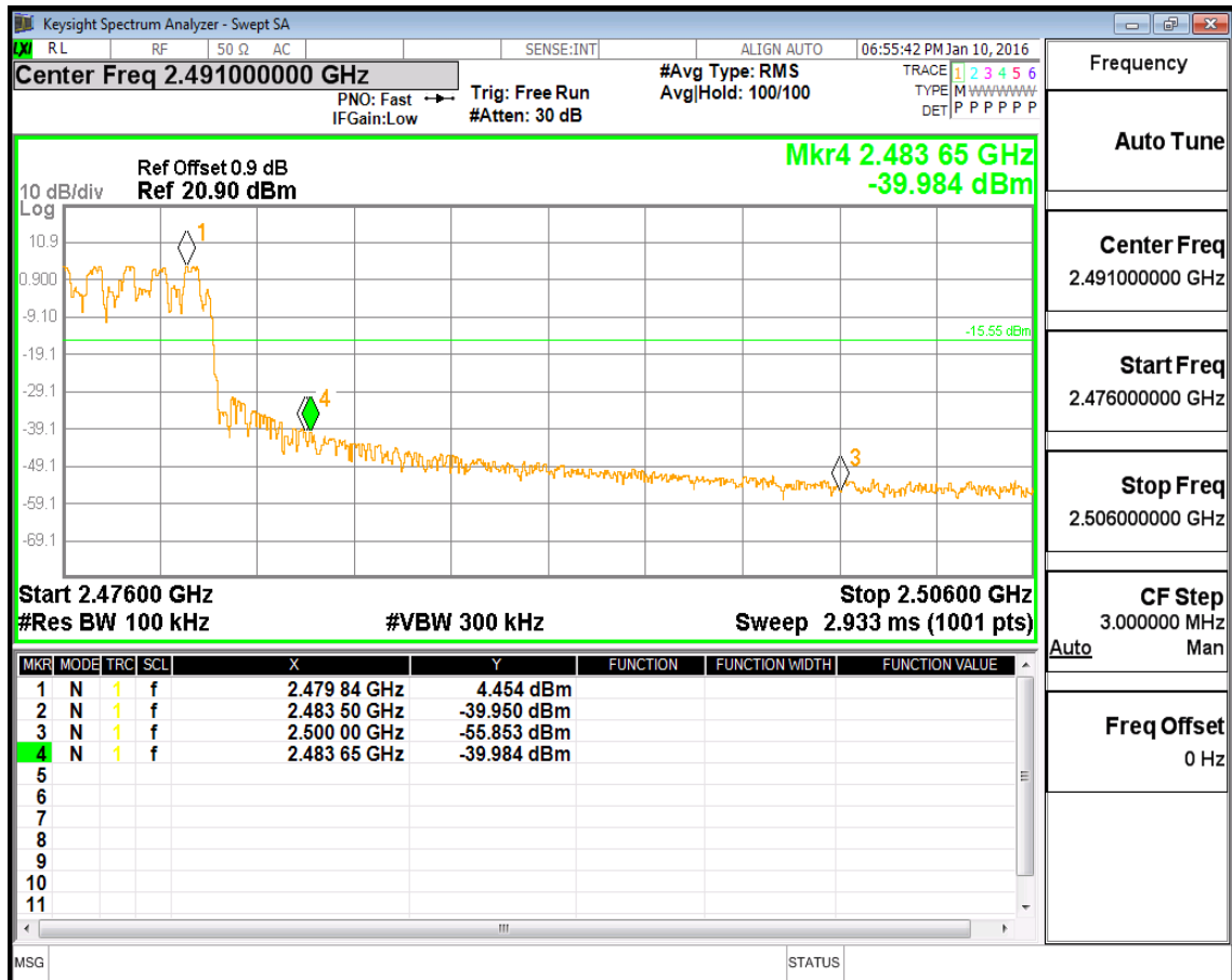
(Plot 4.9.2 D4: Right Band edge hopping on @ 8DPSK)
