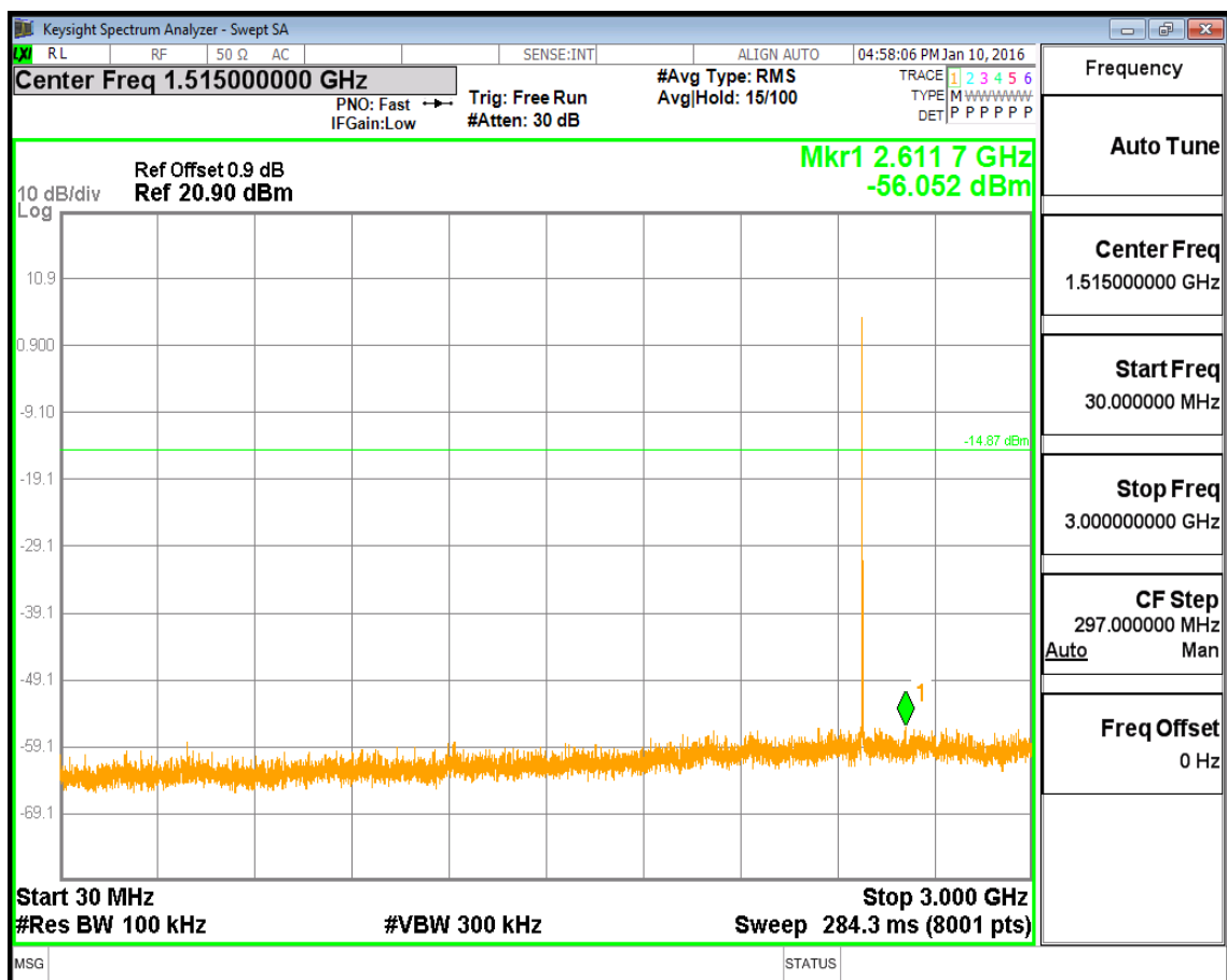
(Plot 4.9.1 C2: Channel 78: 2480MHz @ GFSK)
