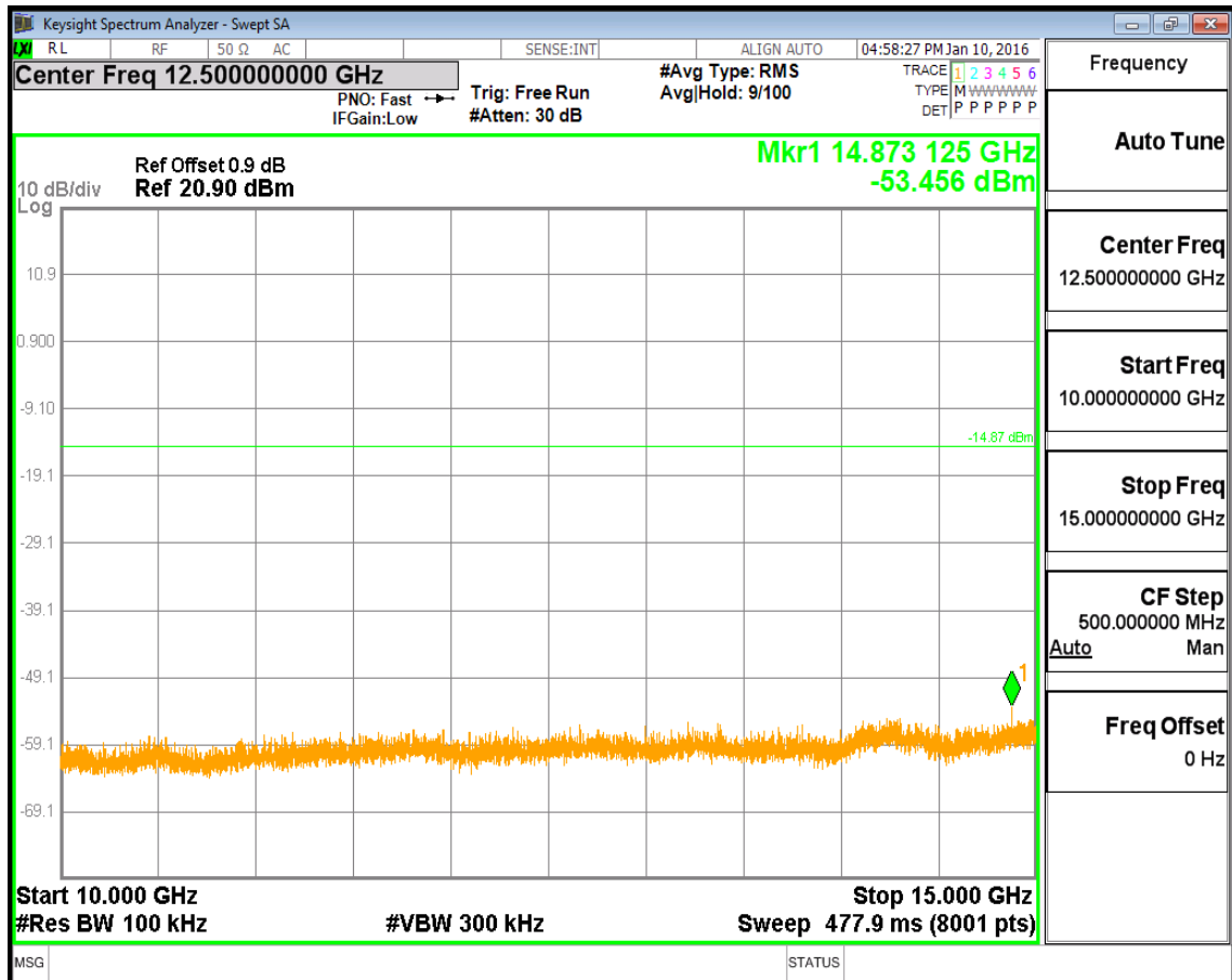
(Plot 4.9.1 C5: Channel 78: 2480MHz @ GFSK)
