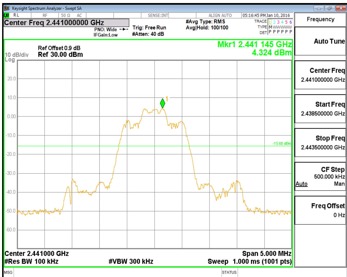
(Plot 4.9.2 B1: Channel 39: 2441MHz @ @ 8DPSK)
