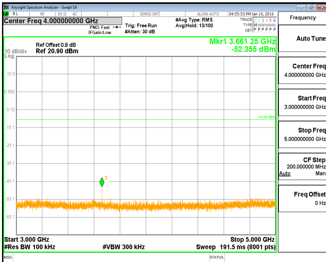
(Plot 4.9.1 B3: Channel 39: 2441MHz @ GFSK)
