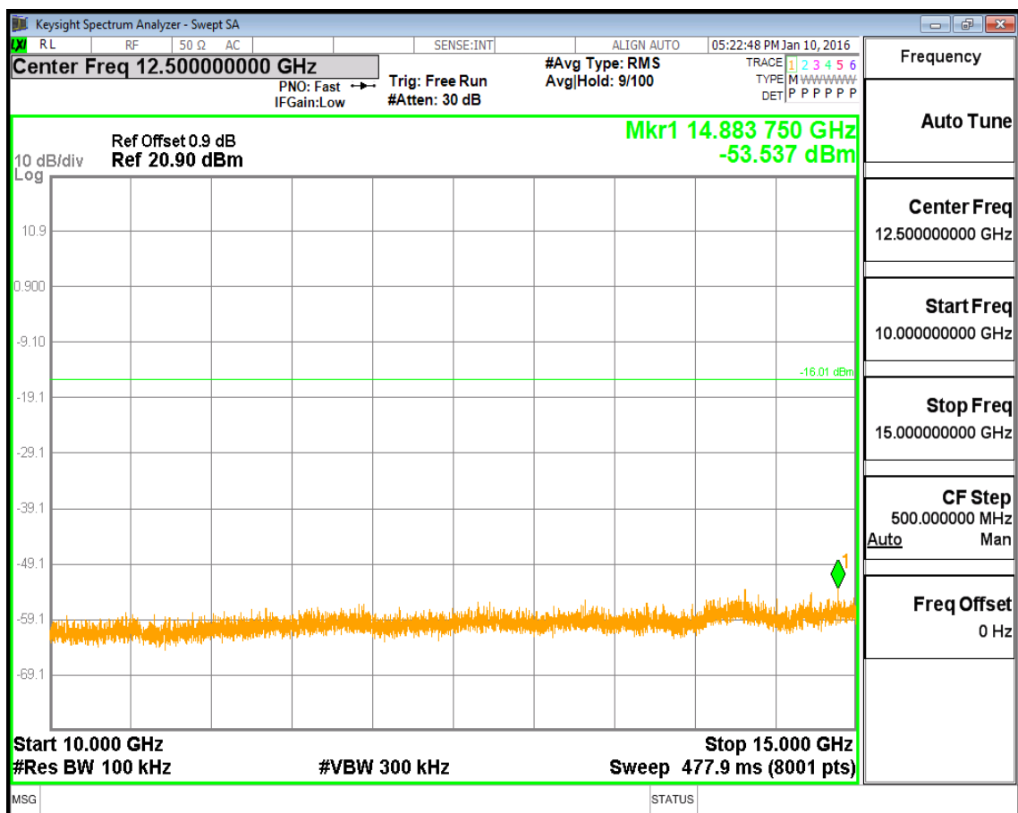
(Plot 4.9.2 C5: Channel 78: 2480MHz @ @ 8DPSK)
