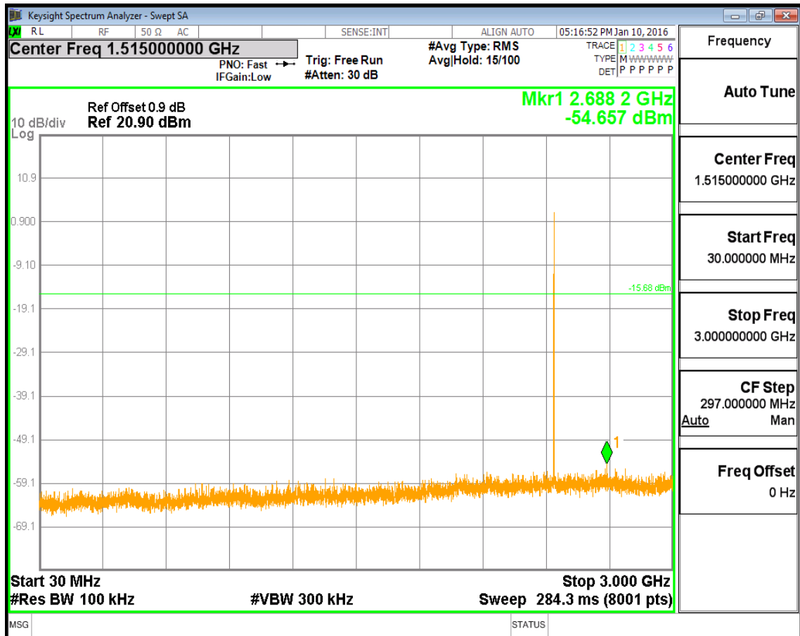
(Plot 4.9.2 B2: Channel 39: 2441MHz @ @ 8DPSK)
