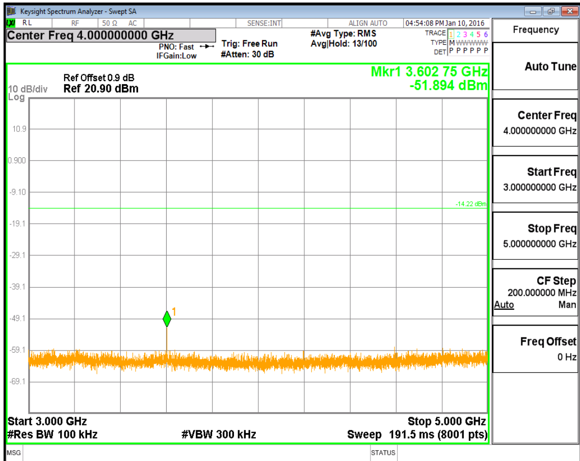
(Plot 4.9.1 A3: Channel 00: 2402MHz @ GFSK)
