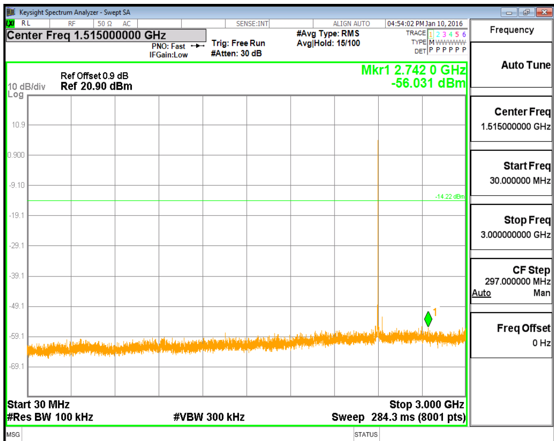
(Plot 4.9.1 A2: Channel 00: 2402MHz @ GFSK)
