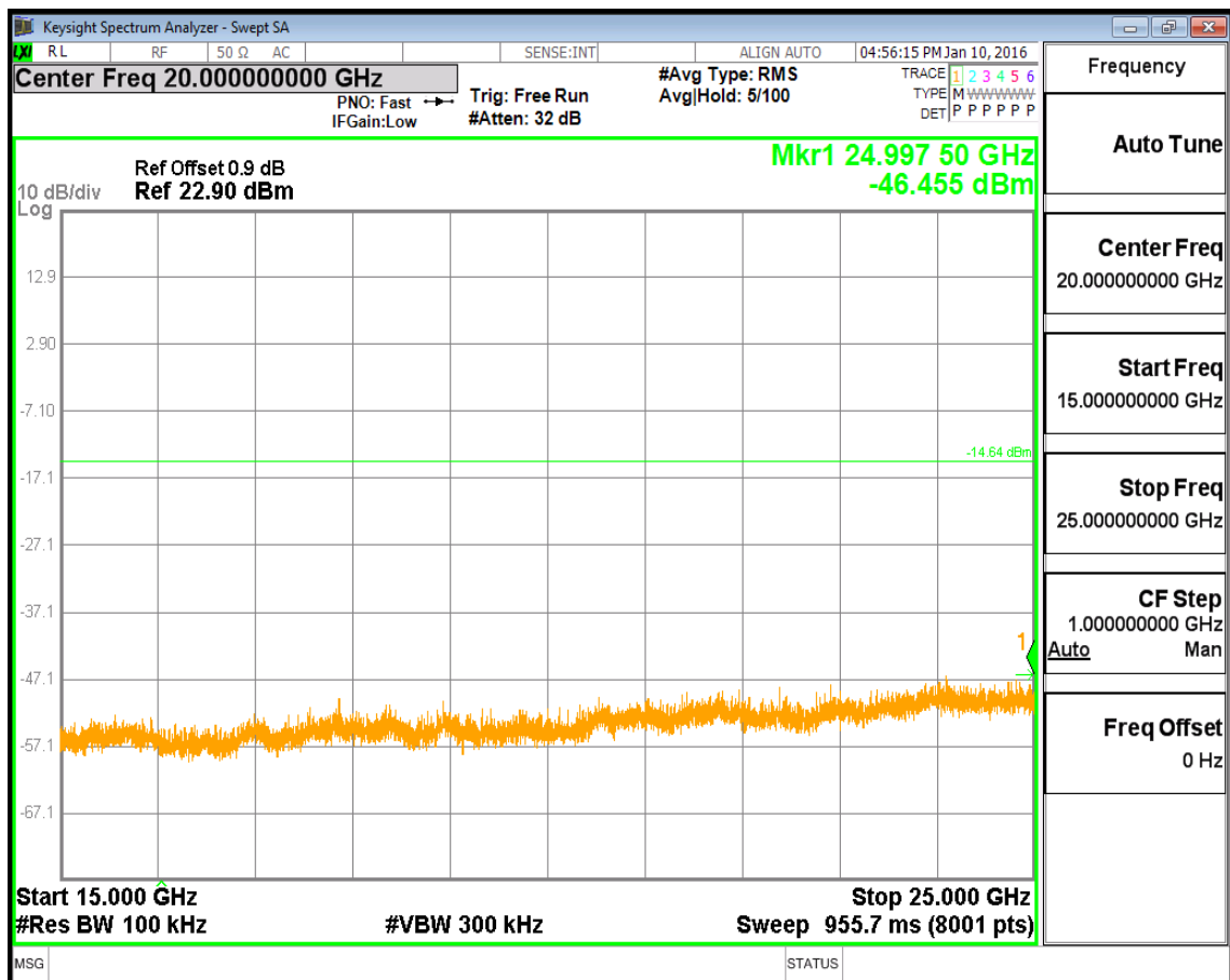
(Plot 4.9.1 B6: Channel 39: 2441MHz @ GFSK)
