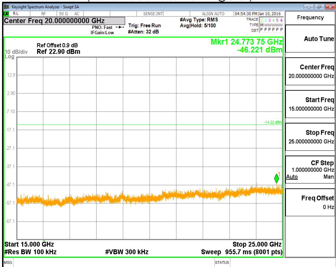
(Plot 4.9.1 A6: Channel 00: 2402MHz @ GFSK)
