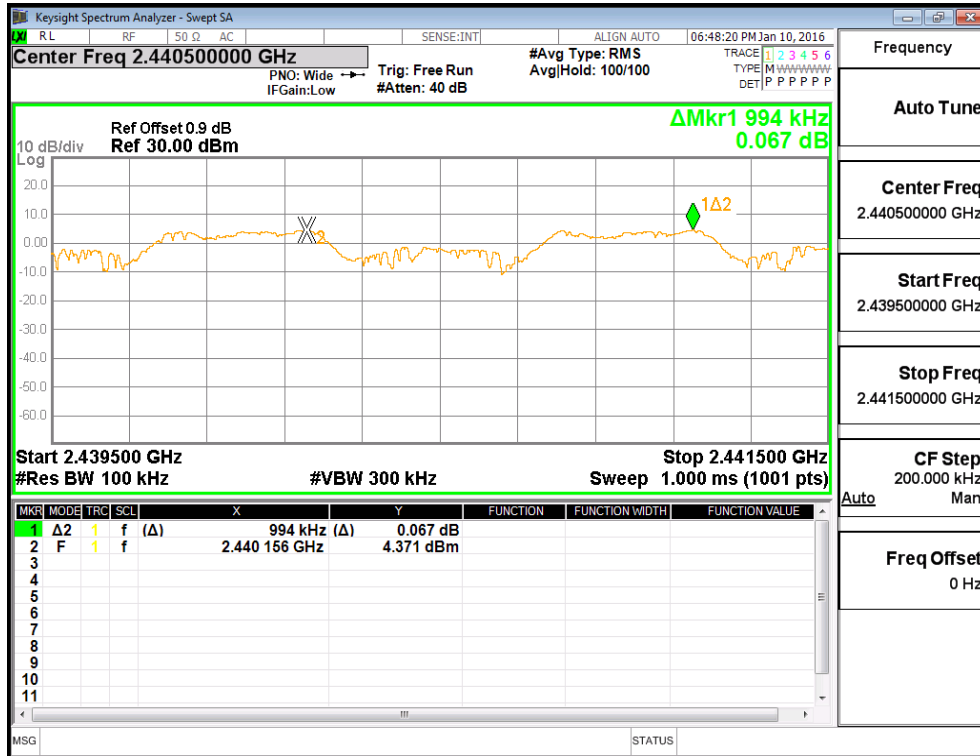
(Plot 4.6.2 A: Channel 39: 2441MHz @ 8DPSK)
