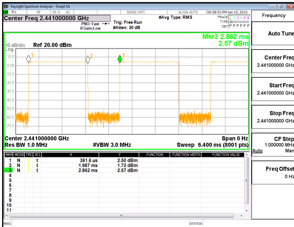
(Plot 4.8.1.B: Channel 39: 2441MHz @ GFSK @ DH3)
