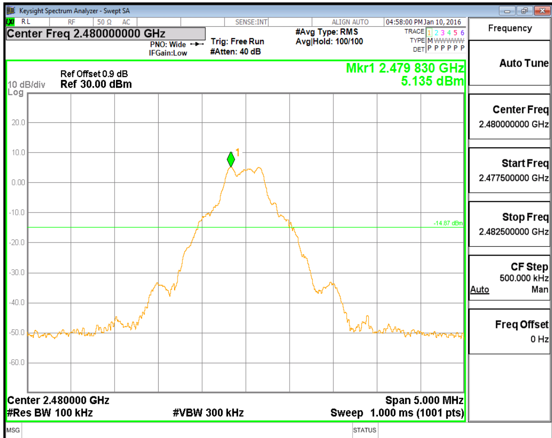
(Plot 4.9.1 C1: Channel 78: 2480MHz @ GFSK)
