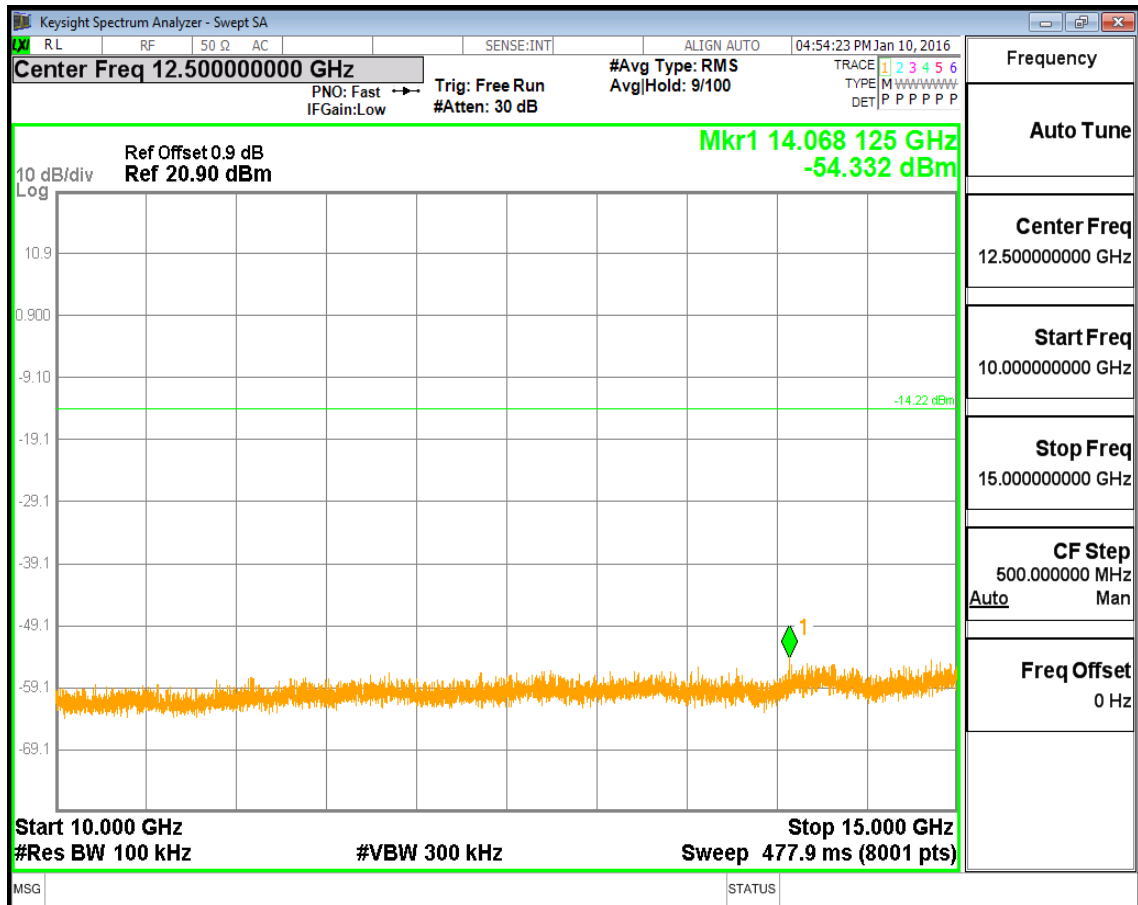
(Plot 4.9.1 A5: Channel 00: 2402MHz @ GFSK)
