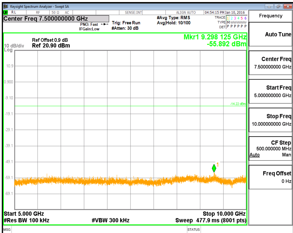
(Plot 4.9.1 A4: Channel 00: 2402MHz @ GFSK)
