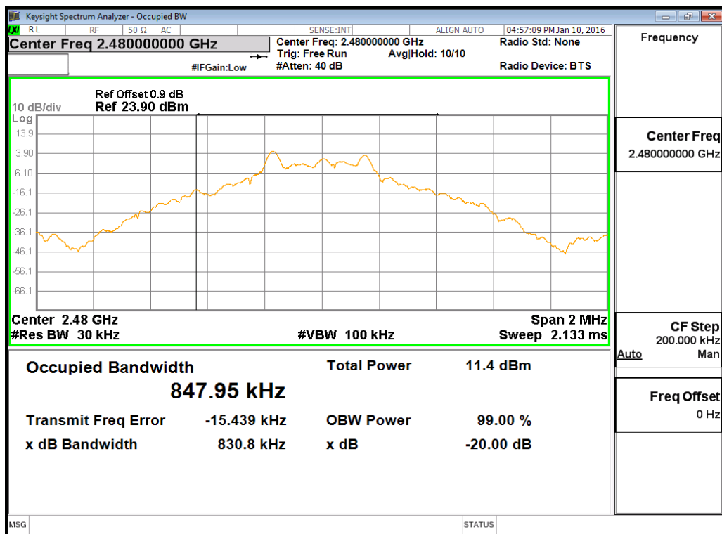
(Plot 4.4.1 C: Channel 78: 2480MHz @ GFSK)
