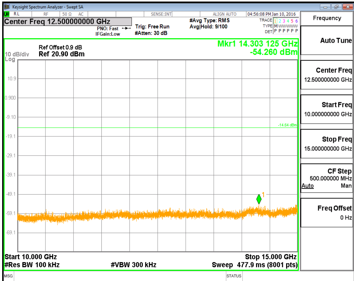
(Plot 4.9.1 B5: Channel 39: 2441MHz @ GFSK)
