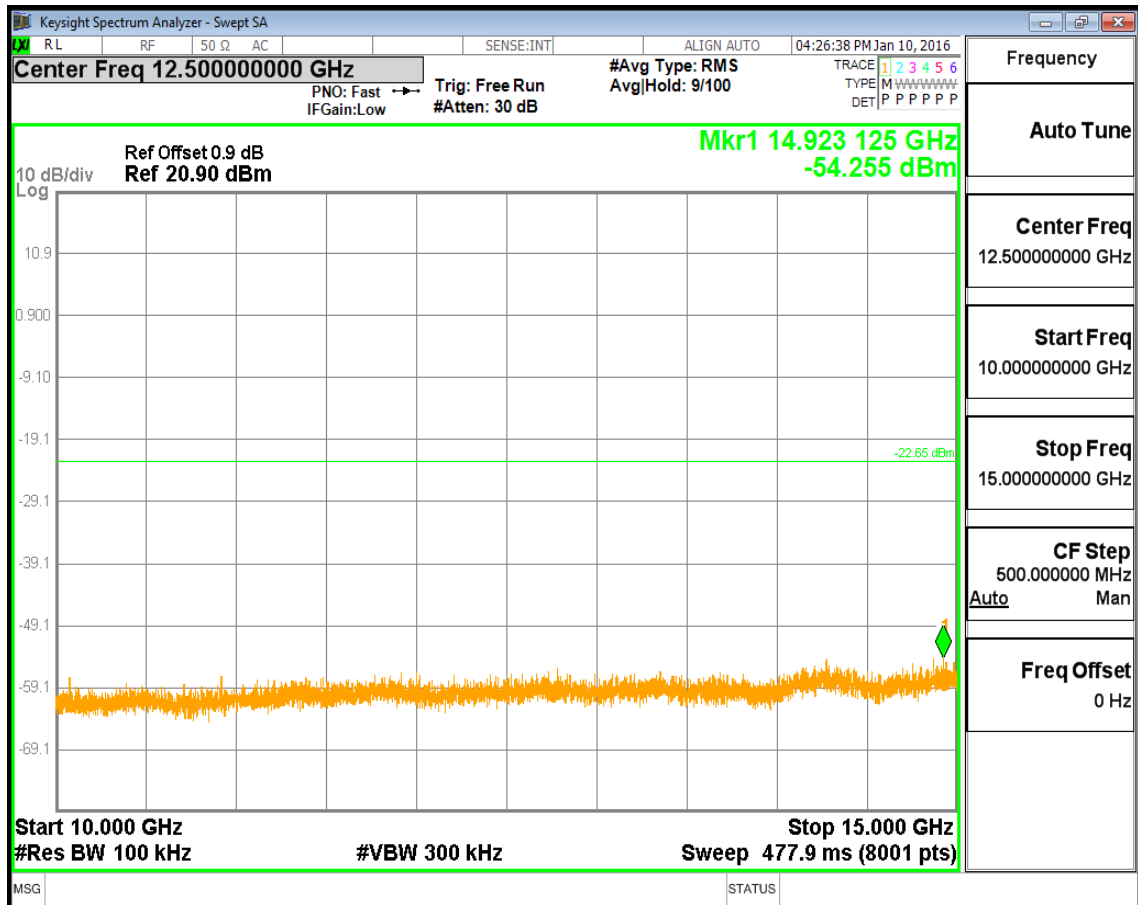
(Plot 4.5.1 A5: Channel 00: 2402MHz @ GFSK)
