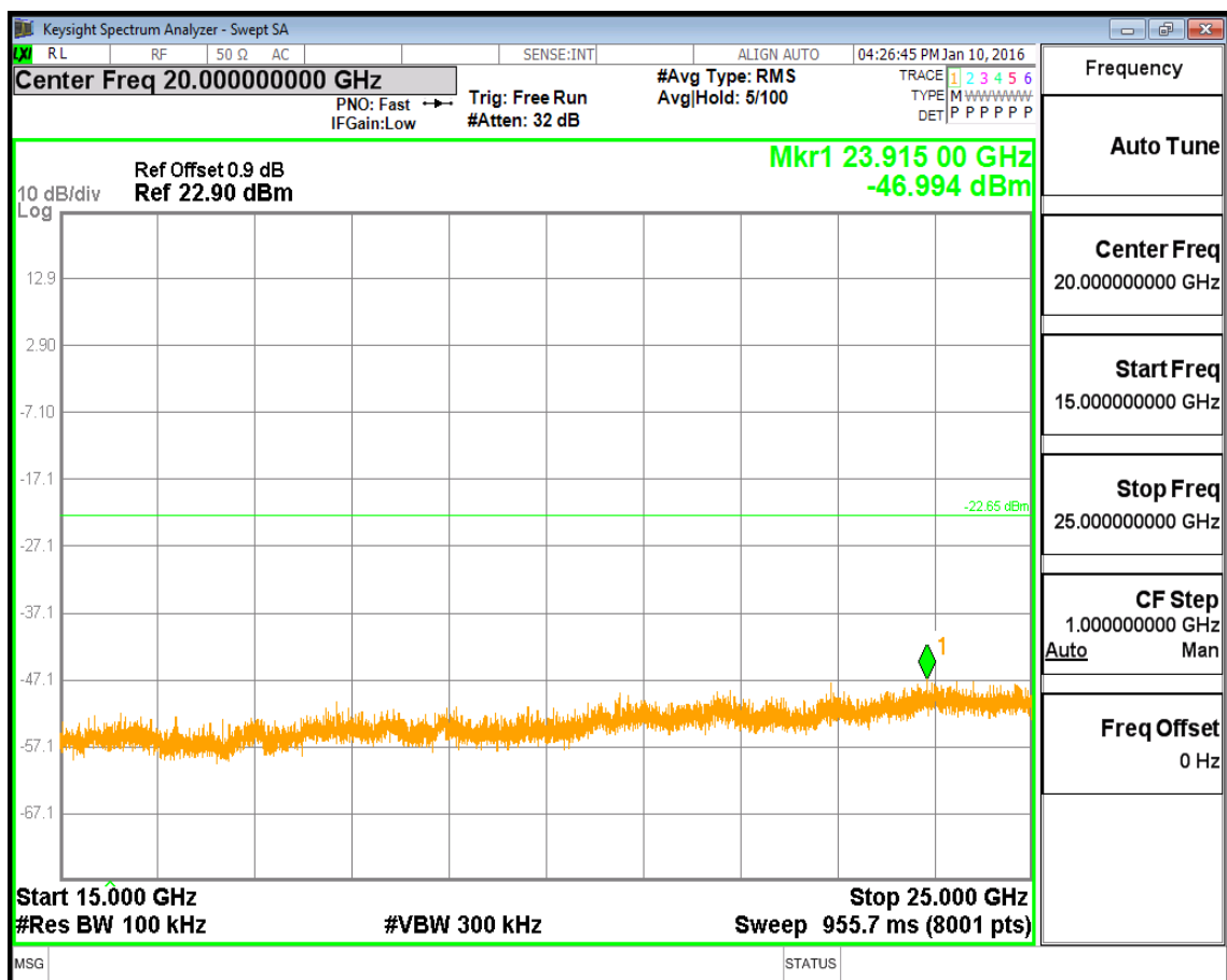
(Plot 4.5.1 A6: Channel 00: 2402MHz @ GFSK)
