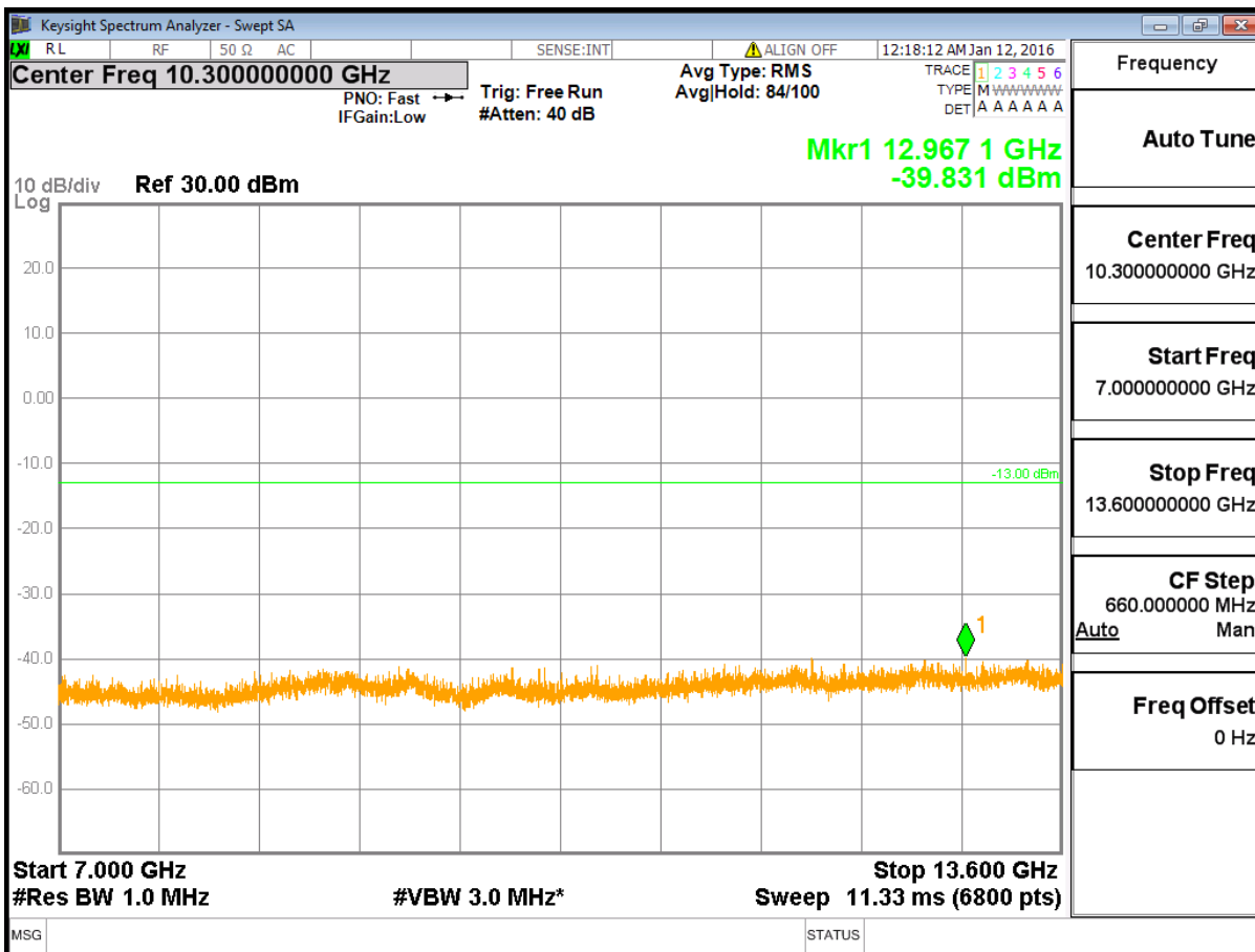
4.5.2 A5: Channel 512: 1850.20MHz @ Traffic @ PCS1900
