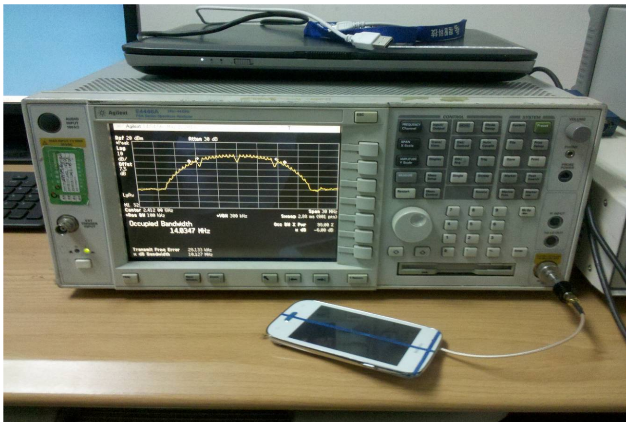
CONNECTED TO THE SPECTRUM ANALYZER
