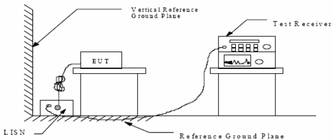
Shielding Room Test Setup Diagram
