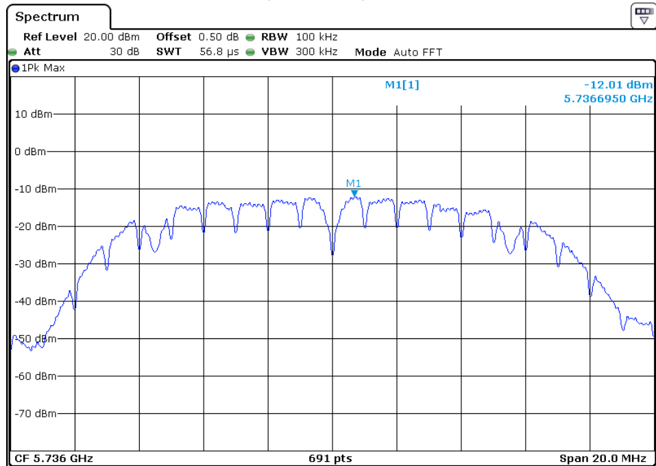
Low channel(Antenna B)
