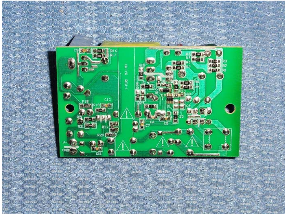
(Alternative Switch Power supply board)
