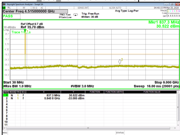
GSM_850_Middle_Conducted_Spurious
