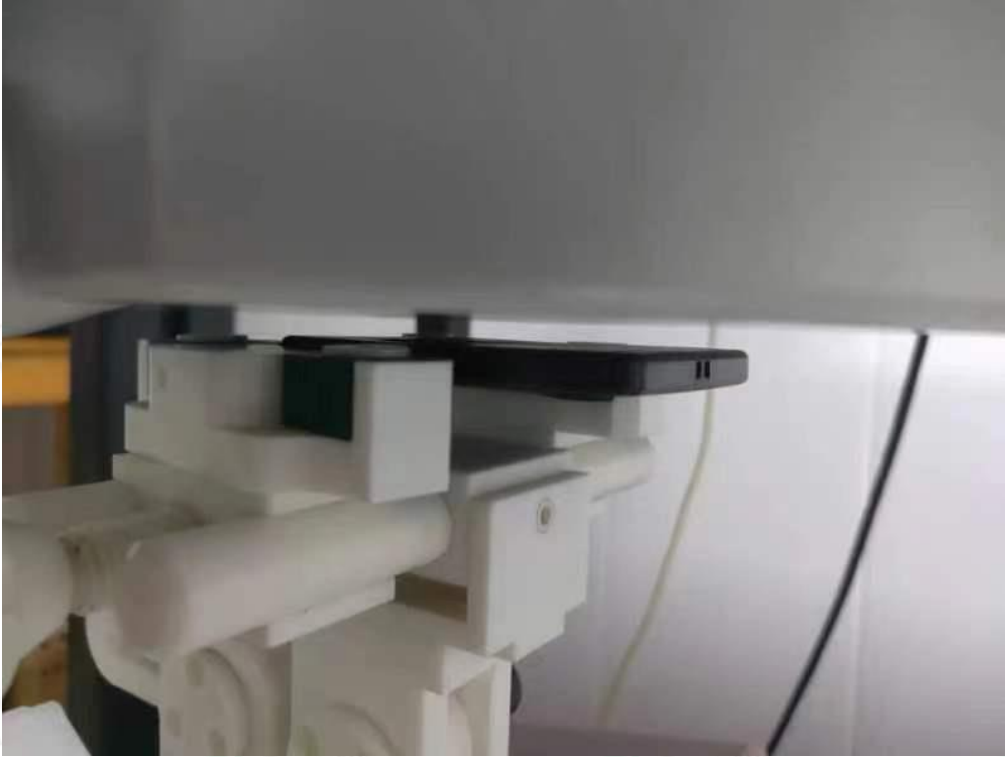
5mm body Vertical-Back Side Setup Photo
