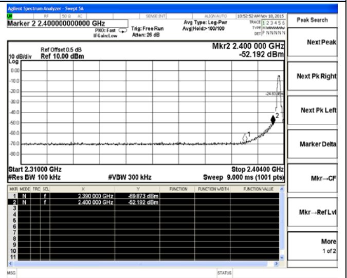
Channel 0 / 2402 MHz
