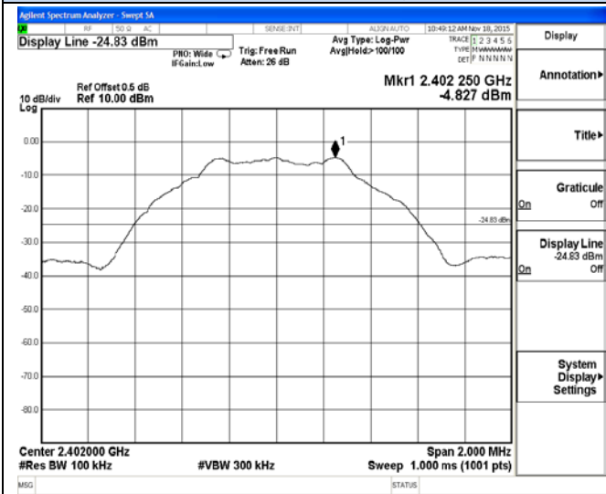
2401 – 2403 MHz
