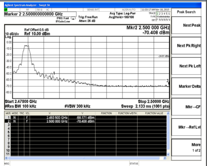
Channel 39 / 2480 MHz
