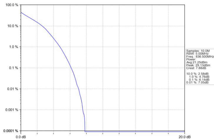
Band26b 3MHz QPSK MCH 836.5MHz RB 15 0 NTNV
