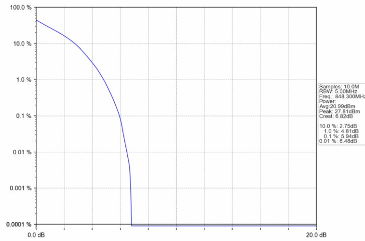
Band26b_1.4MHz_QPSK_HCH_848.3MHz_RB_6_0_NTNV
