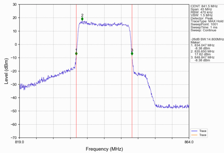
Band26b_15MHz_16QAM_HCH_841.5MHz_RB_75_0_NTNV
