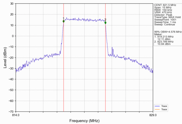
Band26a_5MHz_16QAM_HCH_821.5MHz_RB_25_0_NTNV
