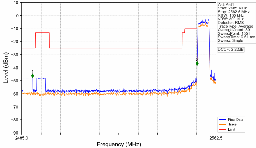
Band41_5MHz_16QAM_LCH_2557.5MHz_RB_25_0_NTNV
