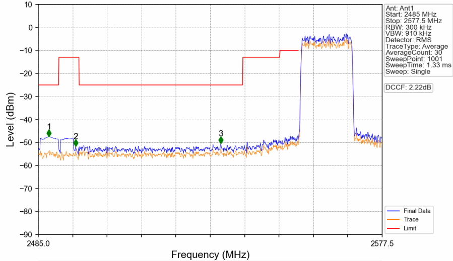
Band41_15MHz_16QAM_LCH_2562.5MHz_RB_75_0_NTNV
