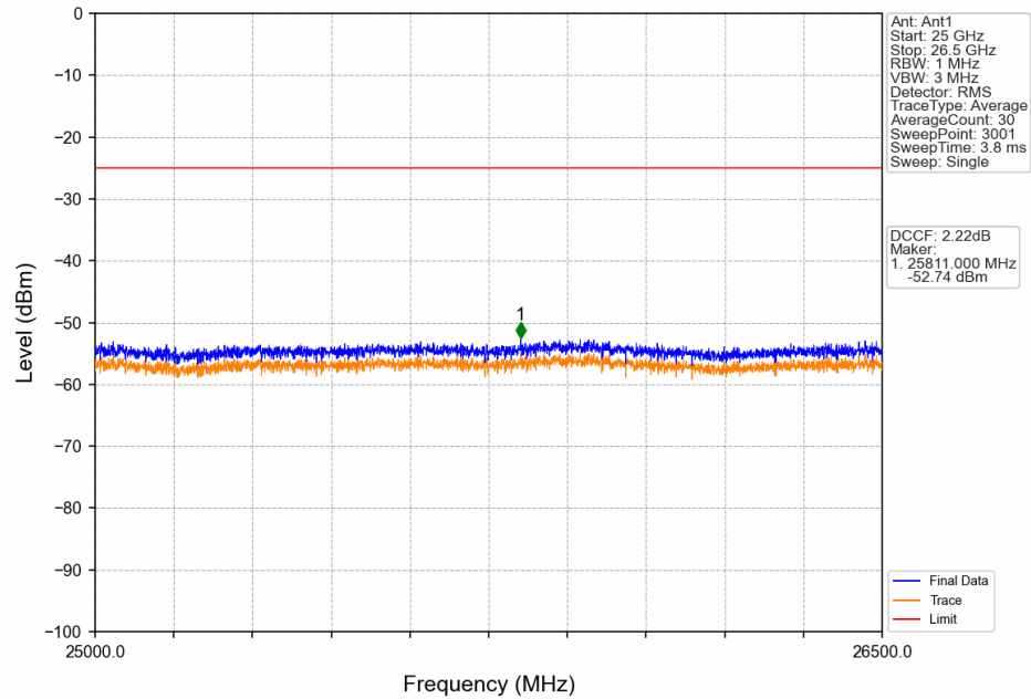
Band41_15MHz_16QAM_HCH_2647.5MHz_RB_1_0_NTNV
