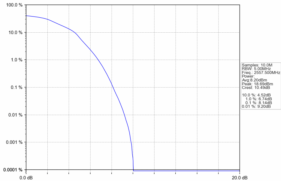
Band41_5MHz_16QAM_LCH_2557.5MHz_RB_25_0_NTNV
