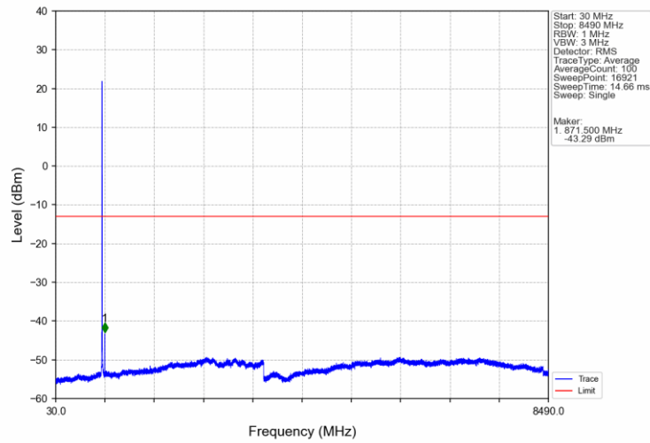
Band26b_3MHz_QPSK_LCH_825.5MHz_RB_1_0_NTNV
