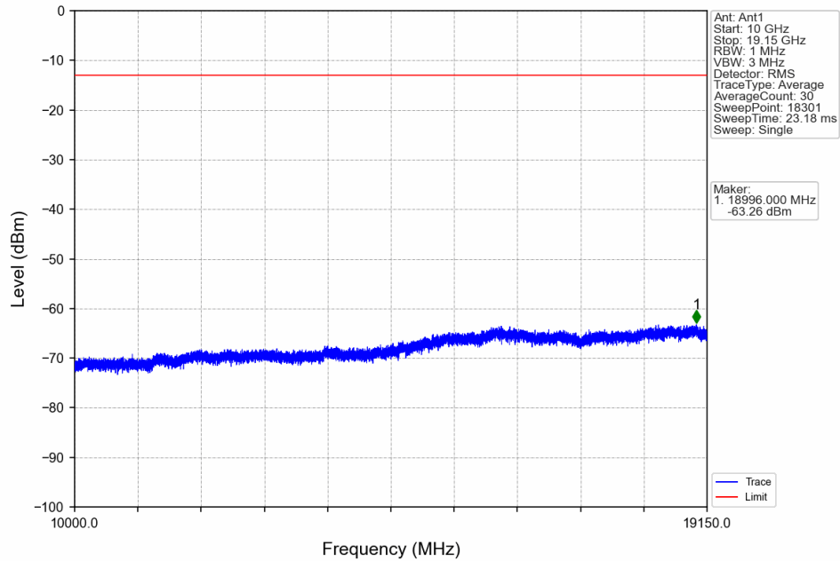
Band25_15MHz_QPSK_MCH_1882.5MHz_RB_1_0_NTNV
