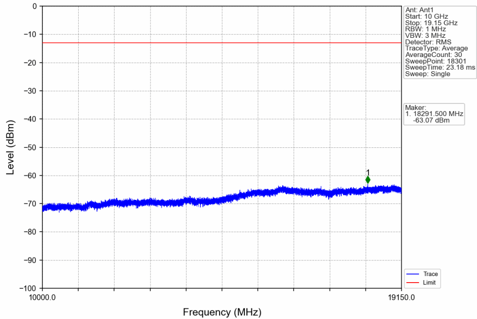
Band25_20MHz_16QAM_HCH_1905MHz_RB_1_0_NTNV
