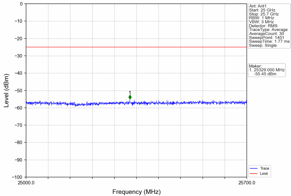
Band7_15MHz_16QAM_HCH_2562.5MHz_RB_1_0_NTNV
