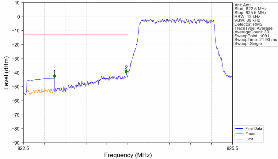
Band5_1.4MHz_16QAM_LCH_824.7MHz_RB_6_0_NTNV
