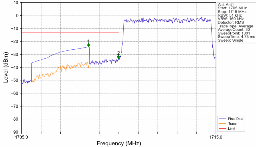
Band4_5MHz_16QAM_LCH_1712.5MHz_RB_25_0_NTNV
