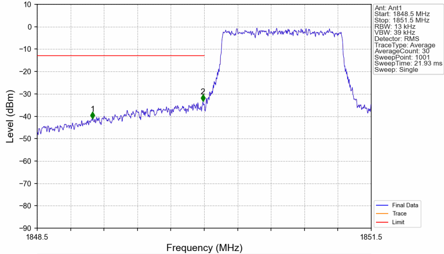
Band2_1.4MHz_QPSK_LCH_1850.7MHz_RB_6_0_NTNV
