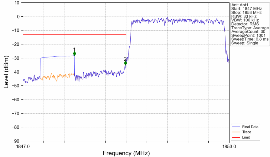
Band2_3MHz_QPSK_LCH_1851.5MHz_RB_15_0_NTNV
