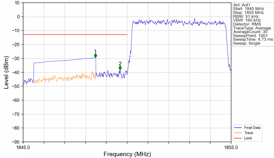
Band2_5MHz_16QAM_LCH_1852.5MHz_RB_25_0_NTNV
