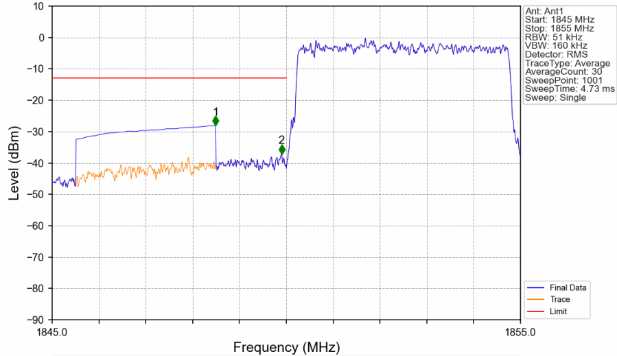
Band2_5MHz_QPSK_LCH_1852.5MHz_RB_25_0_NTNV
