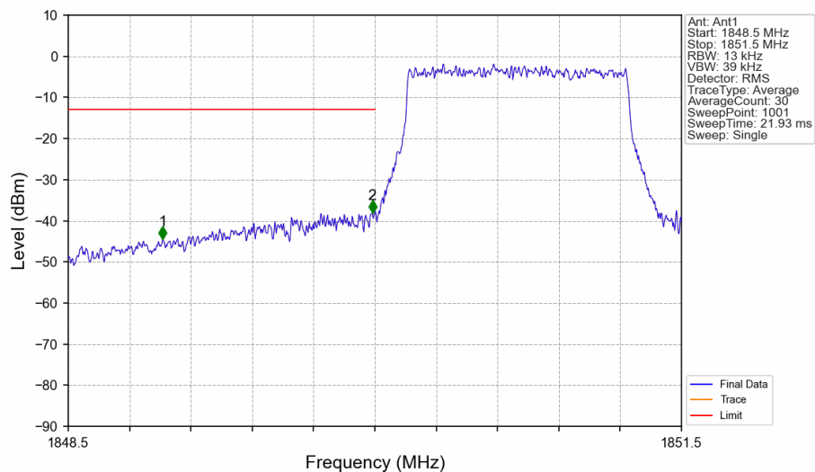
Band2_1.4MHz_16QAM_LCH_1850.7MHz_RB_6_0_NTNV
