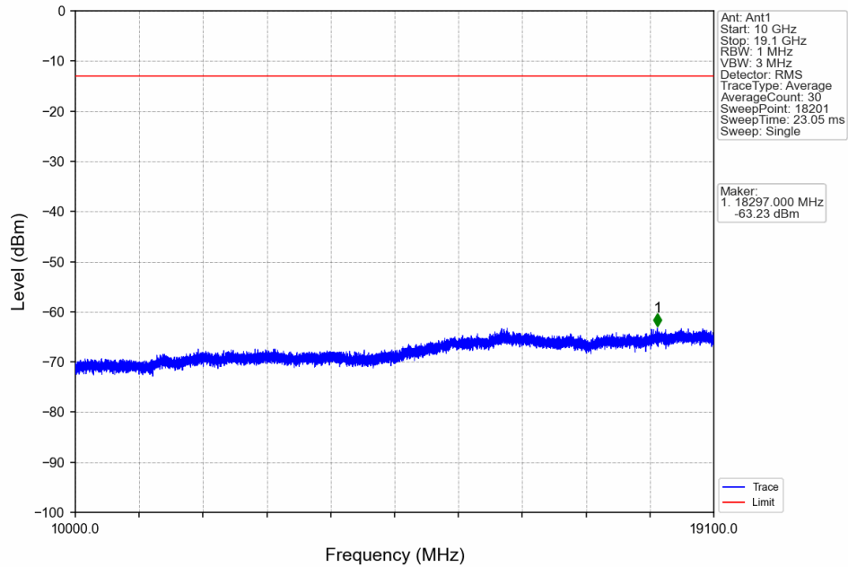
Band2_3MHz_16QAM_HCH_1908.5MHz_RB_1_0_NTNV
