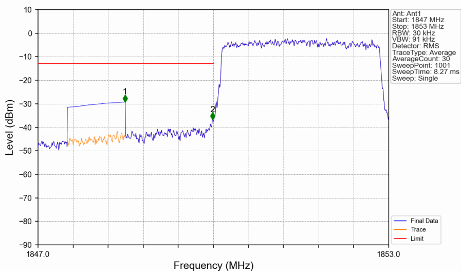
Band2_3MHz_16QAM_LCH_1851.5MHz_RB_15_0_NTNV
