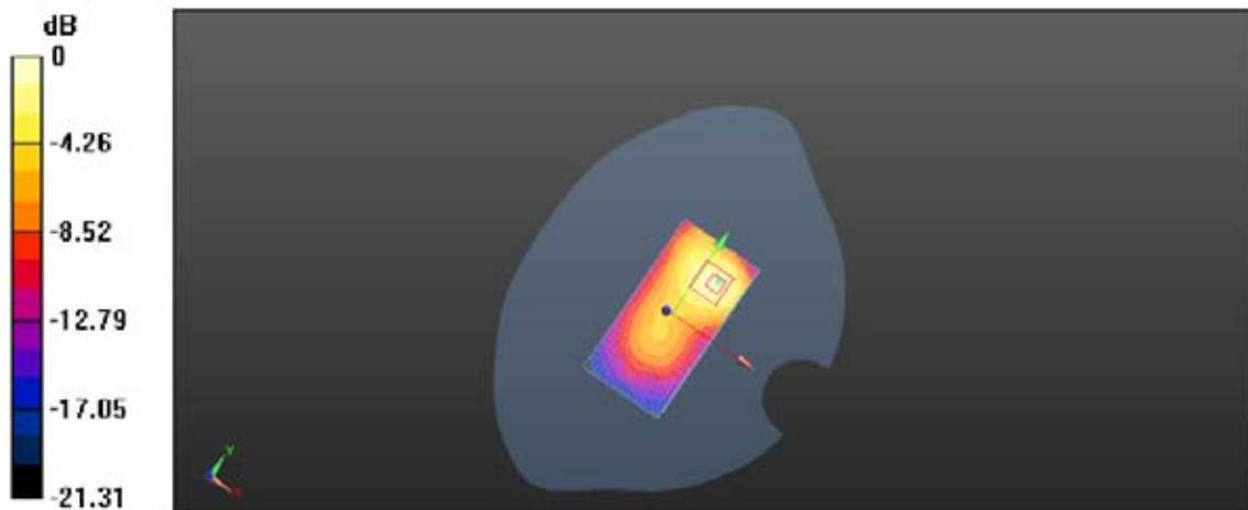
Plot 3: Body Left Side (GSM850 GPRS 2TS Middle Channel)
