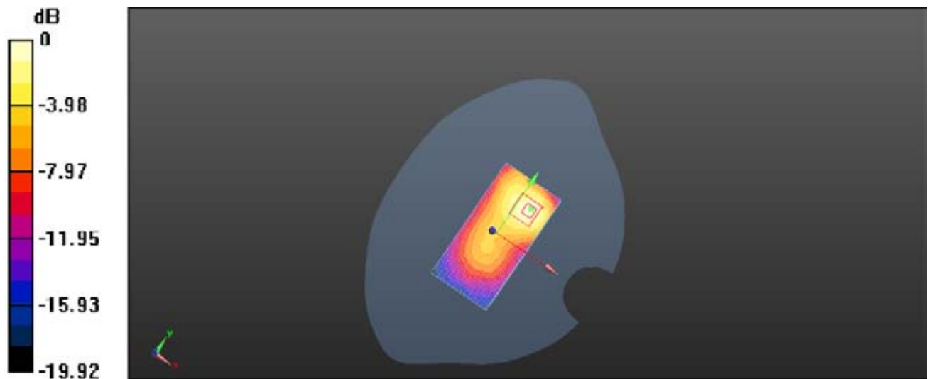
Plot 10: Body Right Side (GSM1900 GPRS 2TS Middle Channel)
