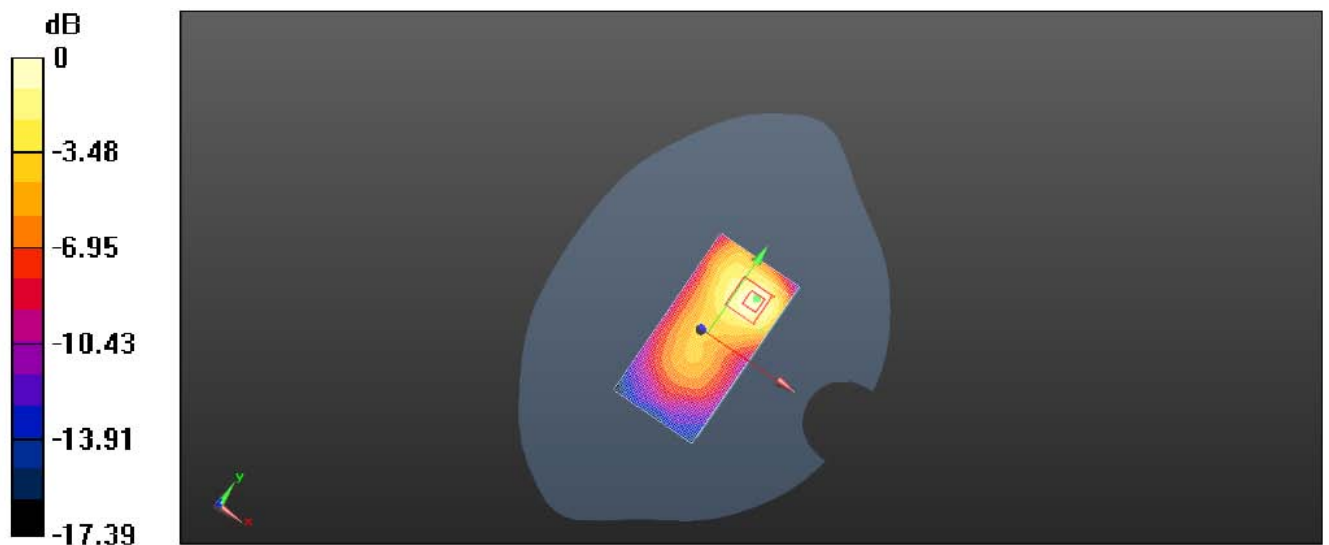
Plot 9: Body Left Side (GSM1900 GPRS 2TS Middle Channel)
