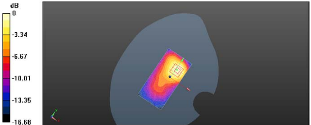
Plot 1: Body Front Side (GSM850 GPRS 2TS Middle Channel)
