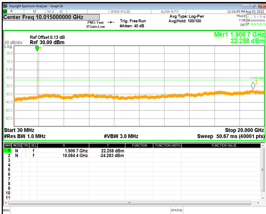
HSDPA Band2 Subtest2 Channel=9538
