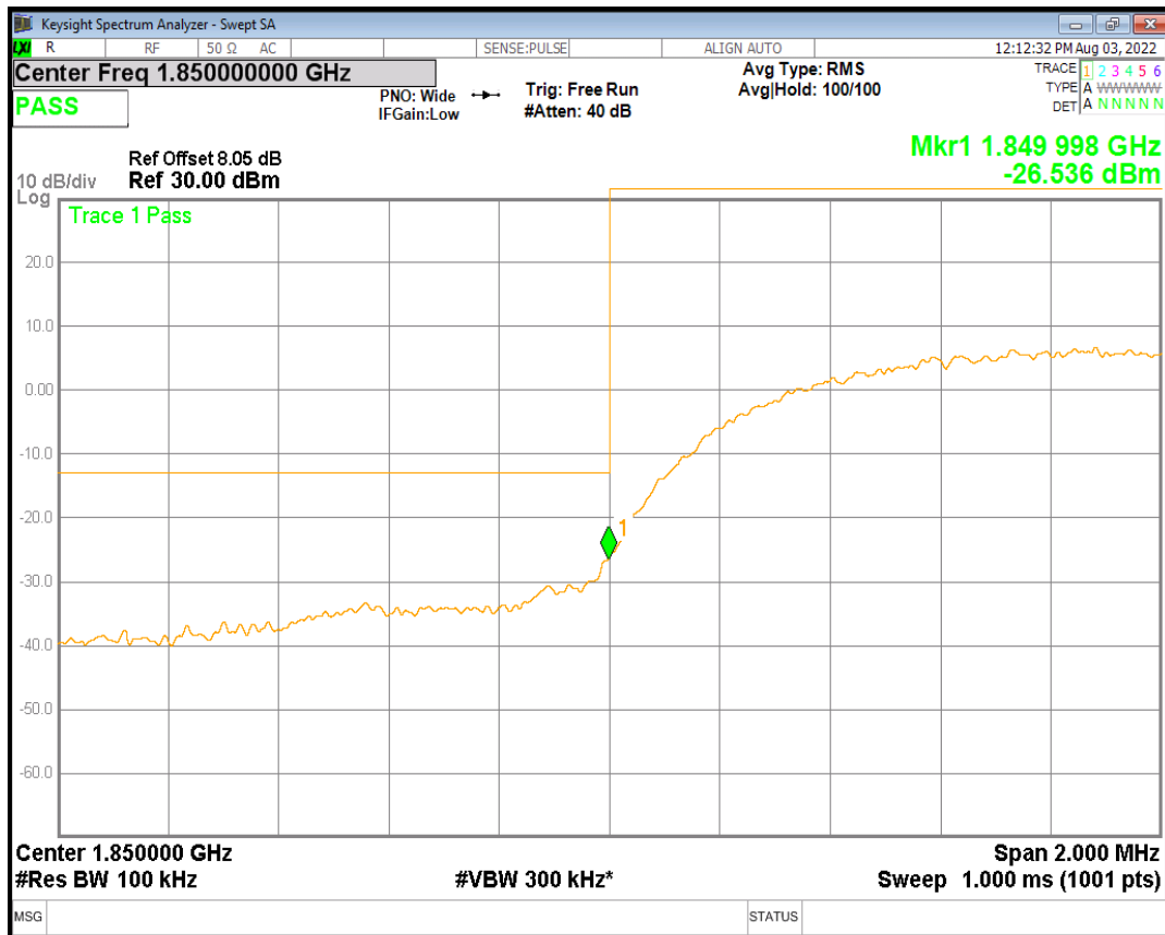
HSDPA Band2 Subtest4 Channel=9262
