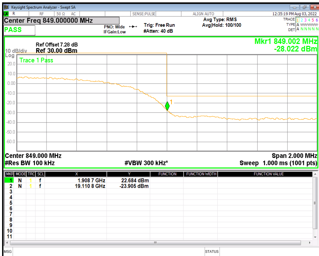
HSDPA Band5 Subtest3 Channel=4233
