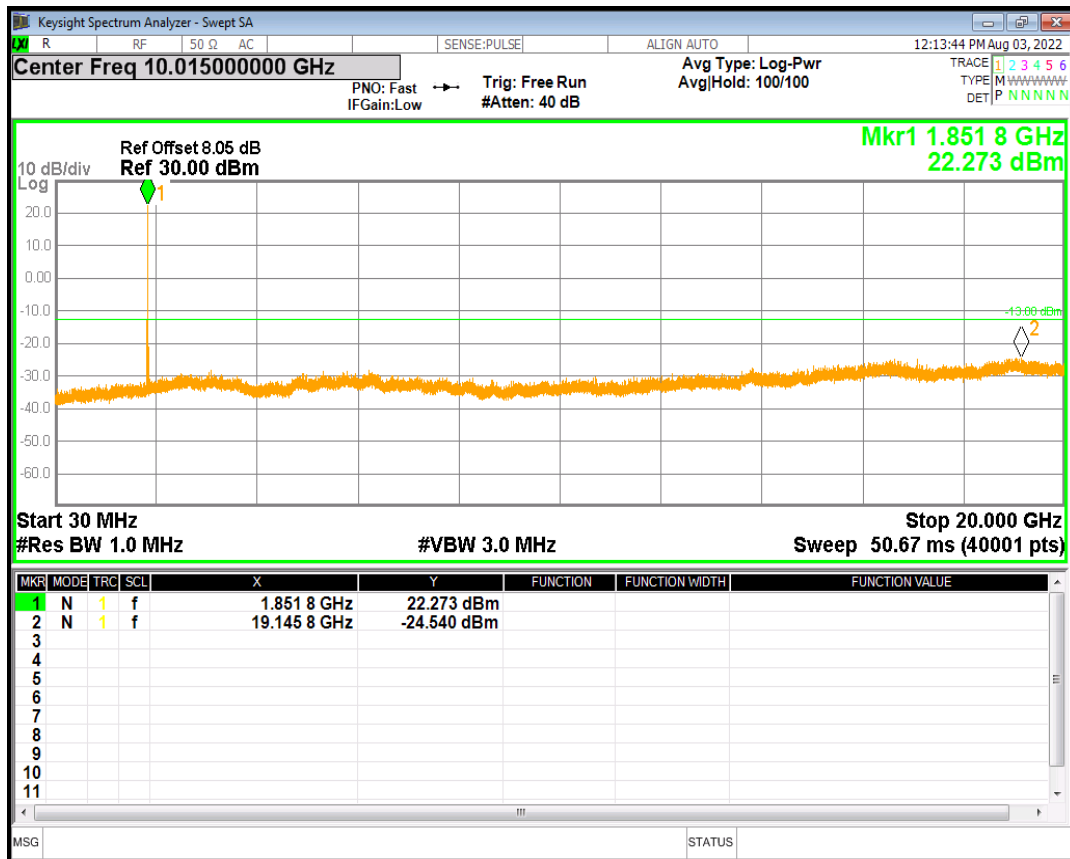
HSDPA Band2 Subtest3 Channel=9262
