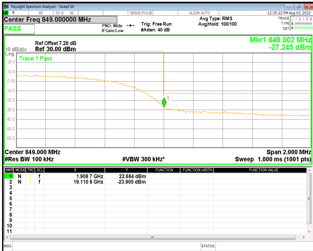
HSDPA Band5 Subtest4 Channel=4233
