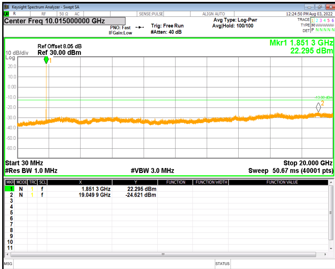
HSUPA Band2 Subtest5 Channel=9262
