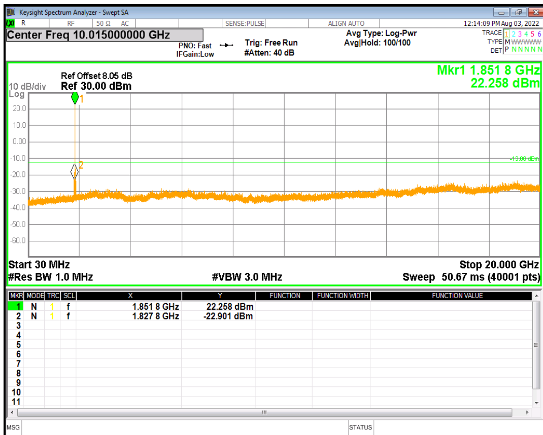
HSDPA Band2 Subtest4 Channel=9262
