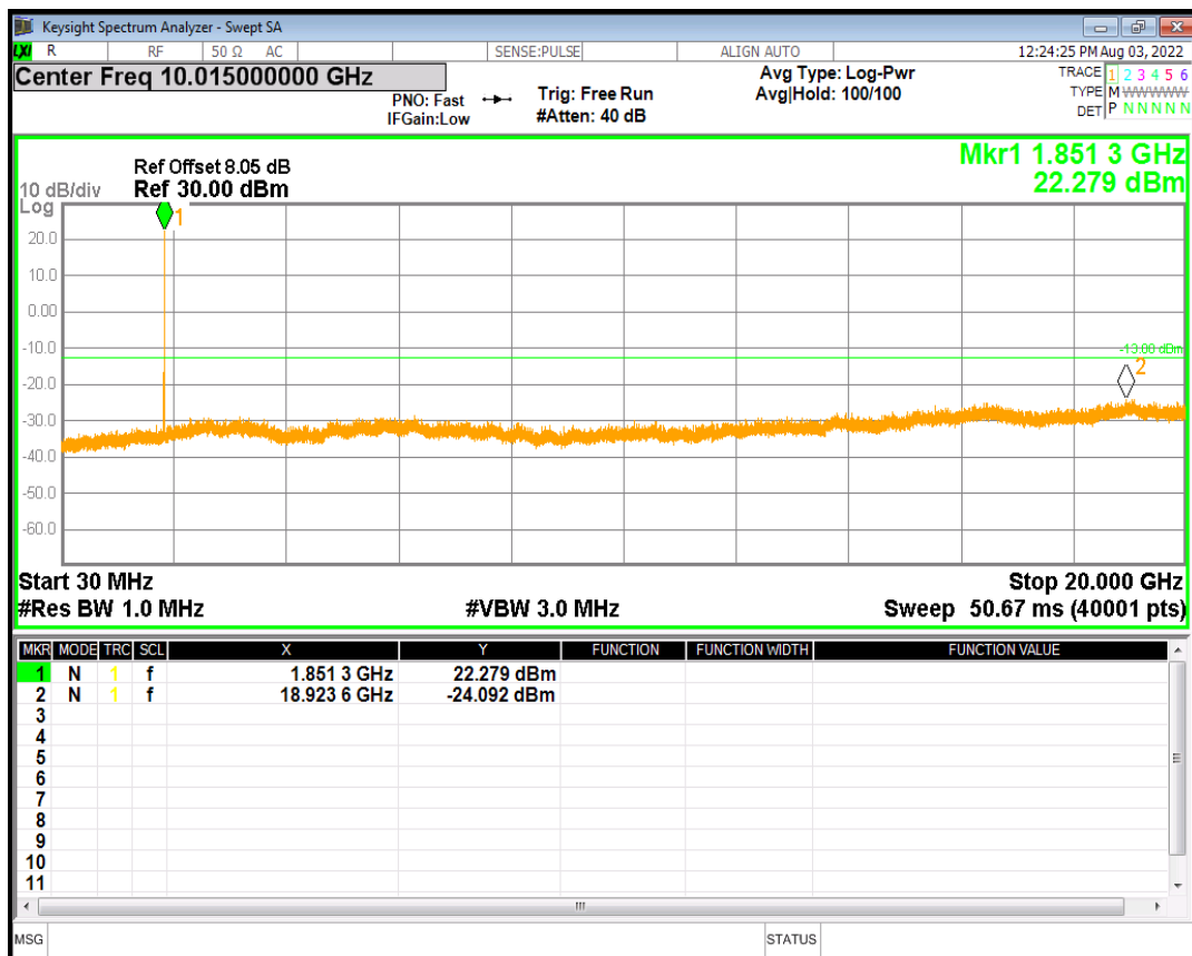
HSUPA Band2 Subtest4 Channel=9262
