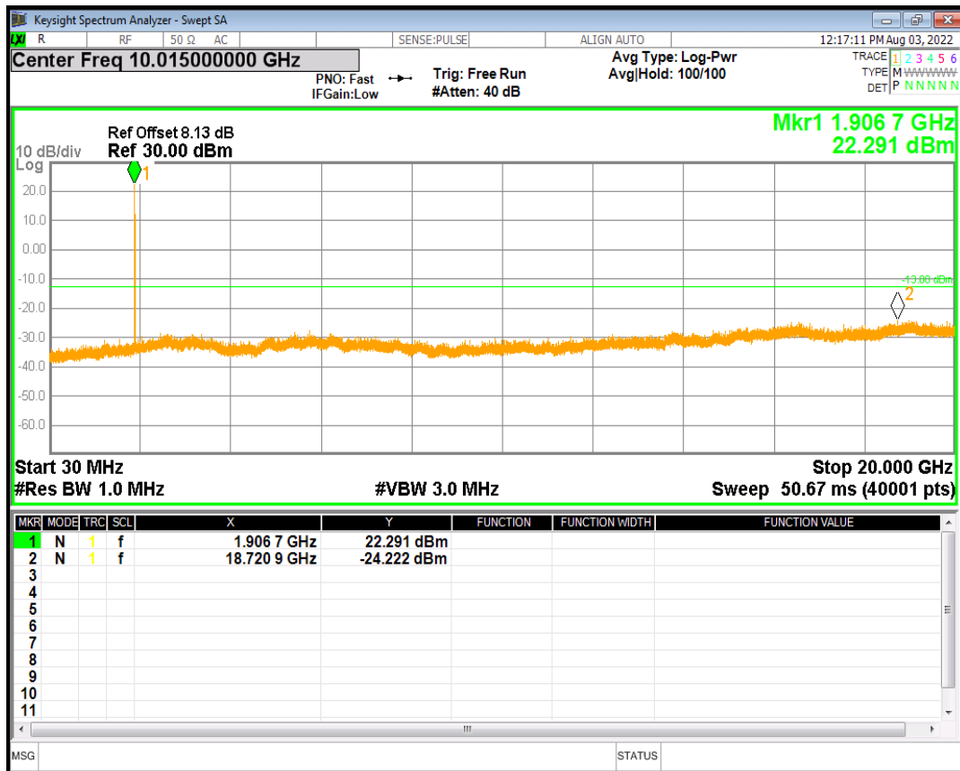
HSDPA Band2 Subtest3 Channel=9538
