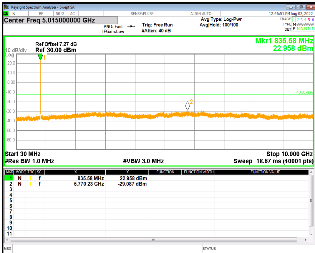
HSUPA Band5 Subtest3 Channel=4182
