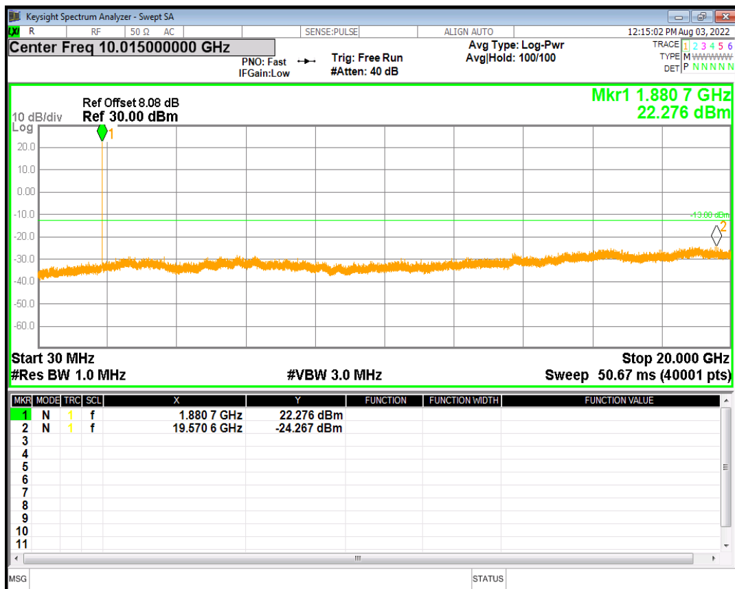
HSDPA Band2 Subtest2 Channel=9400
