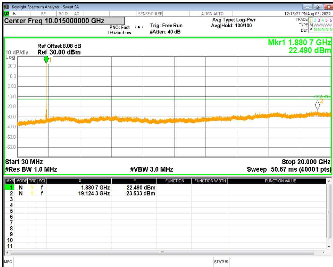
HSDPA Band2 Subtest3 Channel=9400
