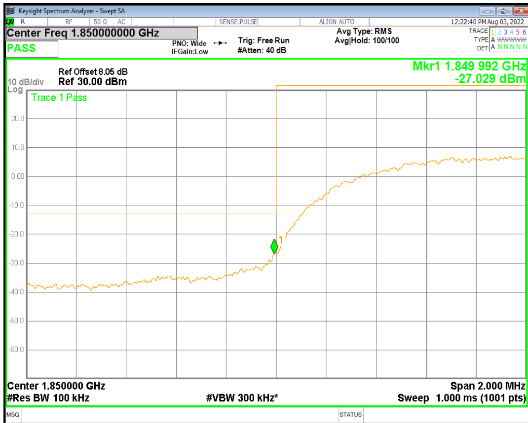
HSUPA Band2 Subtest4 Channel=9262
