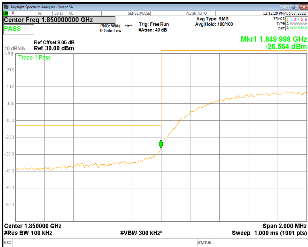
HSDPA Band2 Subtest3 Channel=9262
