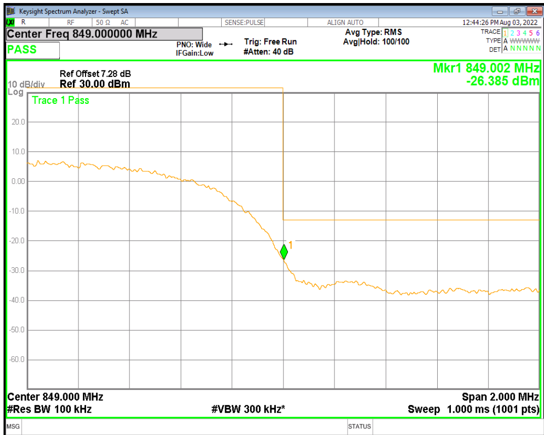
HSUPA Band5 Subtest3 Channel=4233
