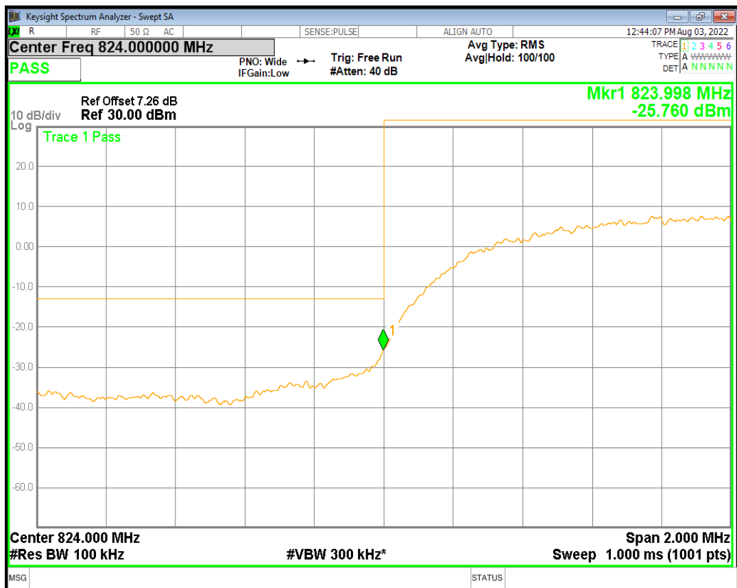
HSUPA Band5 Subtest3 Channel=4132
