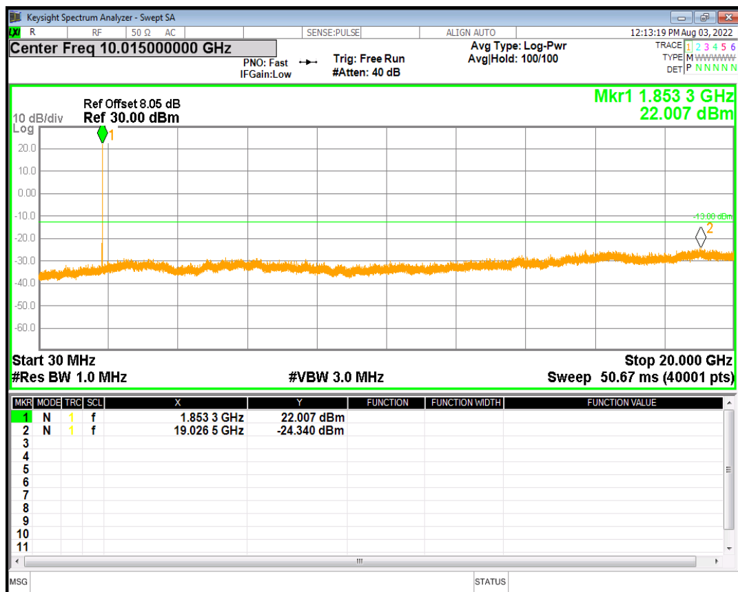
HSDPA Band2 Subtest2 Channel=9262
