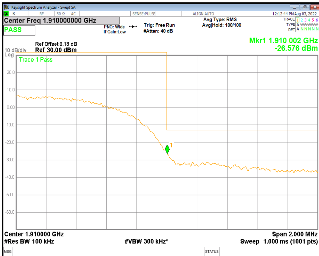
HSDPA Band2 Subtest3 Channel=9538
