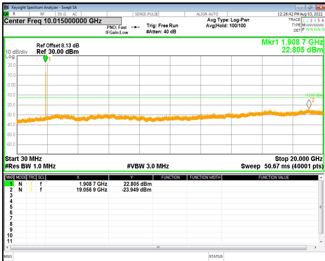
HSUPA Band2 Subtest4 Channel=9538
