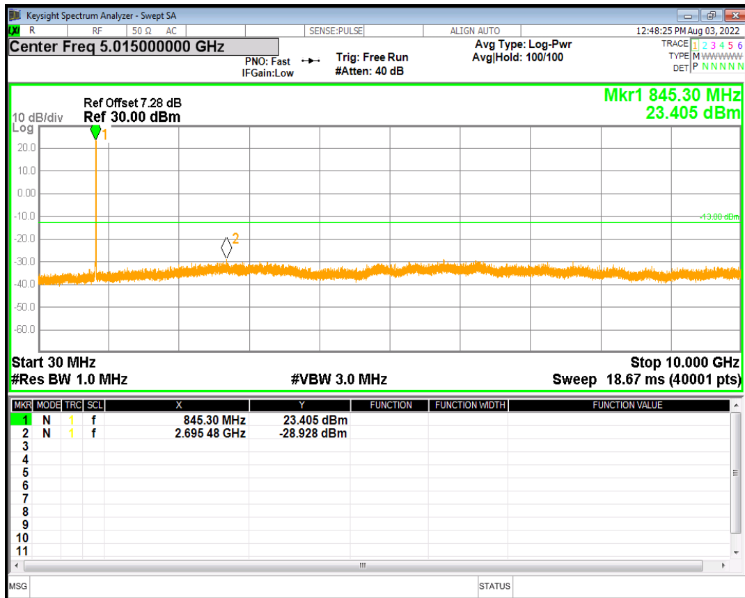
HSUPA Band5 Subtest3 Channel=4233
