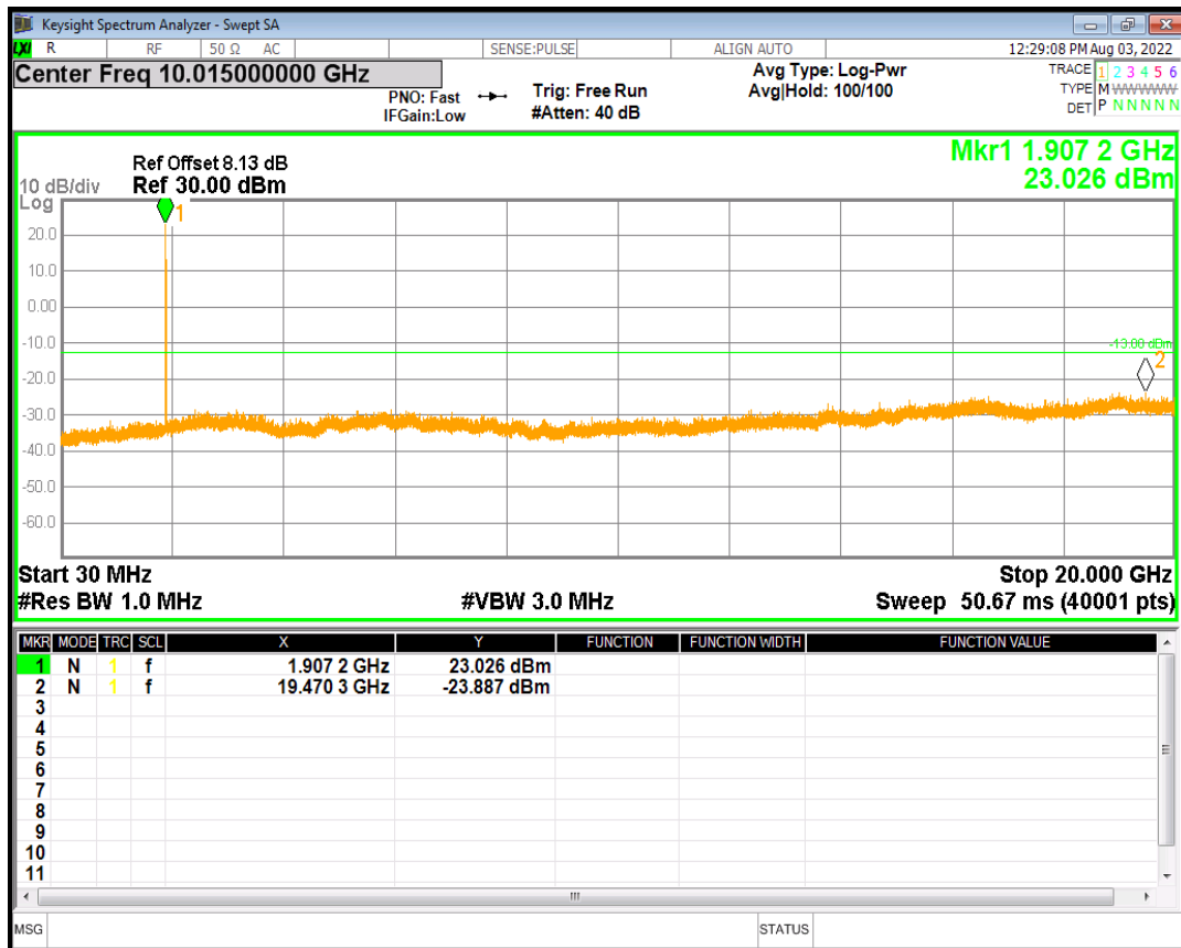
HSUPA Band2 Subtest5 Channel=9538
