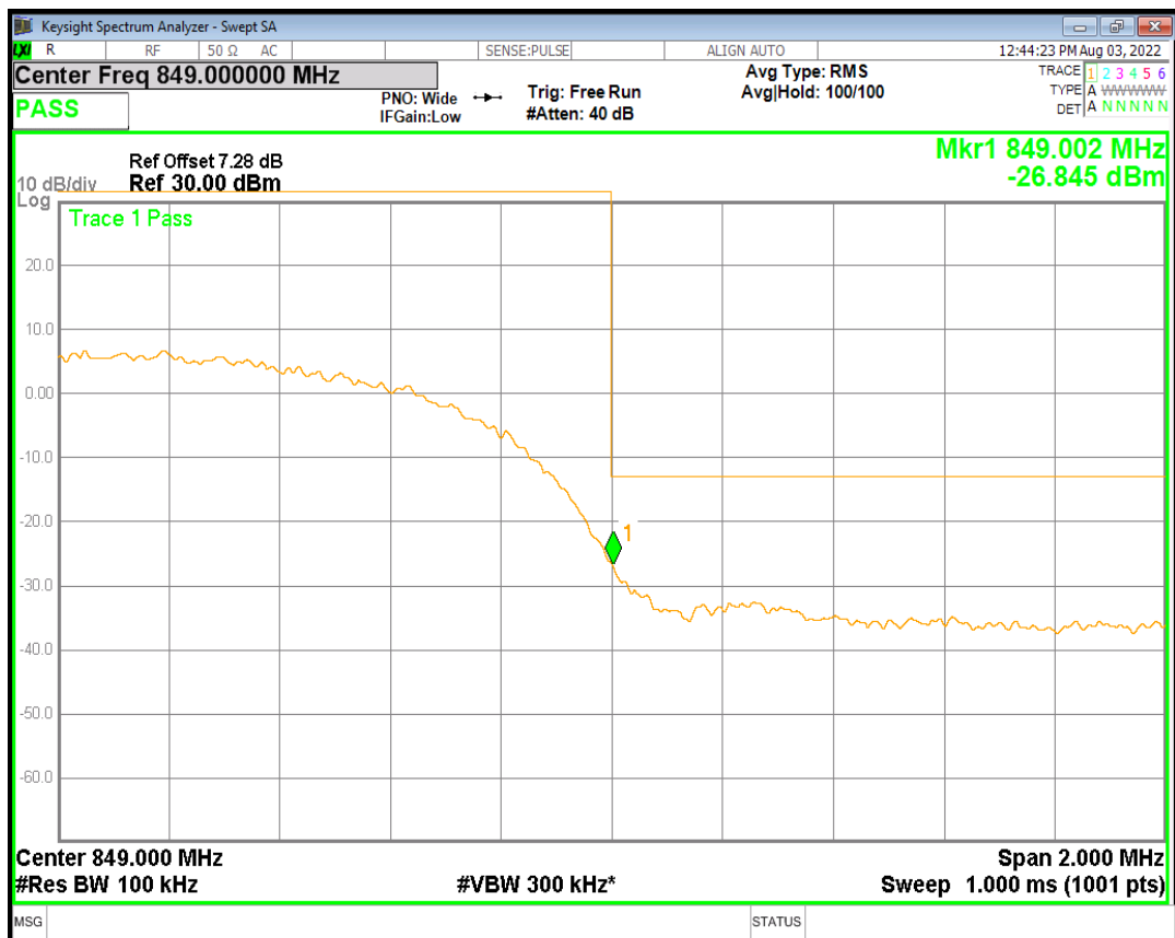
HSUPA Band5 Subtest2 Channel=4233
