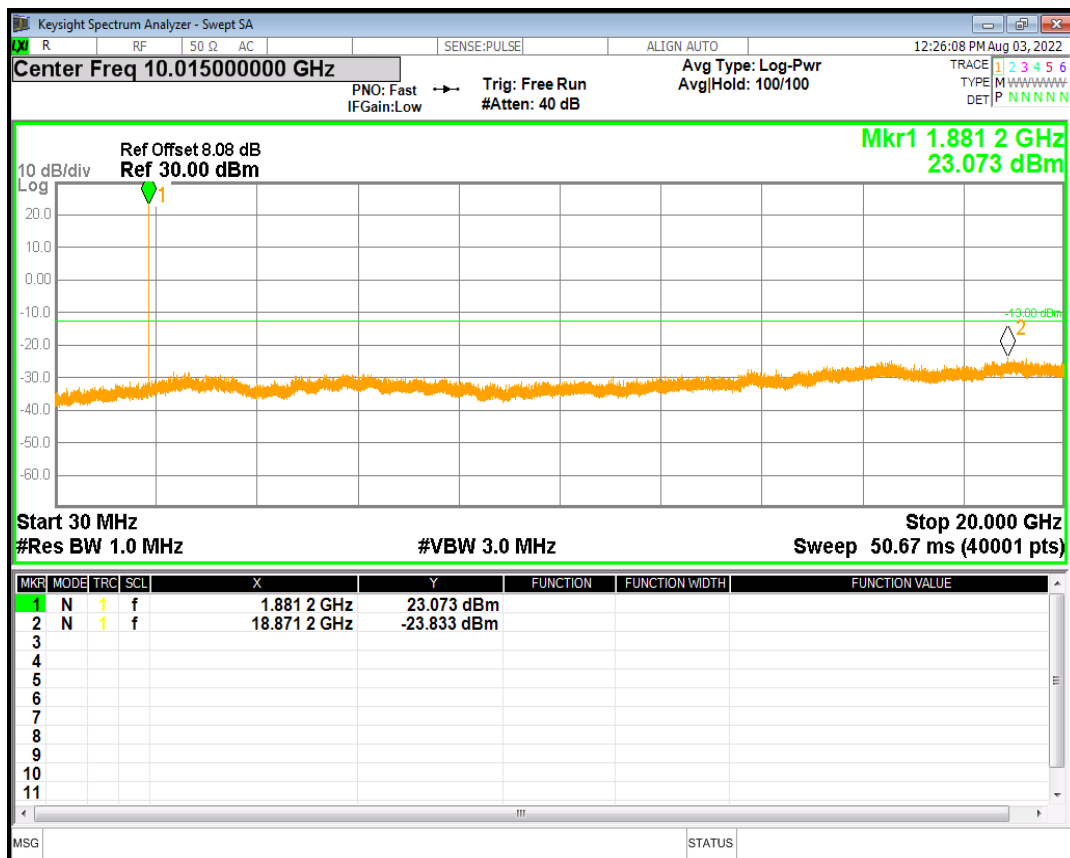
HSUPA Band2 Subtest3 Channel=9400
