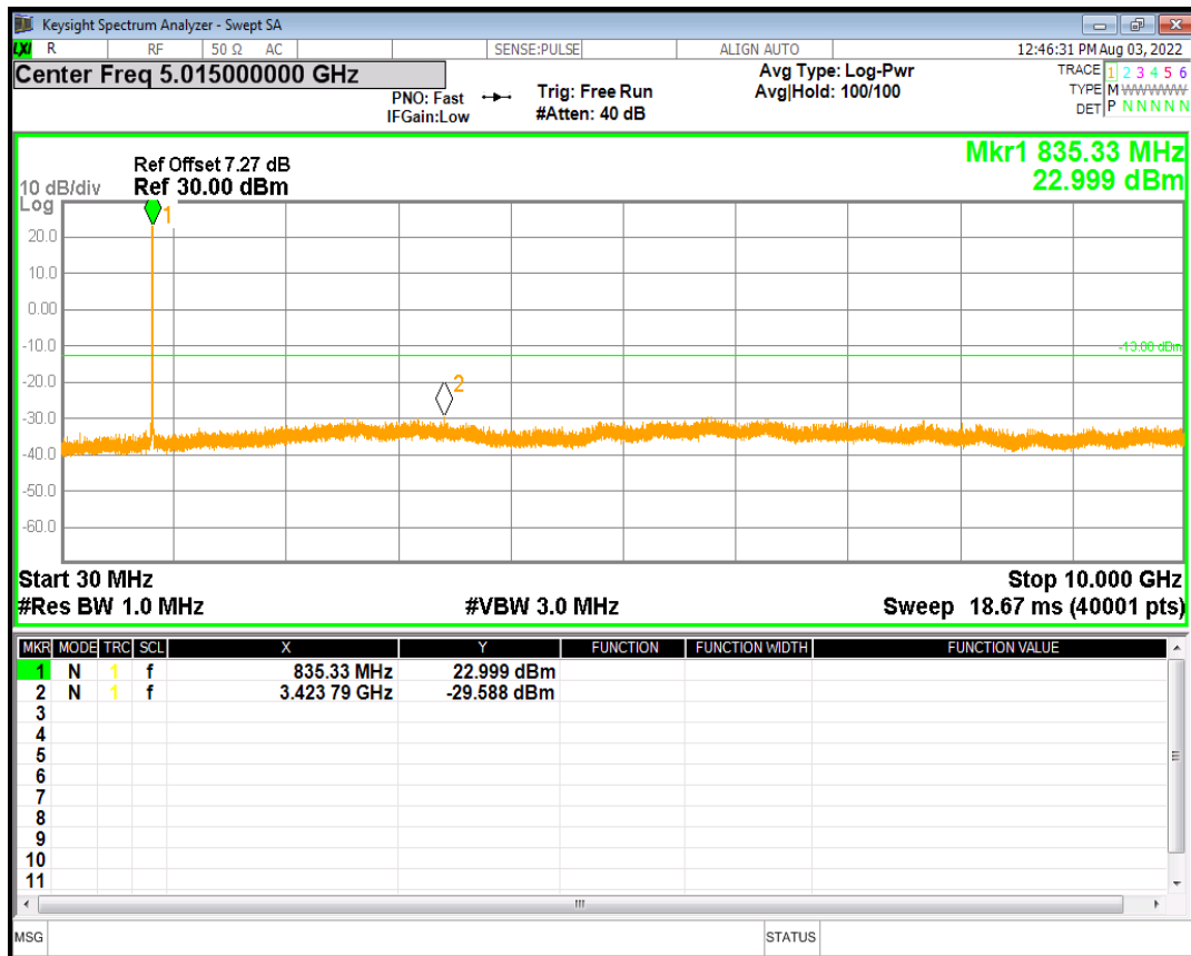
HSUPA Band5 Subtest2 Channel=4182
