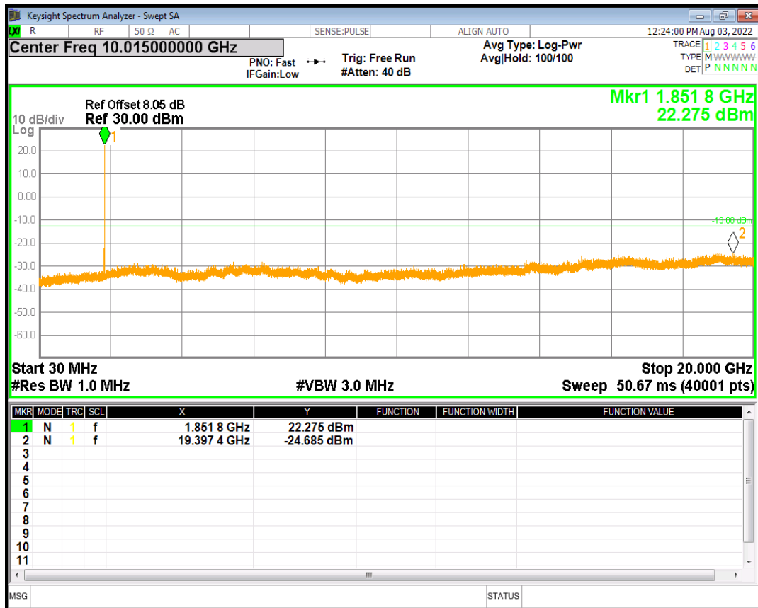
HSUPA Band2 Subtest3 Channel=9262
