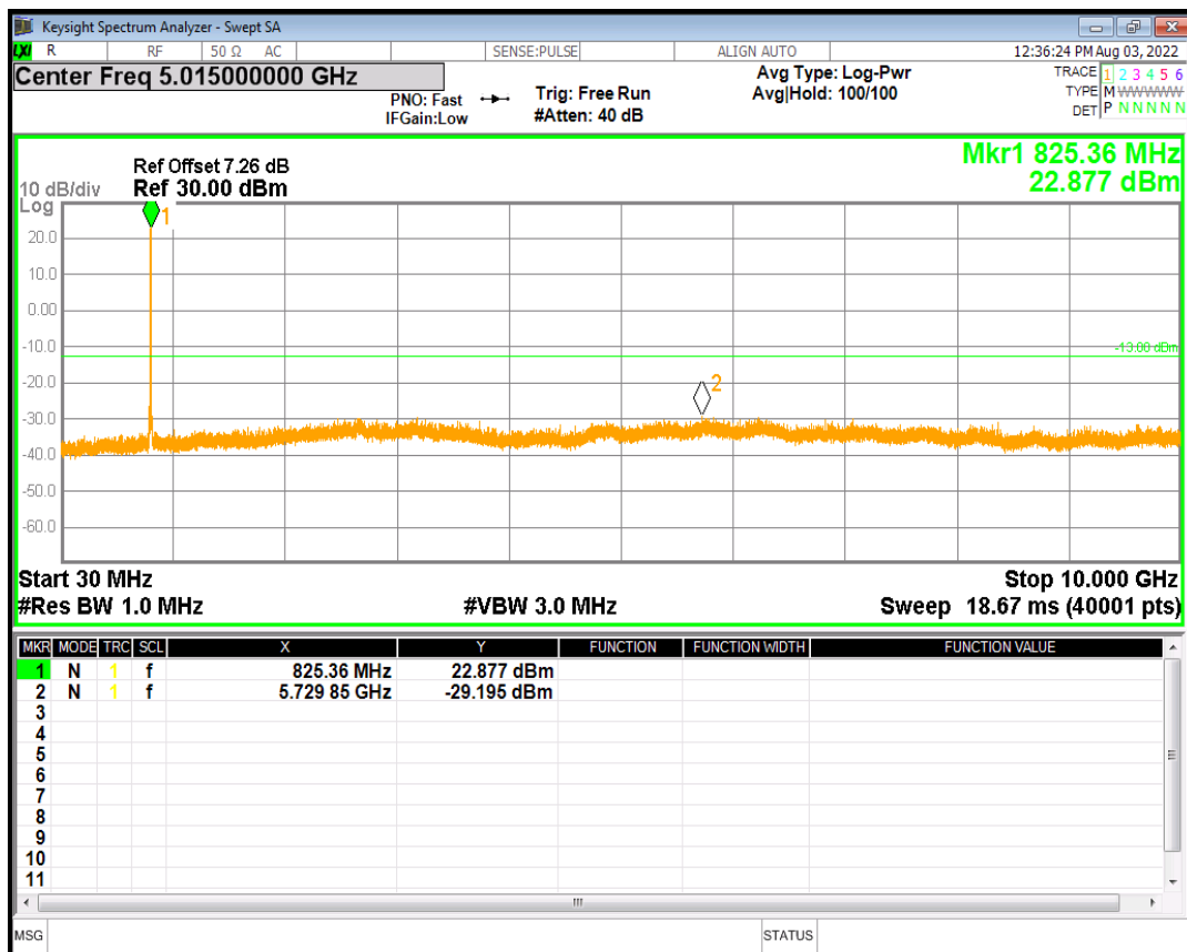
HSDPA Band5 Subtest4 Channel=4132
