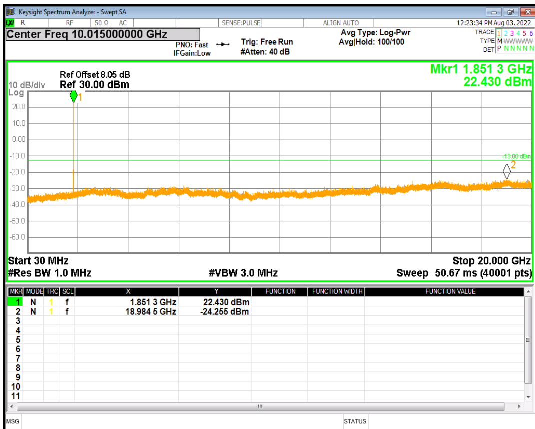
HSUPA Band2 Subtest2 Channel=9262
