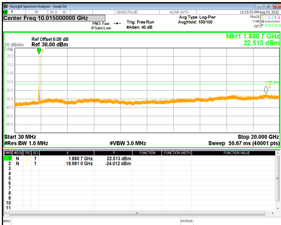
HSDPA Band2 Subtest4 Channel=9400
