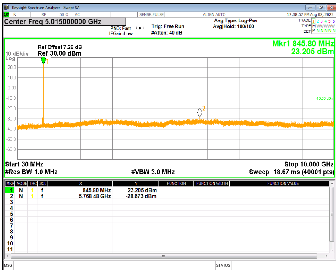
HSDPA Band5 Subtest4 Channel=4233
