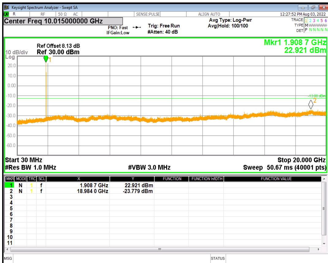
HSUPA Band2 Subtest2 Channel=9538
