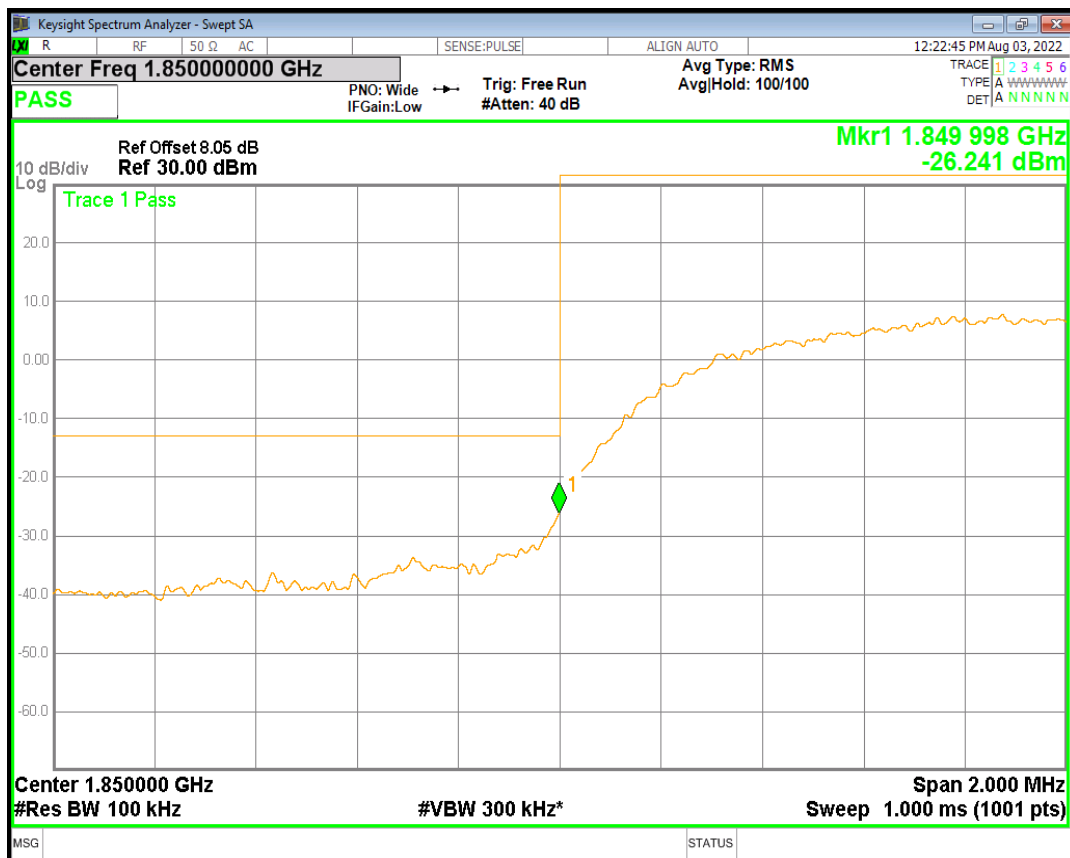
HSUPA Band2 Subtest5 Channel=9262
