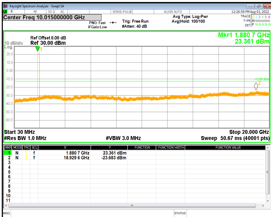
HSUPA Band2 Subtest5 Channel=9400
