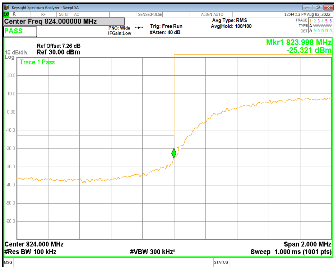
HSUPA Band5 Subtest5 Channel=4132
