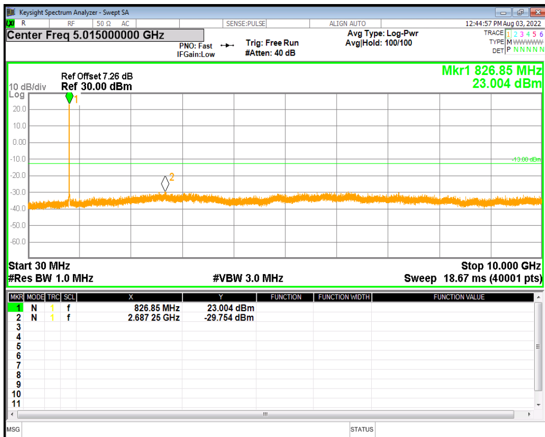
HSUPA Band5 Subtest2 Channel=4132
