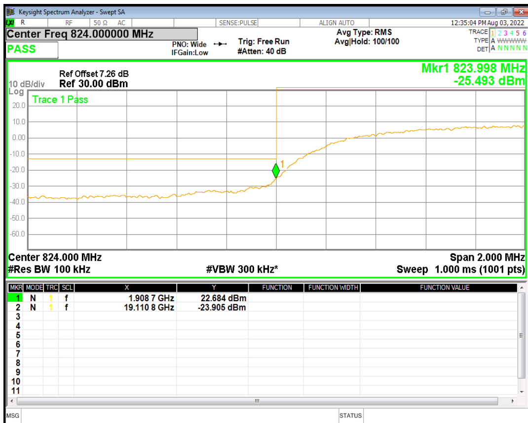
HSDPA Band5 Subtest3 Channel=4132
