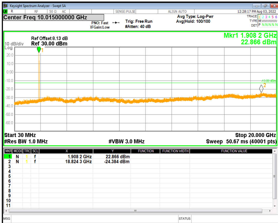
HSUPA Band2 Subtest3 Channel=9538
