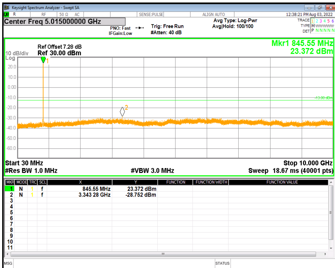
HSDPA Band5 Subtest2 Channel=4233
