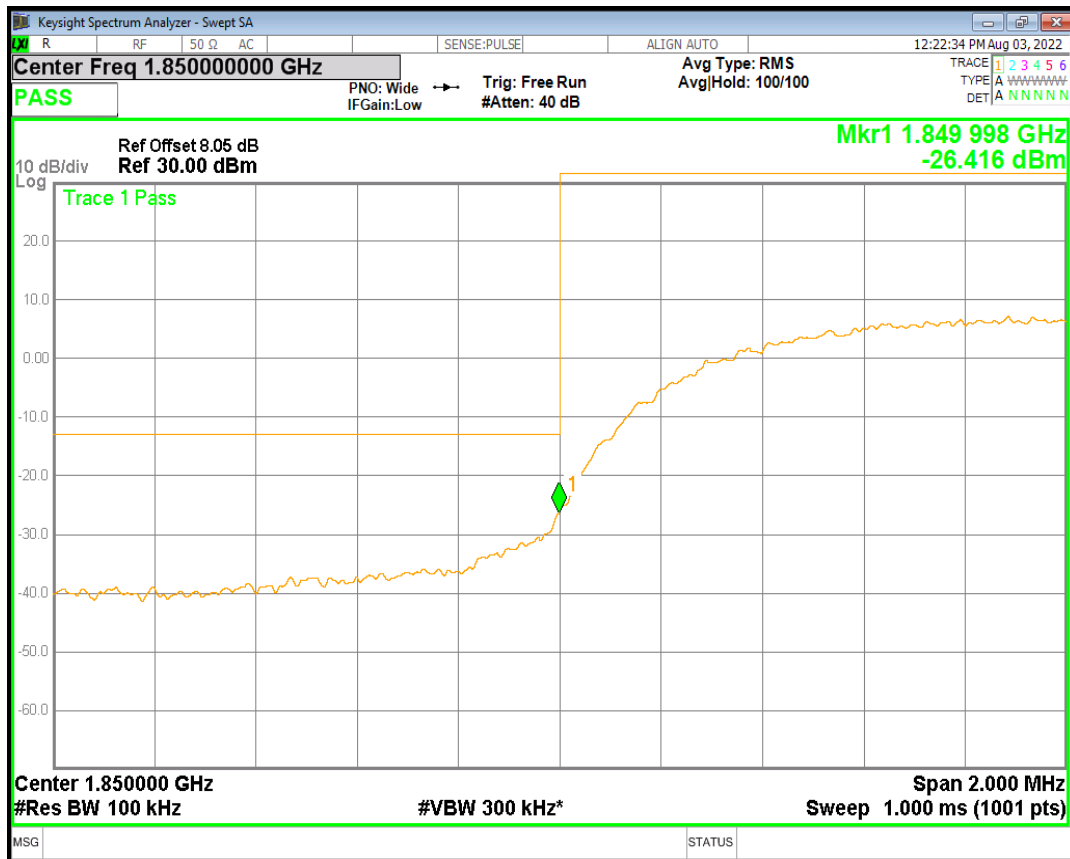
HSUPA Band2 Subtest2 Channel=9262
