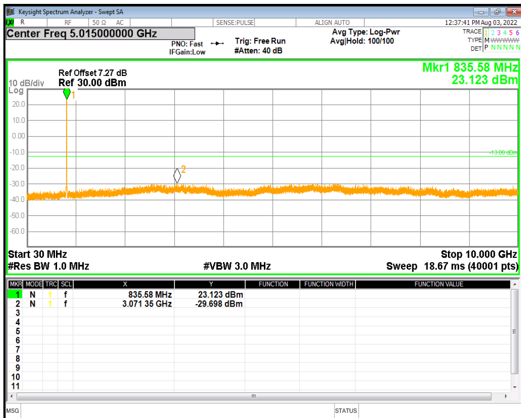
HSDPA Band5 Subtest4 Channel=4182
