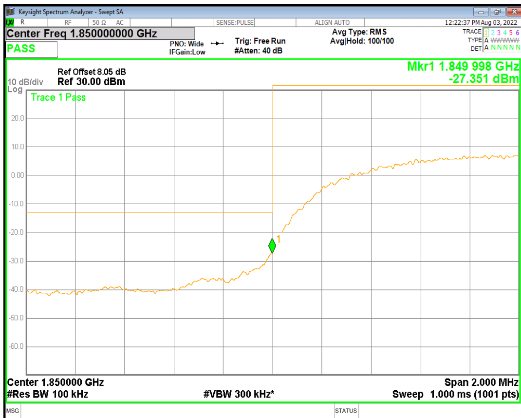
HSUPA Band2 Subtest3 Channel=9262
