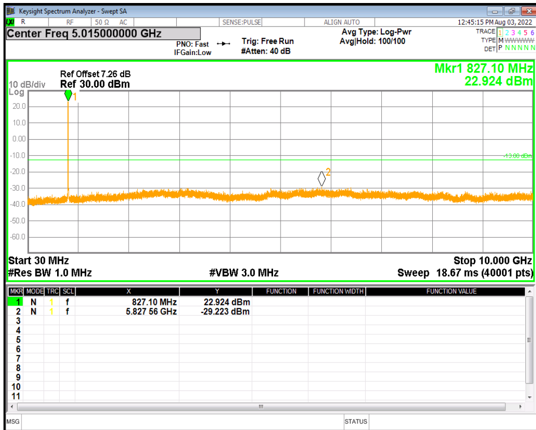
HSUPA Band5 Subtest3 Channel=4132
