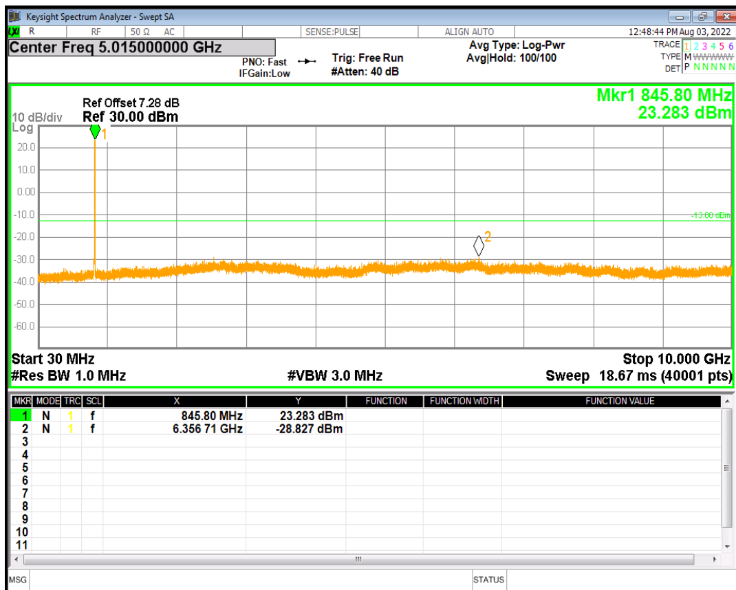
HSUPA Band5 Subtest4 Channel=4233
