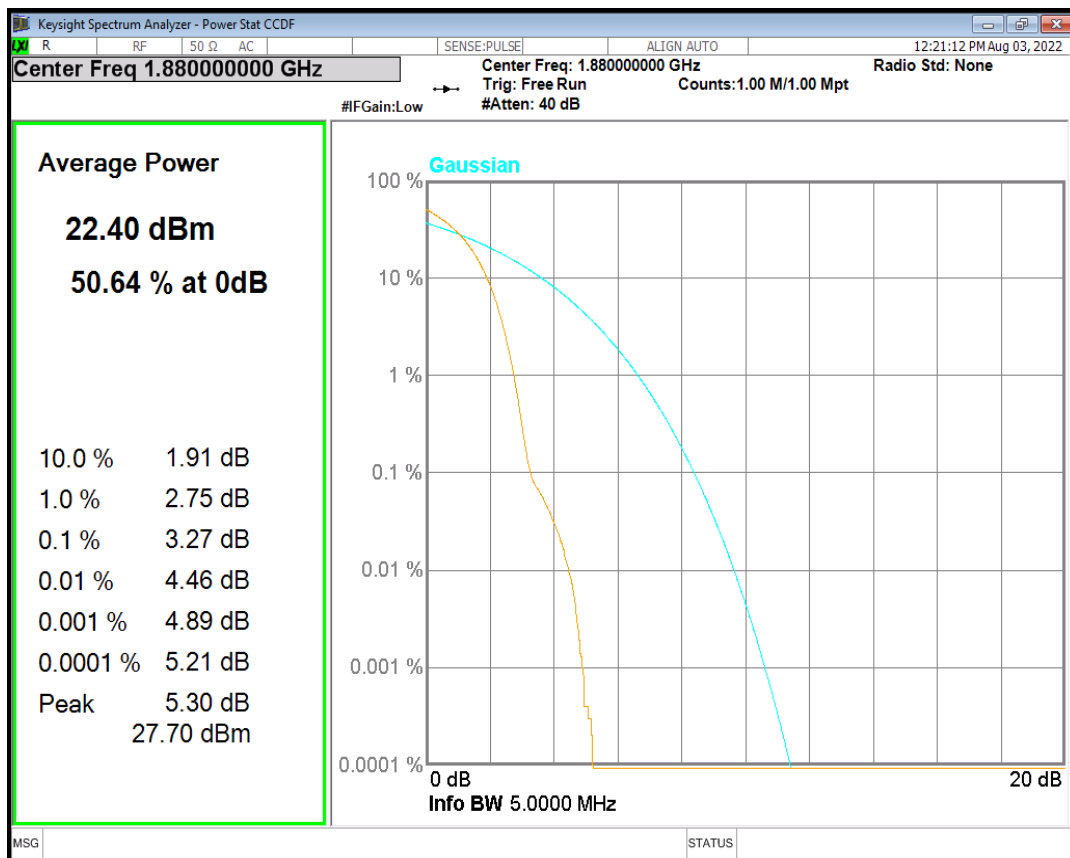
HSDPA Band2 Subtest5 Channel=9400
