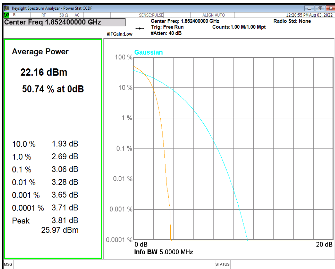
HSDPA Band2 Subtest5 Channel=9262
