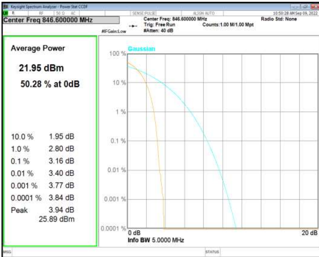
HSDPA Band5 Subtest5 Channel=4233
