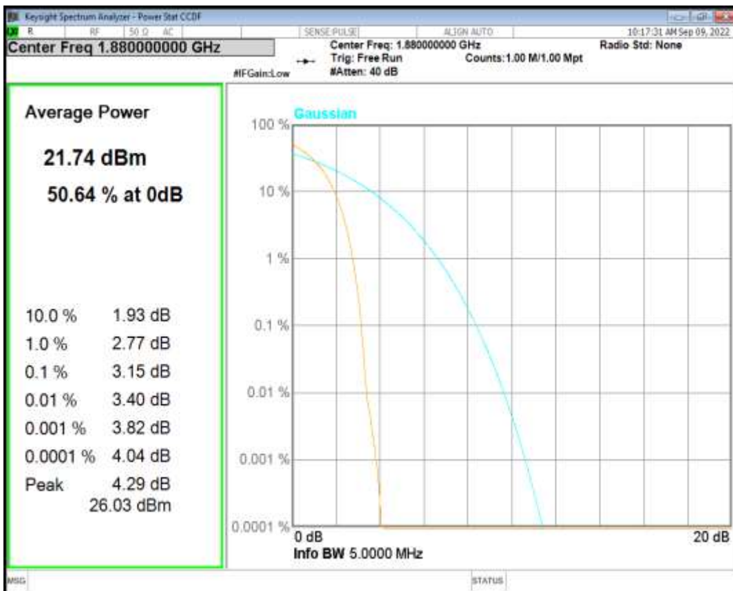
HSDPA Band2 Subtest5 Channel=9400
