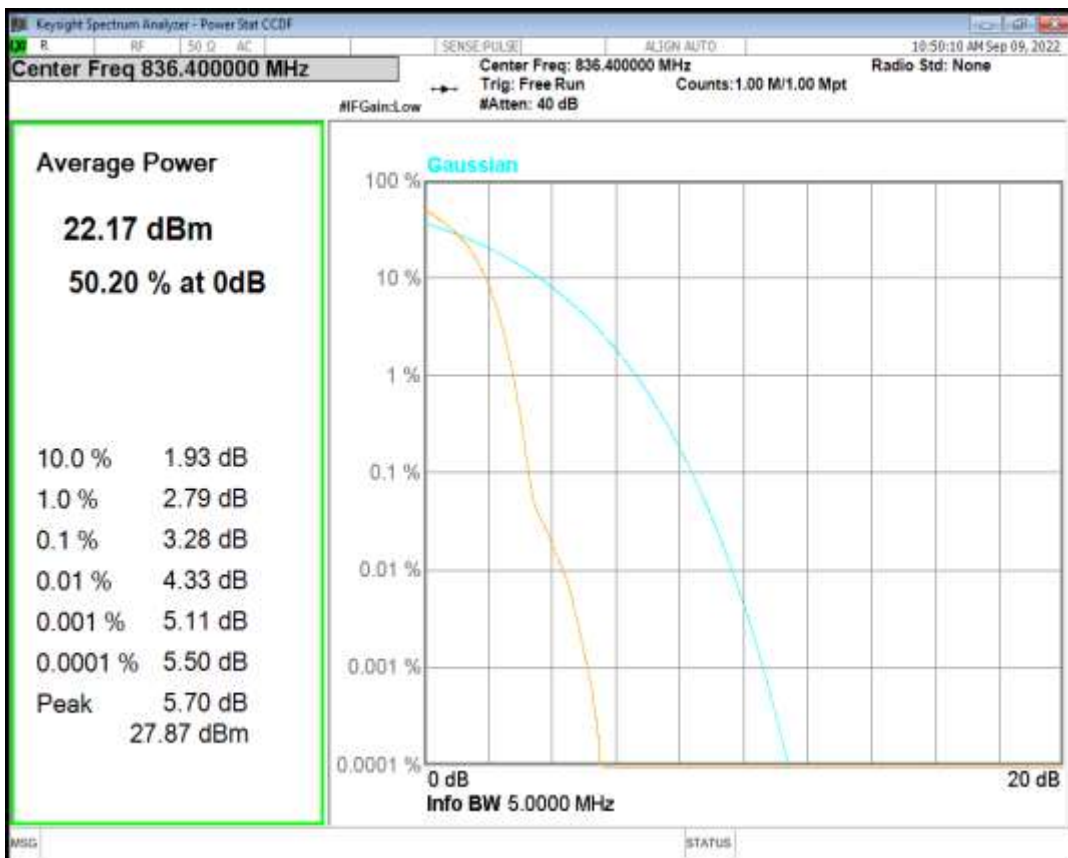
HSDPA Band5 Subtest5 Channel=4182
