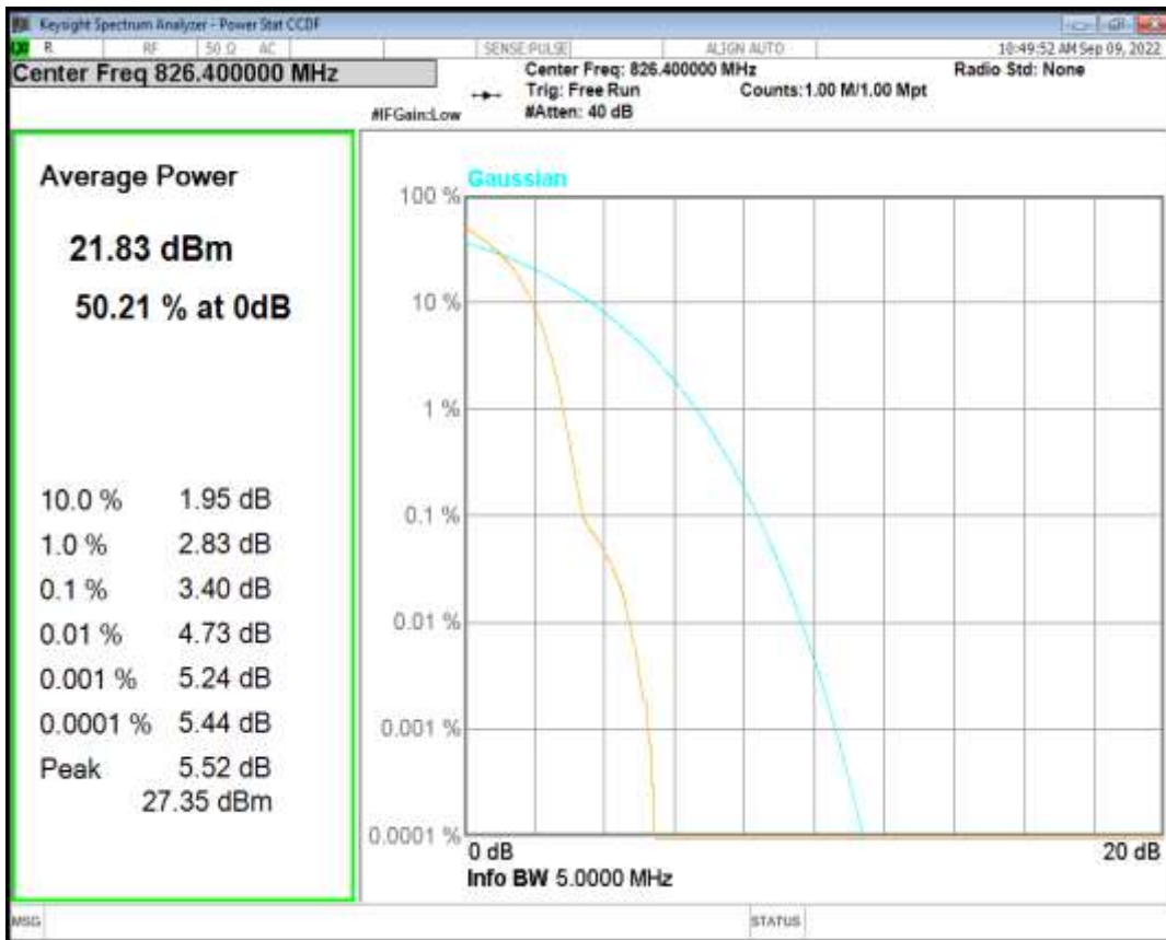
HSDPA Band5 Subtest5 Channel=4132
