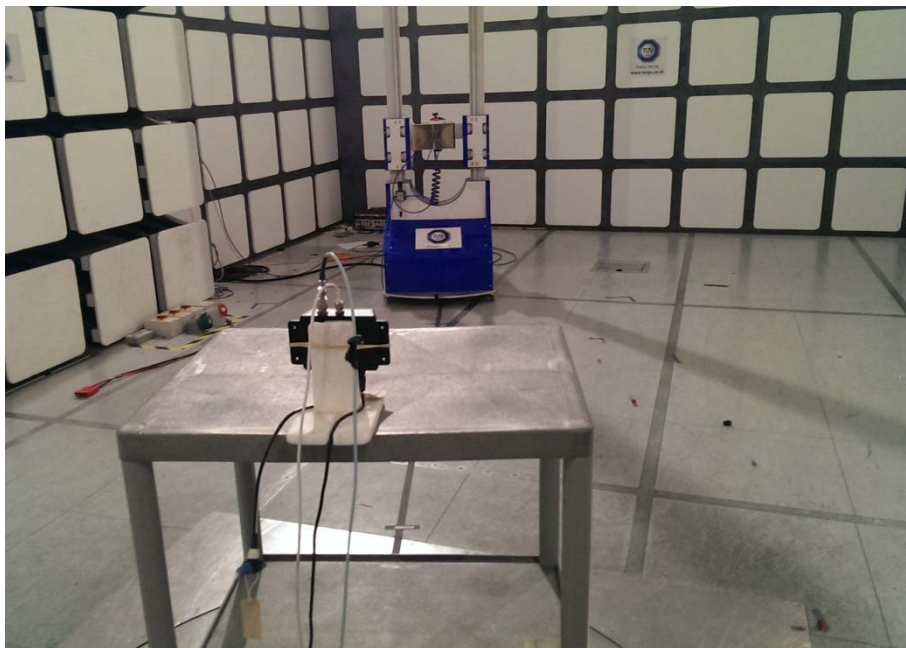
Emission Limitations (1 GHz to 2 GHz)
