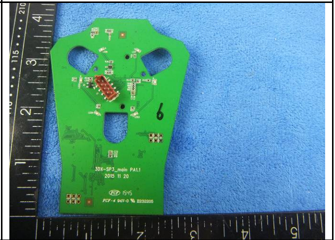
Mainboard Board Bottom View
