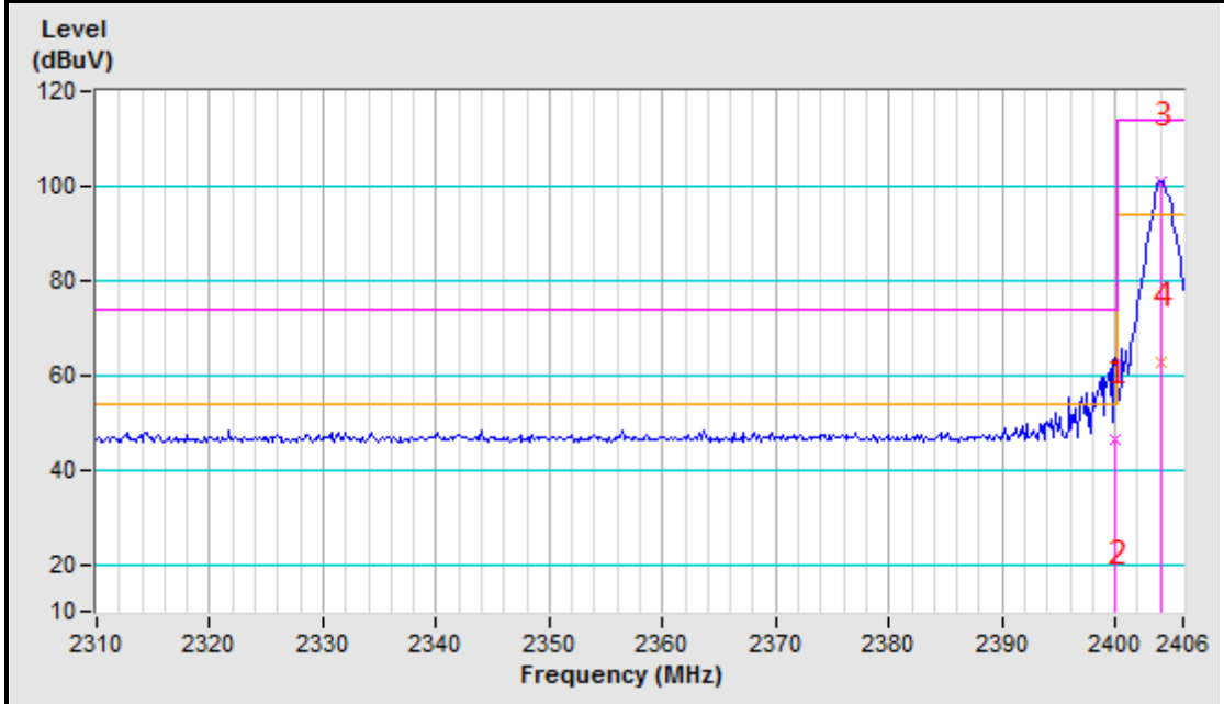
2404MHz Vertical
