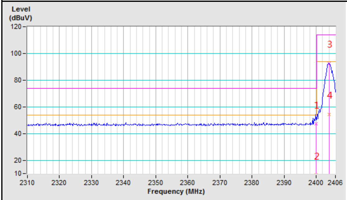
2404MHz Vertical
