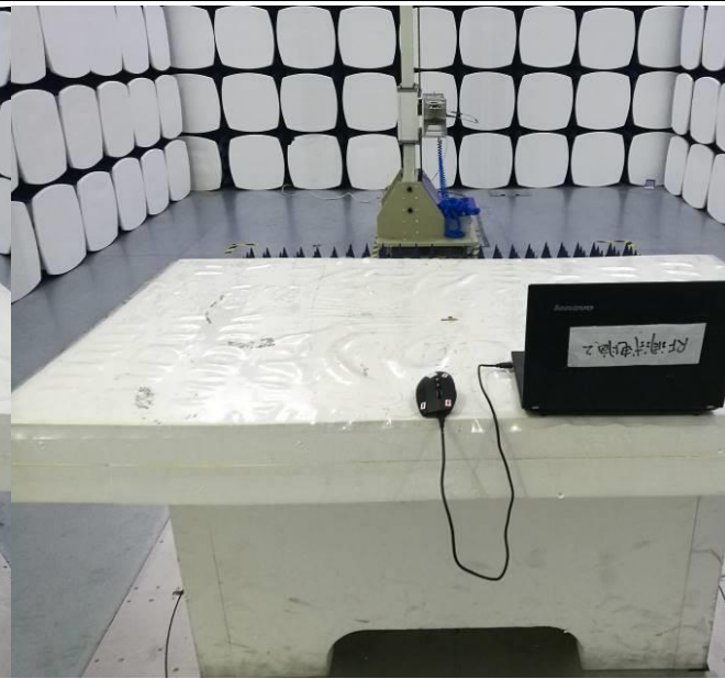
Radiated Emissions Test Setup Above 1GHz
