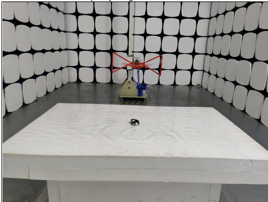
Frequency Range<30MHz~1GHz >
