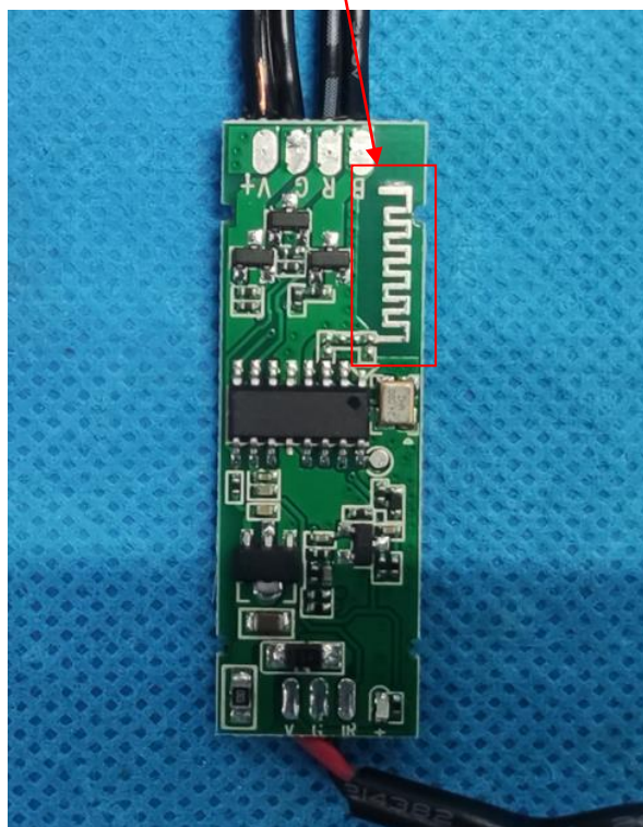
BT antenna
