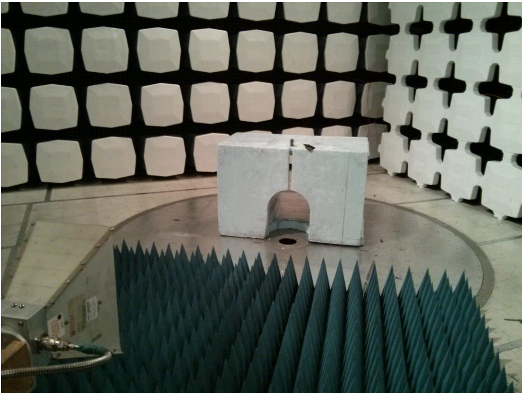
Figure 8: EUT Position Assessment
