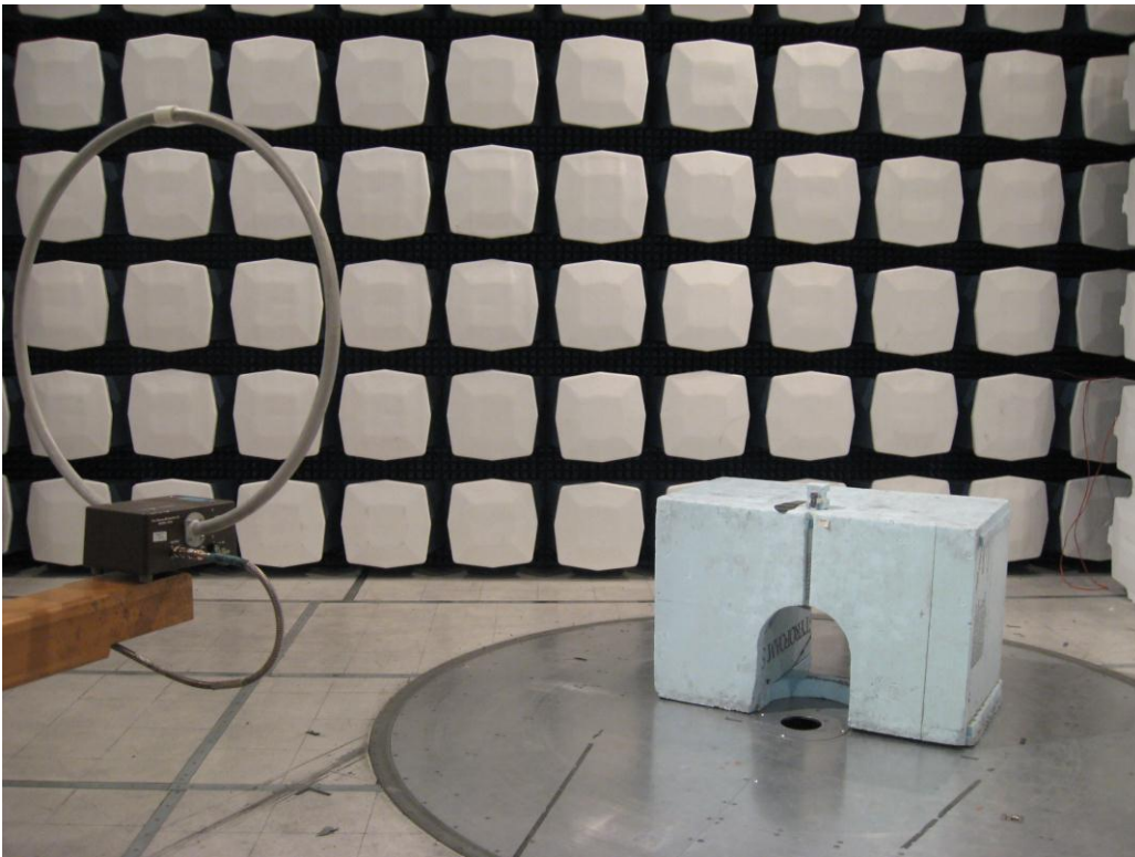
Figure 1: SSV2 Emissions below 30 MHz
