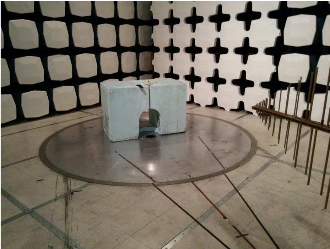
Figure 3: SSV2 Emissions 30 MHz to 1 GHz
