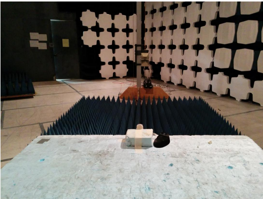
Figure 4: SSV2 Emissions above 1 GHz
