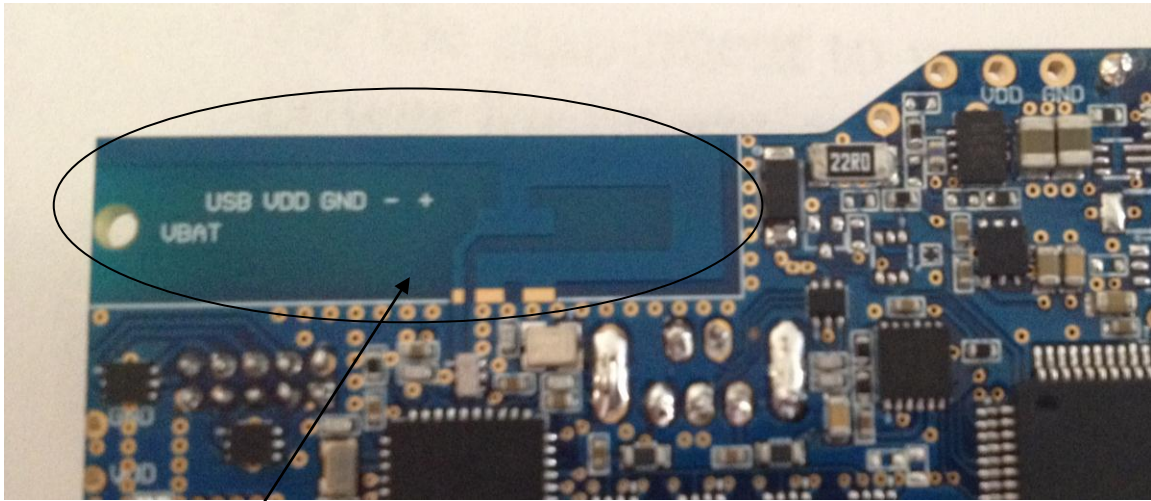
Figure 3: Internal antenna
