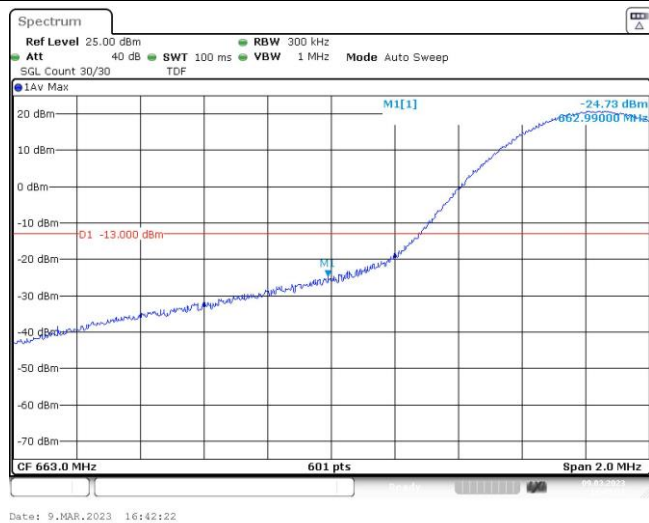
Band71-15MHz-16QAM-133197-1RB#74
