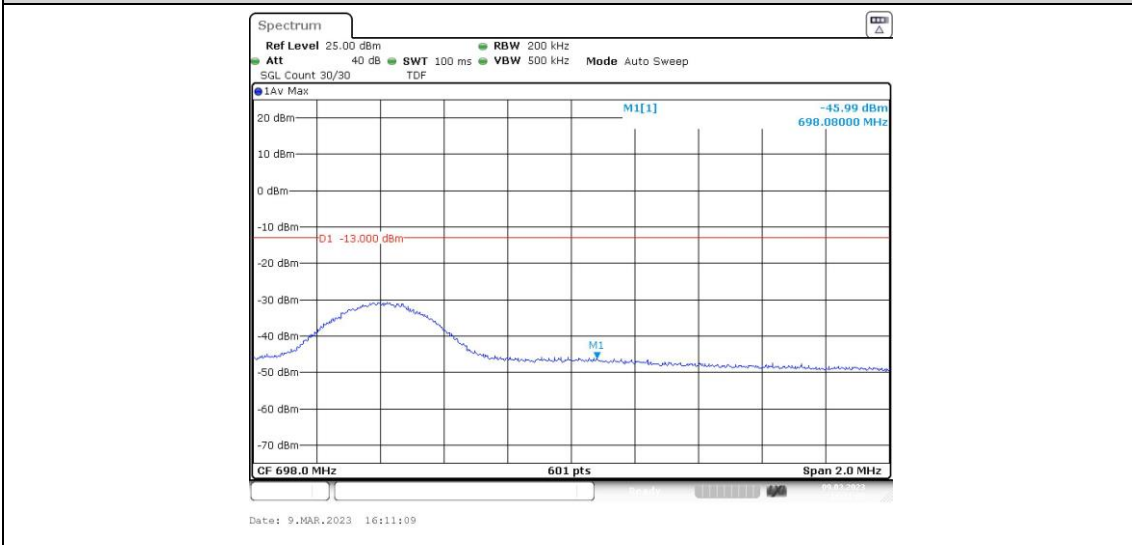
Band71-10MHz-16QAM-133422-1RB#49
