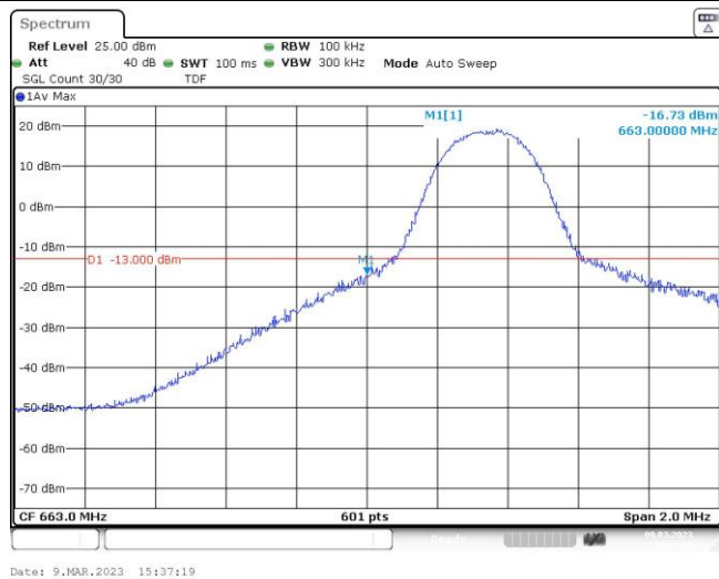
Band71-5MHz-16QAM-133147-1RB#24
