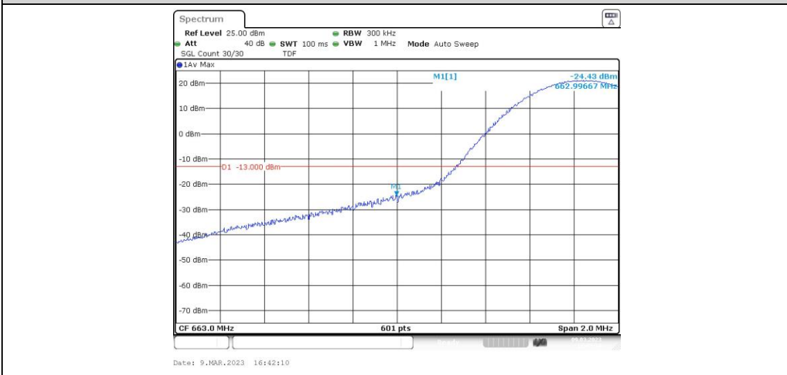
Band71-15MHz-QPSK-133197-1RB#74
