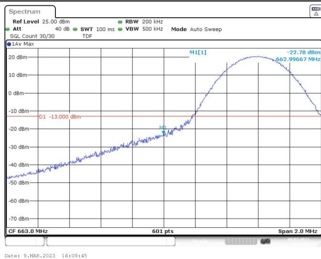
Band71-10MHz-16QAM-133172-1RB#49
