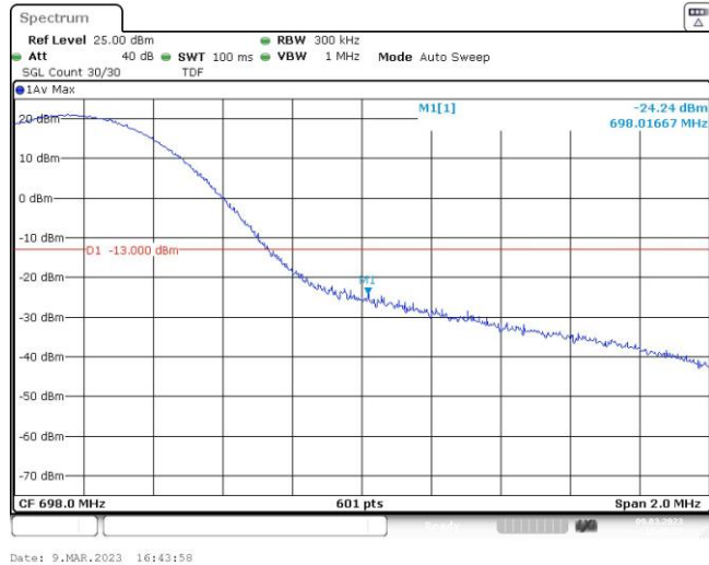
Band71-15MHz-QPSK-133397-75RB#0
