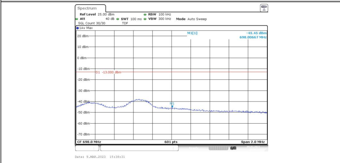
Band71-5MHz-QPSK-133447-1RB#24
