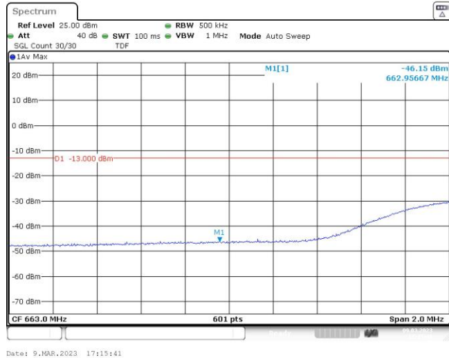
Band71-20MHz-QPSK-133222-100RB#0
