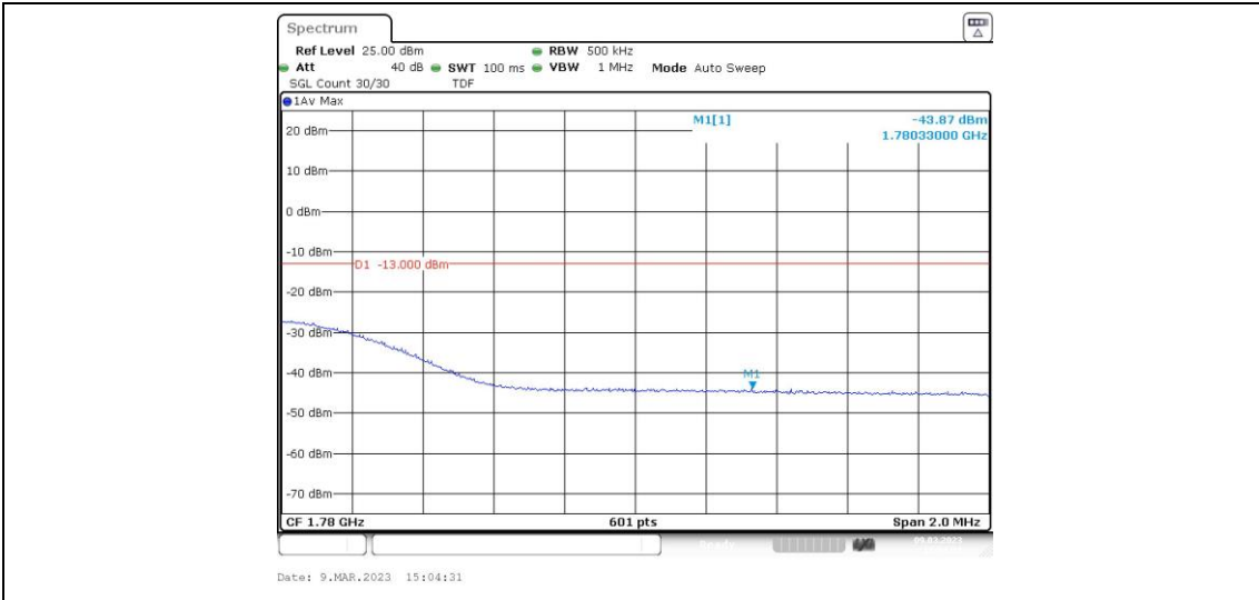
Band66-20MHz-16QAM-132572-1RB#99
