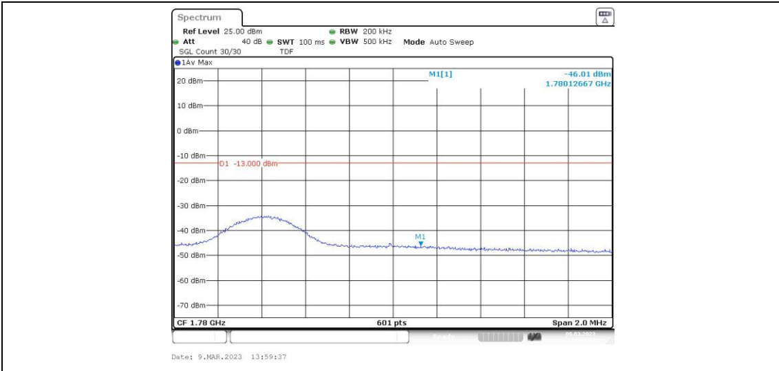
Band66-10MHz-16QAM-132622-1RB#49
