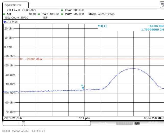
Band66-10MHz-16QAM-132022-50RB#0
