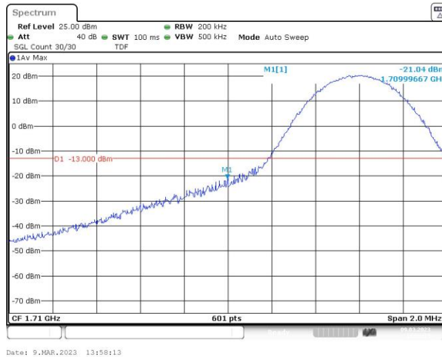
Band66-10MHz-16QAM-132022-1RB#49
