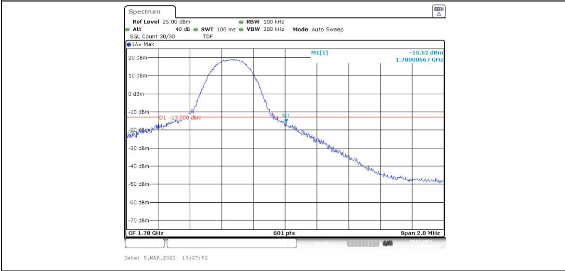
Band66-5MHz-16QAM-132647-25RB#0
