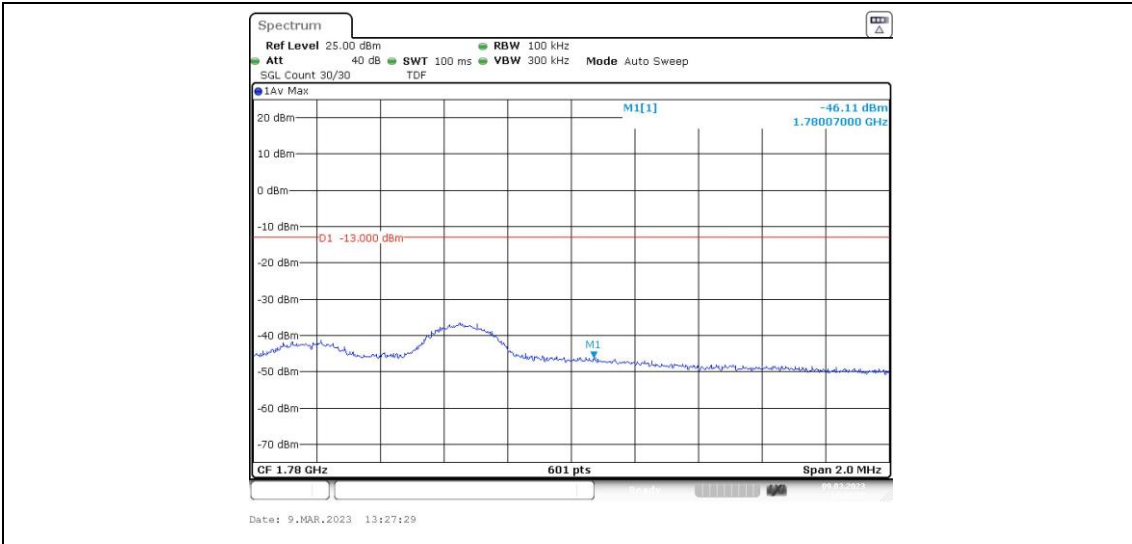
Band66-5MHz-16QAM-132647-1RB#24
