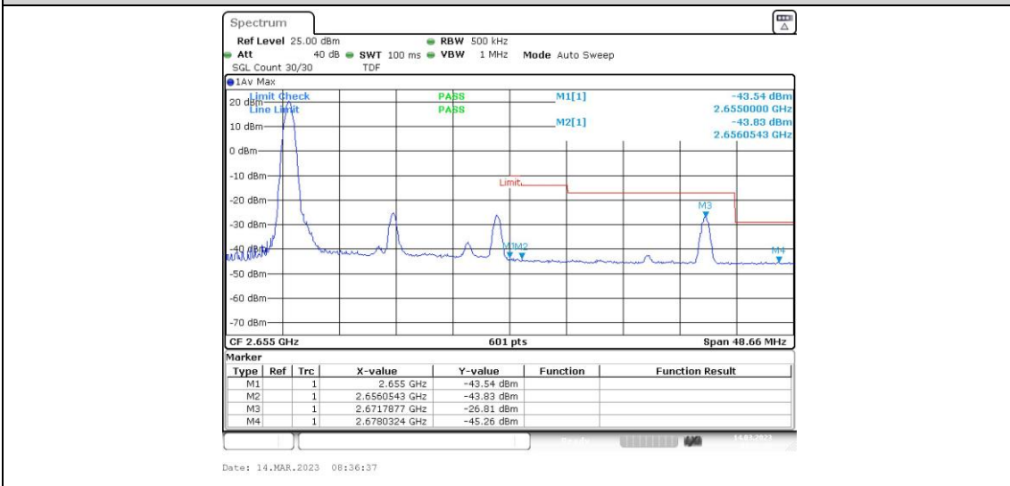
Band41-20MHz-16QAM-41140-1RB#99
