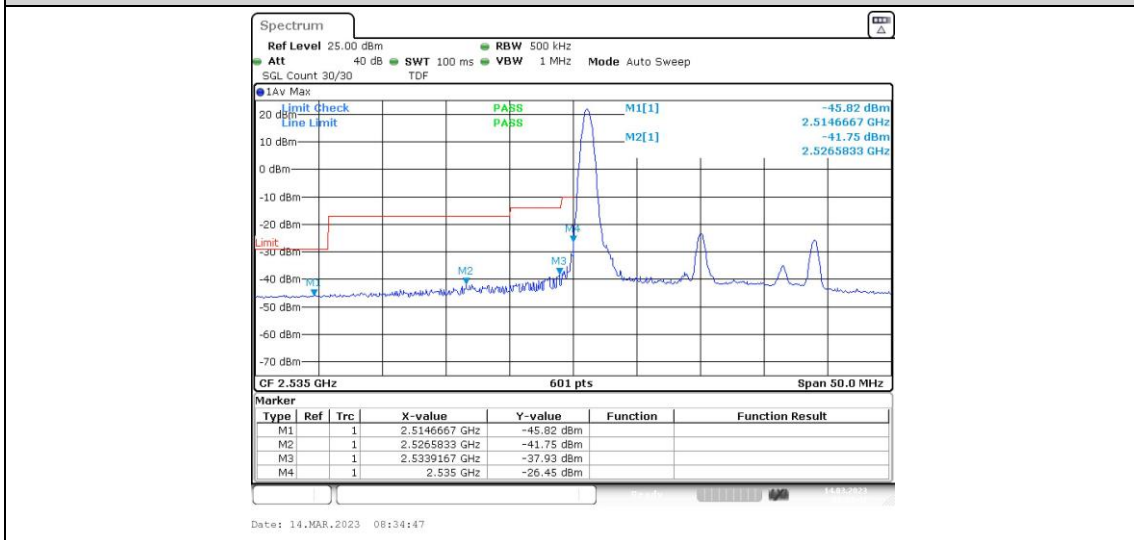
Band41-20MHz-QPSK-40140-1RB#99
