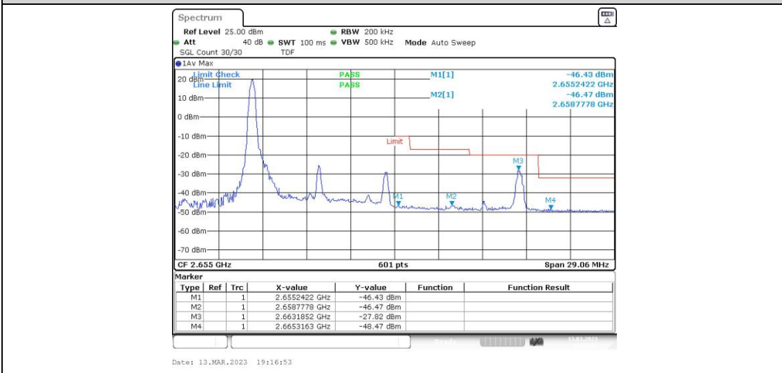
Band41-10MHz-16QAM-41190-1RB#49
