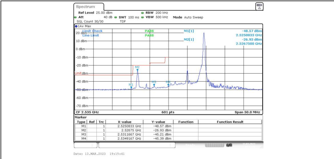
Band41-10MHz-16QAM-40090-50RB#0
