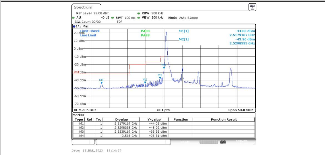
Band41-10MHz-QPSK-40090-1RB#49
