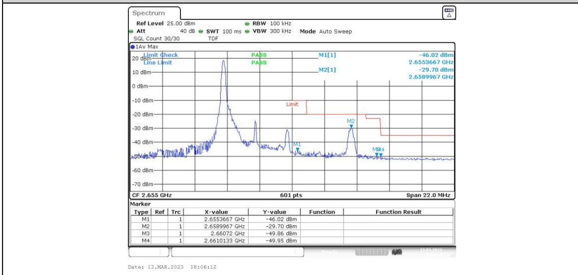
Band41-5MHz-16QAM-41215-1RB#24
