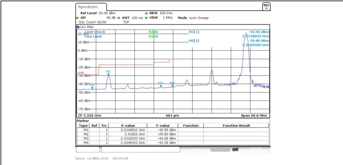
Band41-20MHz-16QAM-40140-100RB#0
