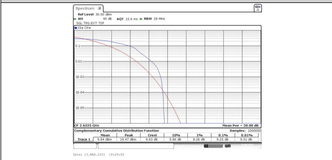
Band41-5MHz-QPSK-41215-25RB#0
