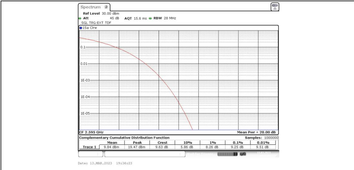
Band41-10MHz-16QAM-40640-50RB#0
