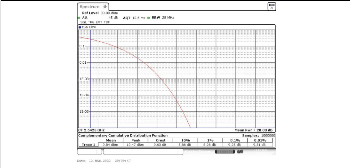
Band41-15MHz-QPSK-40115-75RB#0
