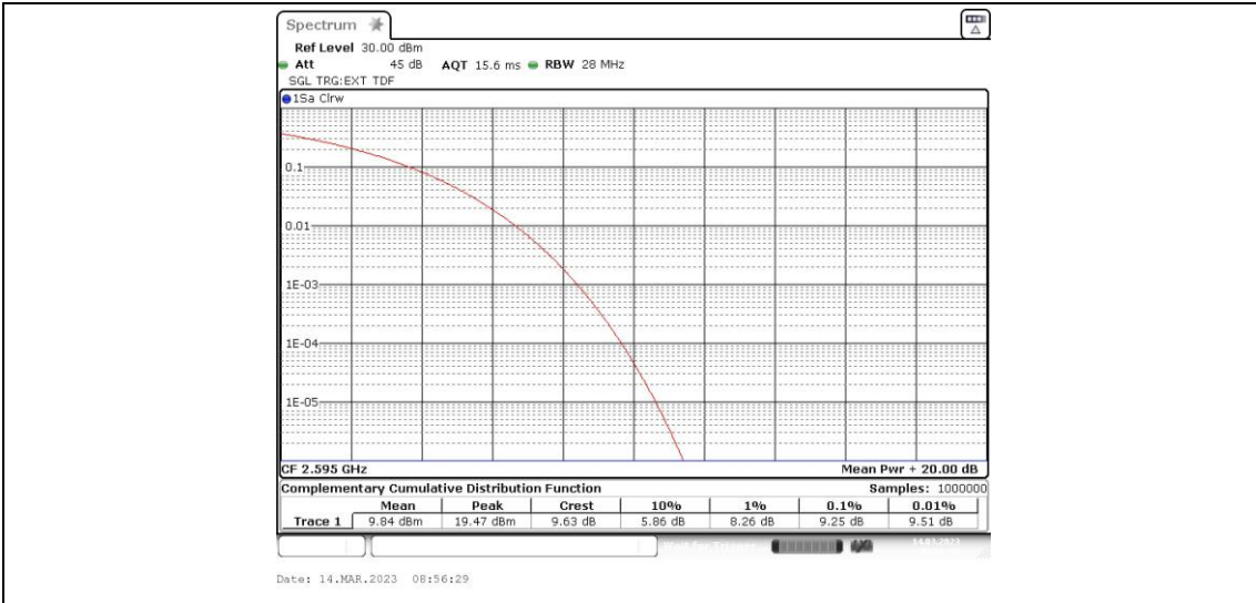
Band41-20MHz-16QAM-40640-100RB#0
