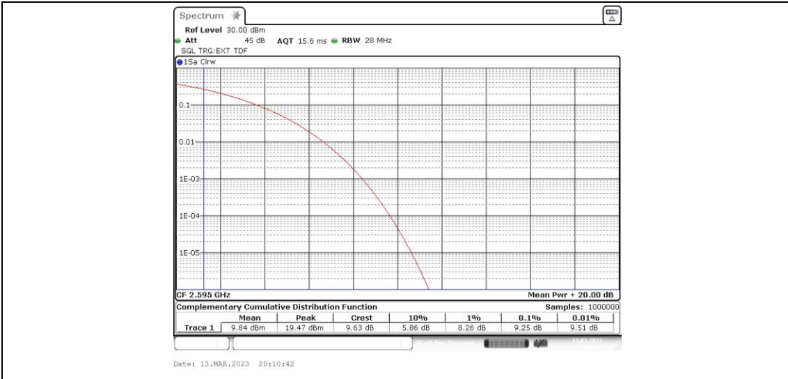
Band41-15MHz-QPSK-40640-75RB#0
