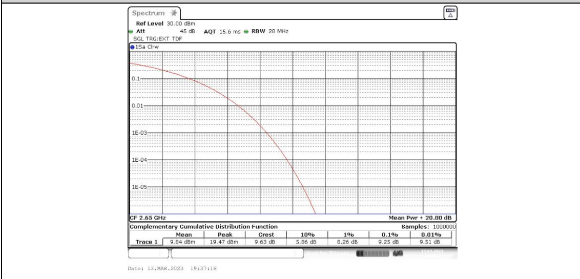
Band41-10MHz-16QAM-41190-50RB#0
