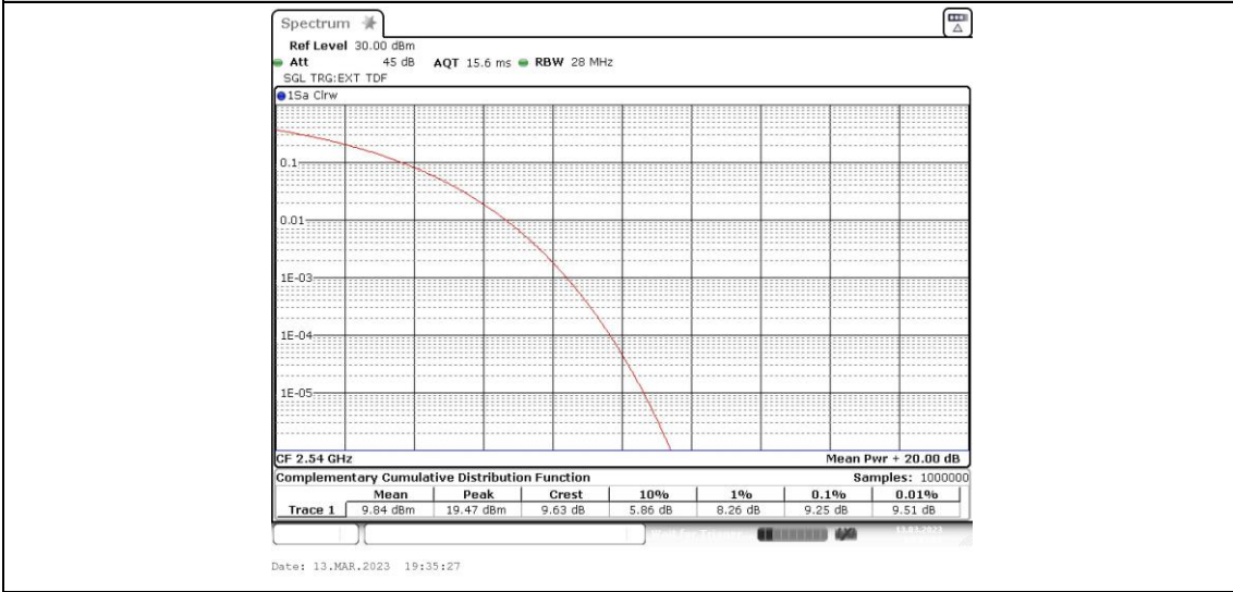
Band41-10MHz-16QAM-40090-50RB#0
