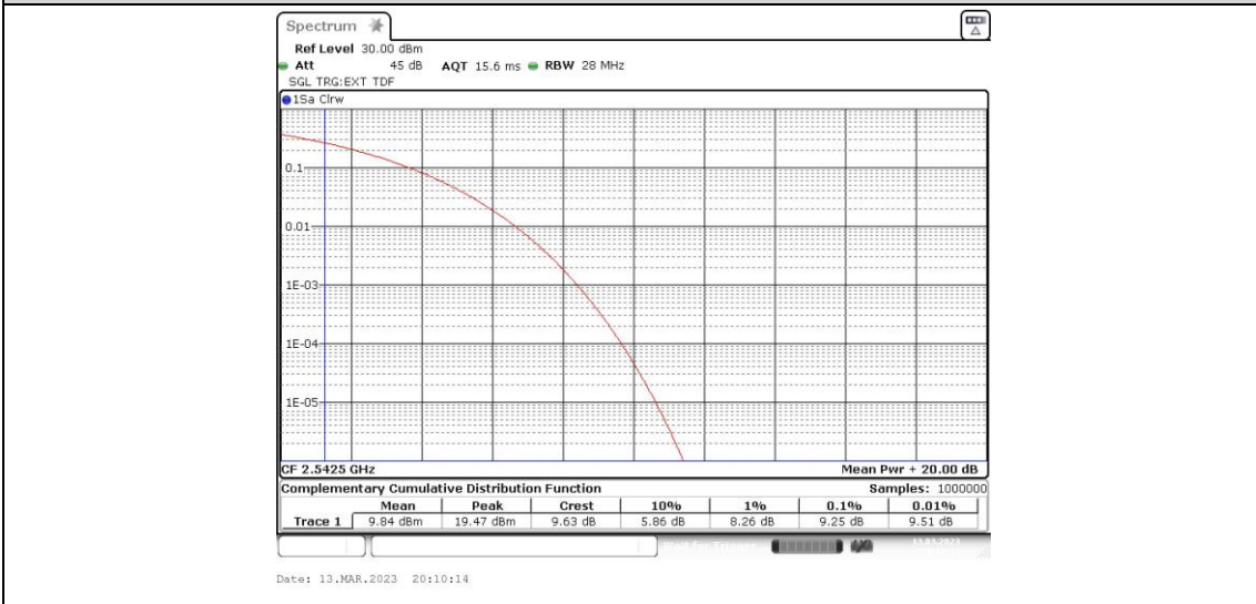
Band41-15MHz-QPSK-40640-1RB#0
