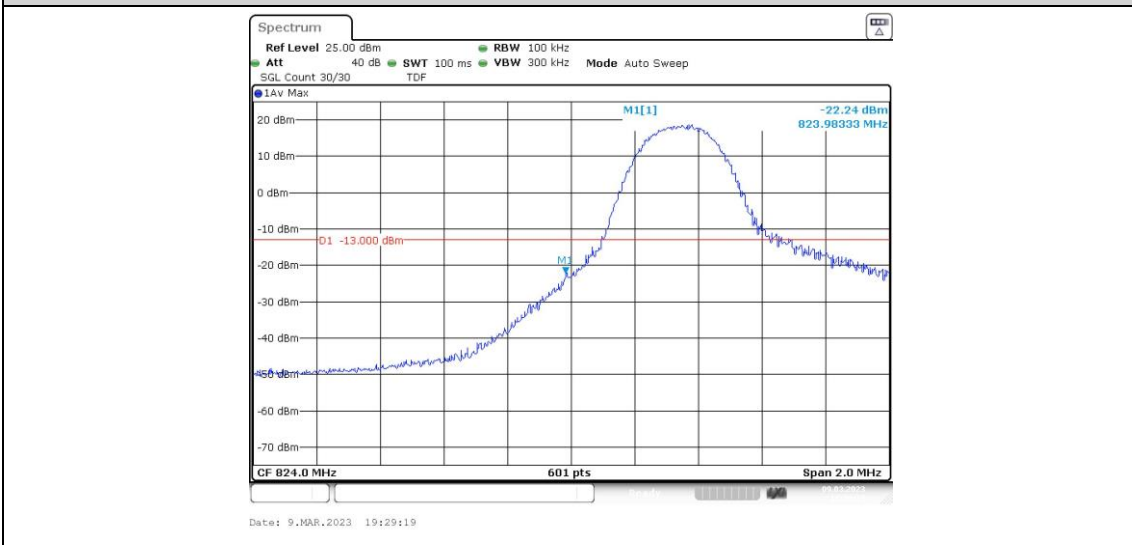
Band26-5MHz-16QAM-26815-1RB#24
