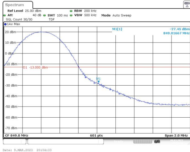
Band26-10MHz-QPSK-26990-50RB#0
