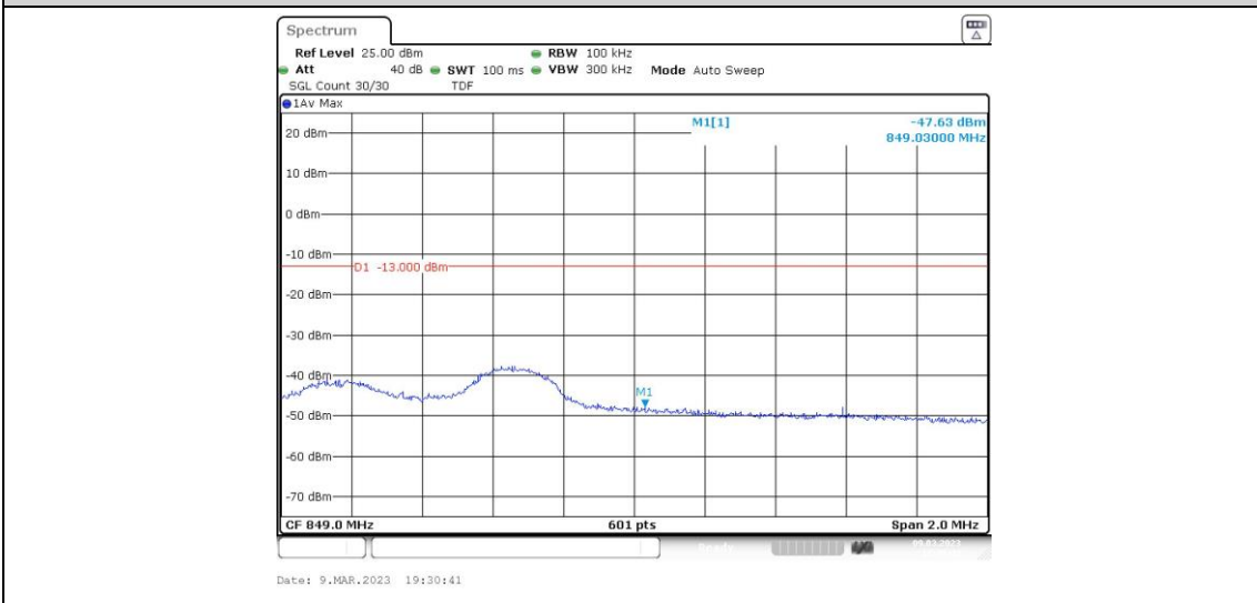
Band26-5MHz-16QAM-27015-1RB#24
