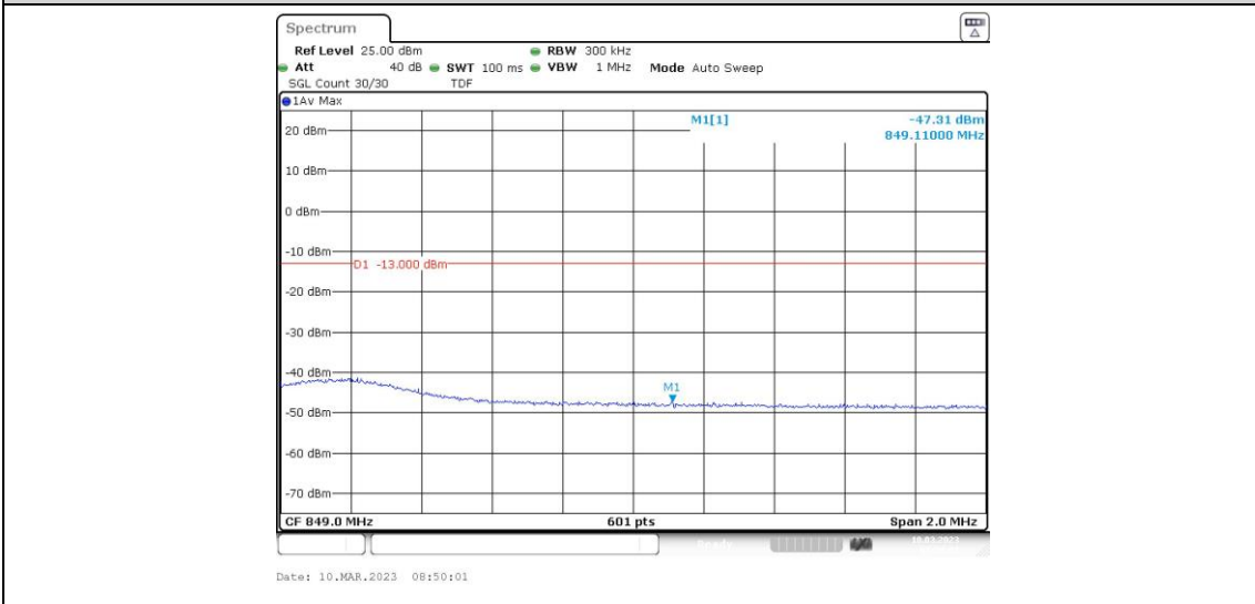
Band26-15MHz-16QAM-26965-1RB#74
