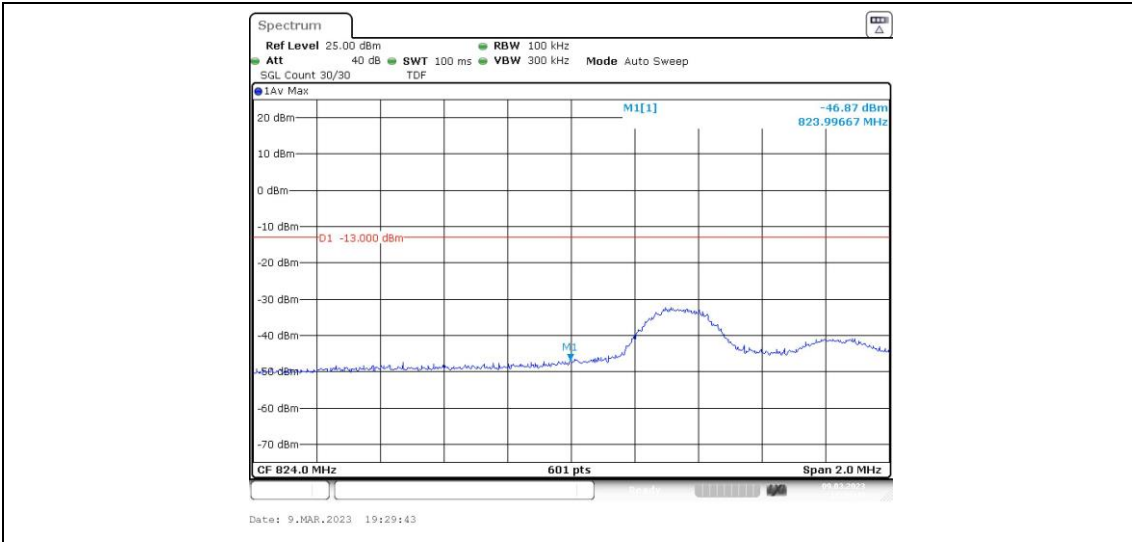
Band26-5MHz-16QAM-26815-25RB#0
