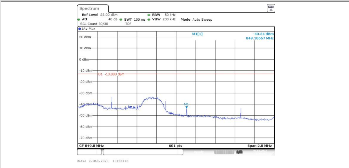
Band26-3MHz-QPSK-27025-1RB#14
