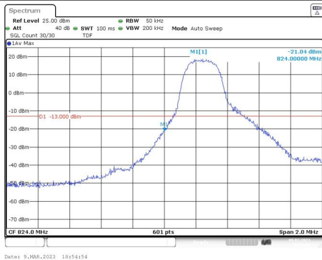
Band26-3MHz-QPSK-26805-1RB#14
