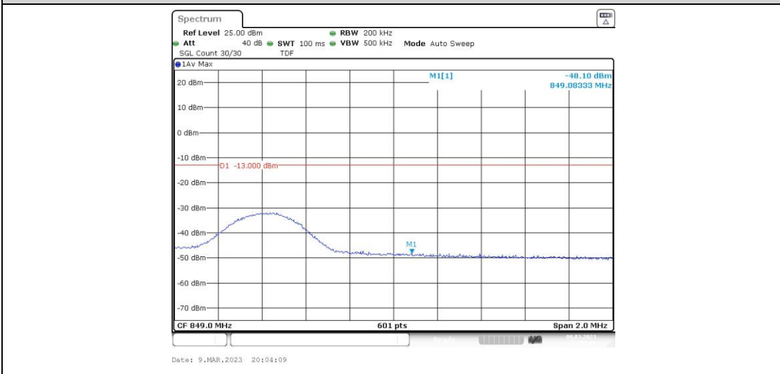
Band26-10MHz-QPSK-26990-1RB#49
