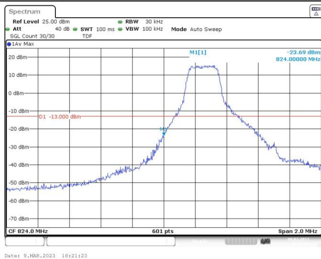
Band26-1.4MHz-16QAM-26797-1RB#5
