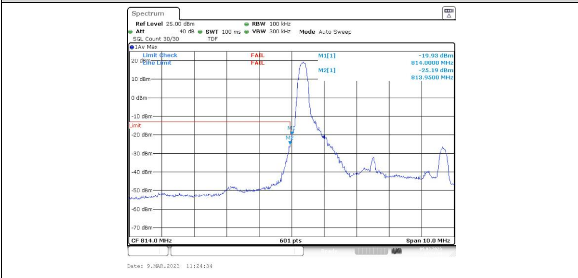
Band26-5MHz-16QAM-26715-1RB#24
