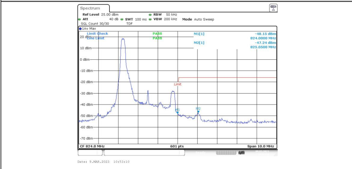
Band26-3MHz-QPSK-26775-1RB#14
