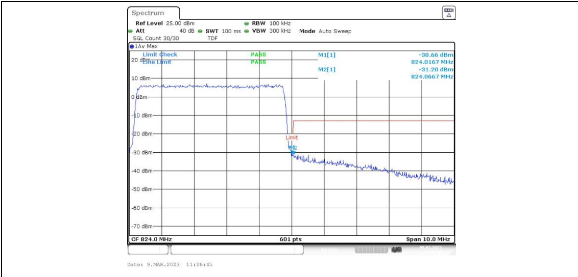
Band26-5MHz-16QAM-26715-1RB#0
