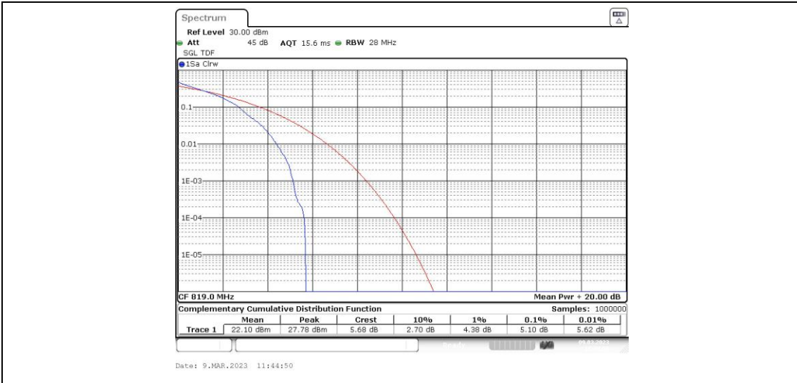
Band26-5MHz-QPSK-26740-25RB#0
