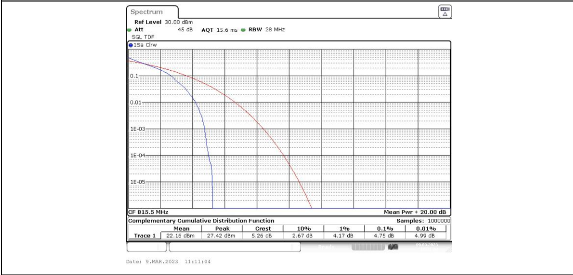
Band26-3MHz-QPSK-26705-15RB#0
