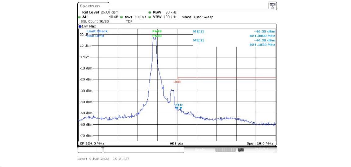
Band26-1.4MHz-QPSK-26783-1RB#5
