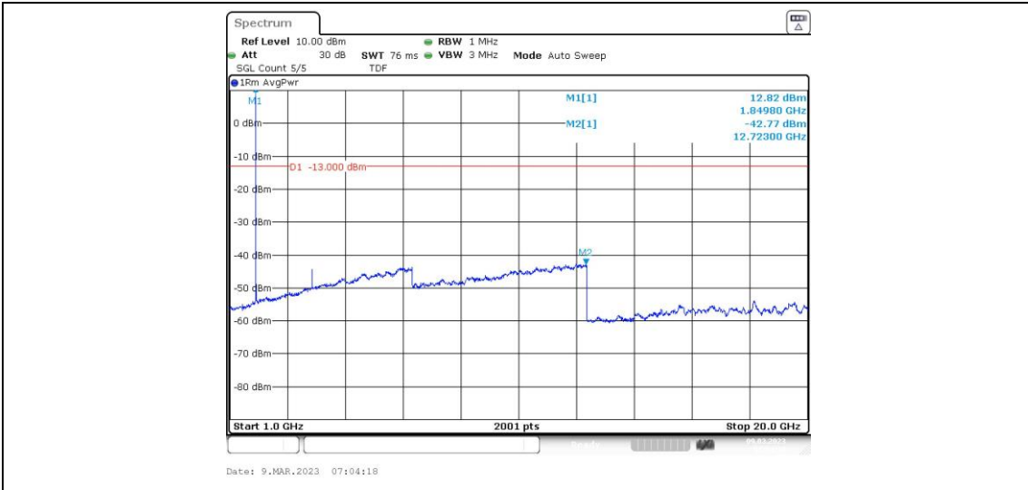
Band25-1.4MHz-16QAM-26365-1RB#0-Range1:0.009~0.15MHz
