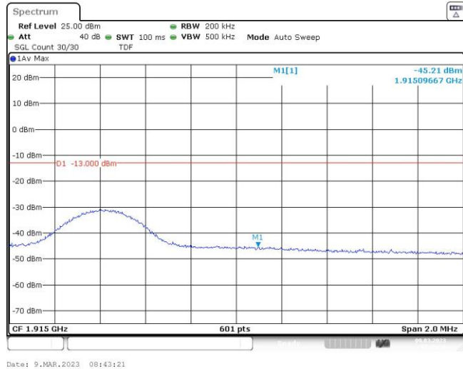
Band25-10MHz-16QAM-26640-1RB#49
