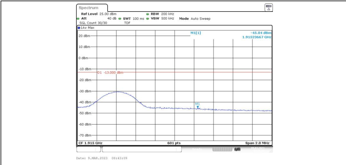
Band25-10MHz-QPSK-26640-1RB#49
