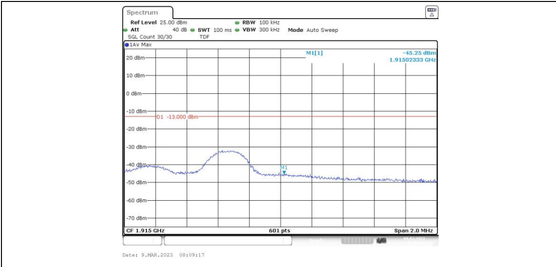
Band25-5MHz-QPSK-26665-1RB#24
