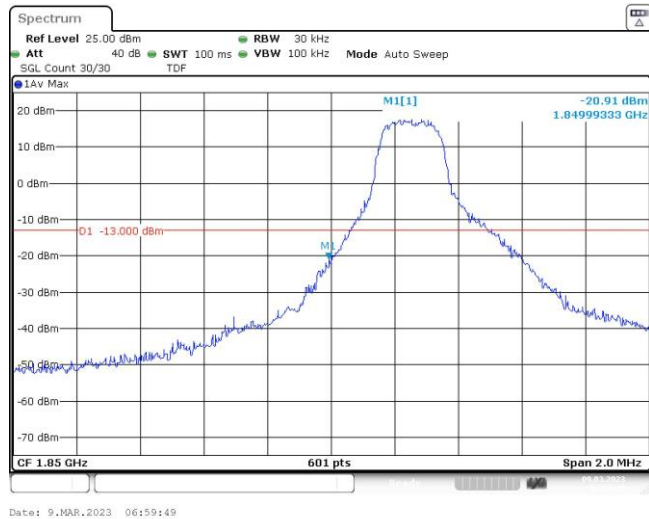
Band25-1.4MHz-QPSK-26047-1RB#5
