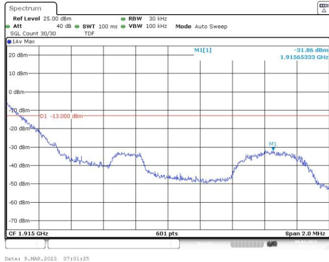
Band25-1.4MHz-16QAM-26683-1RB#5
