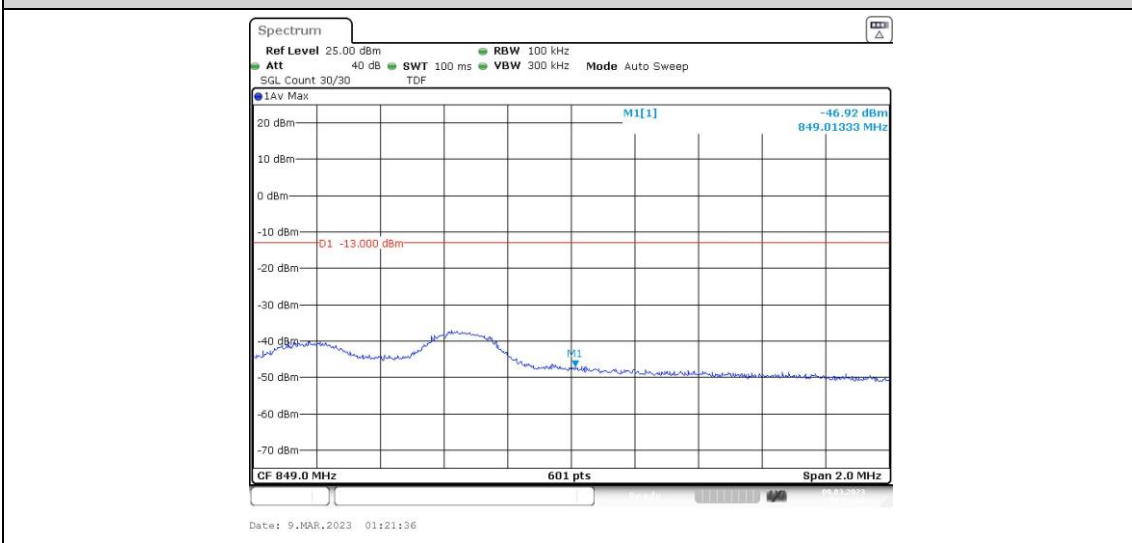
Band5-5MHz-16QAM-20625-1RB#24
