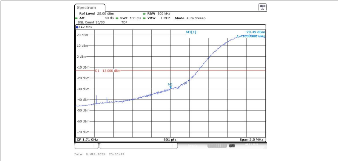
Band4-15MHz-16QAM-20025-1RB#74
