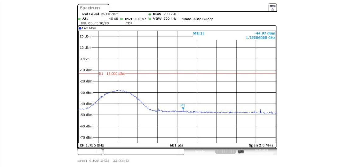
Band4-10MHz-16QAM-20350-1RB#49
