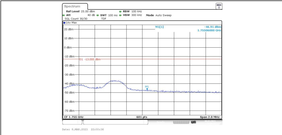
Band4-5MHz-16QAM-20375-1RB#24
