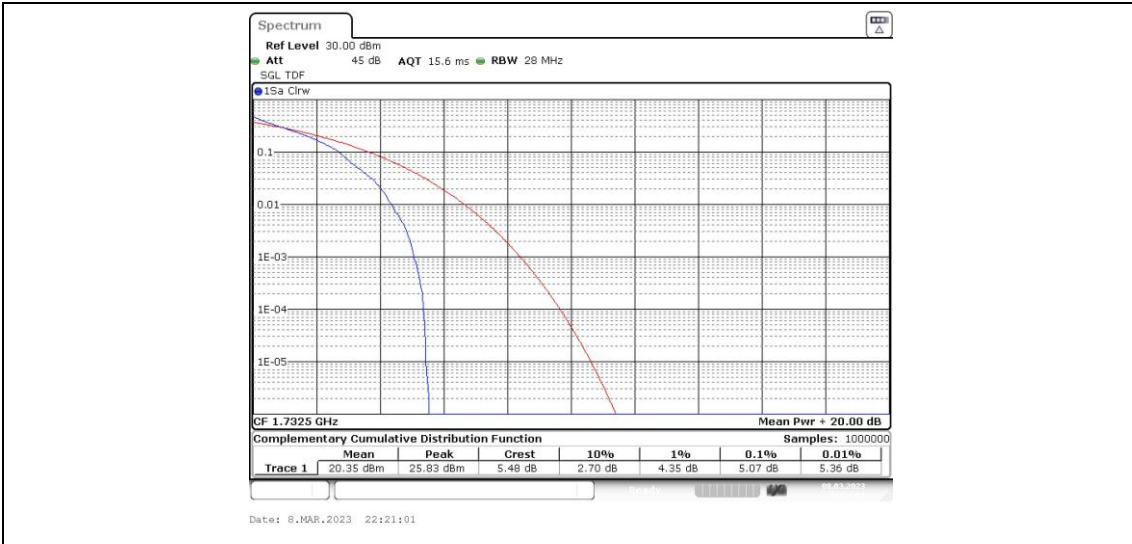
Band4-5MHz-QPSK-20175-25RB#0
