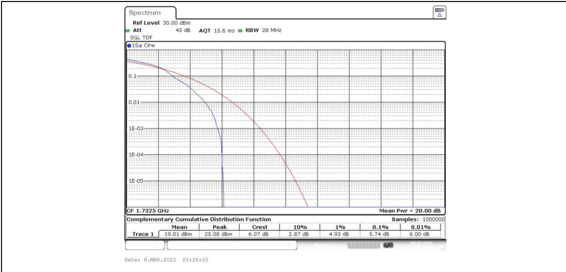
Band4-15MHz-16QAM-20175-75RB#0
