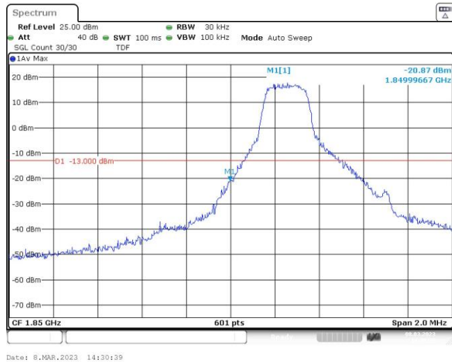
Band2-1.4MHz-QPSK-18607-1RB#5
