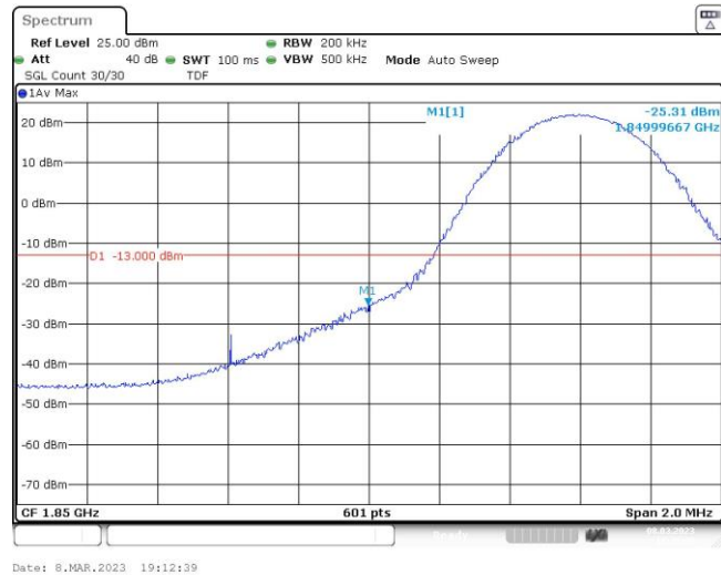
Band2-10MHz-QPSK-18650-1RB#49
