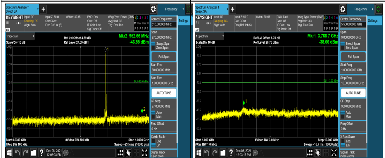
Band71-5MHz-QPSK-133297-1RB#0-Range1:30~1000MHz
