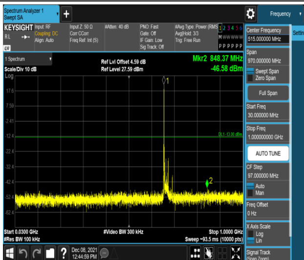
Band71-20MHz-16QAM-133222-1RB#0-Range1:30~1000MHz
