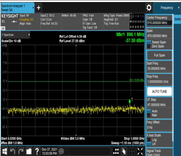
Band25-20MHz-16QAM-26365-1RB#0-Range1:30~1000MHz
