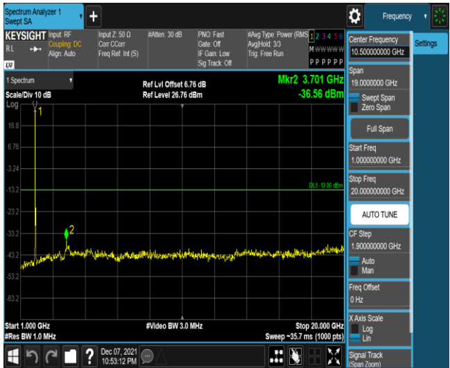
Band25-20MHz-16QAM-26140-1RB#0-Range2:1000~20000MHz
