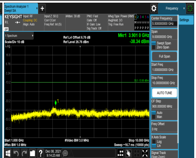
Band26-10MHz-16QAM-26740-1RB#0-Range2:1000 ~10000MHz
